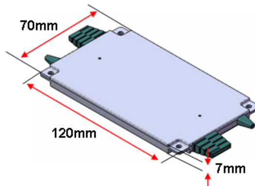
Same package size as 100 GHz MSA (120x70x7 mm)
