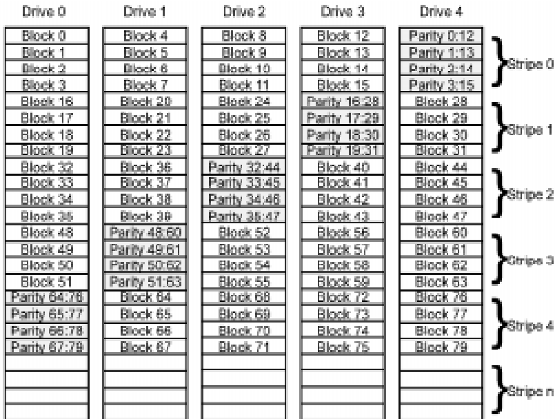
Figure 2-10. Block Striping with Parity
