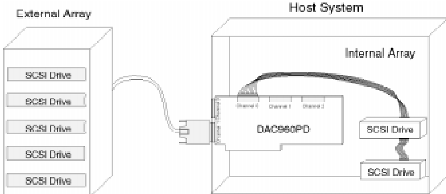
Figure 2-1. System Diagram
