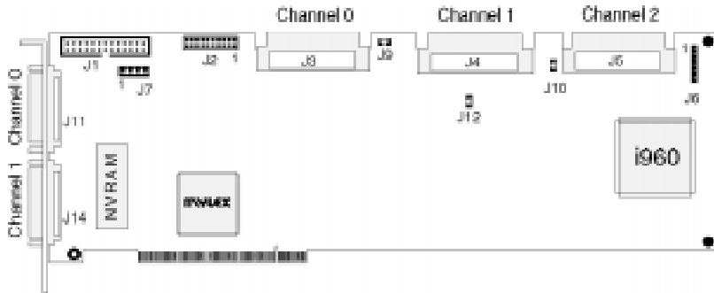
Figure 3-1. DAC960P/PD/PD-Ultra Series Component Locator
