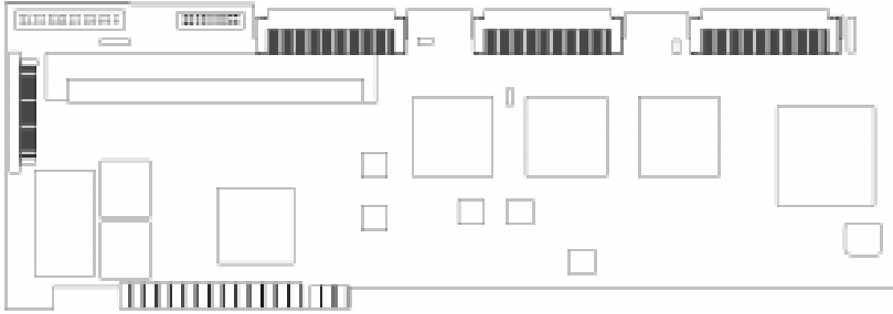
Figure 1-2. DAC960 Controller component layout
