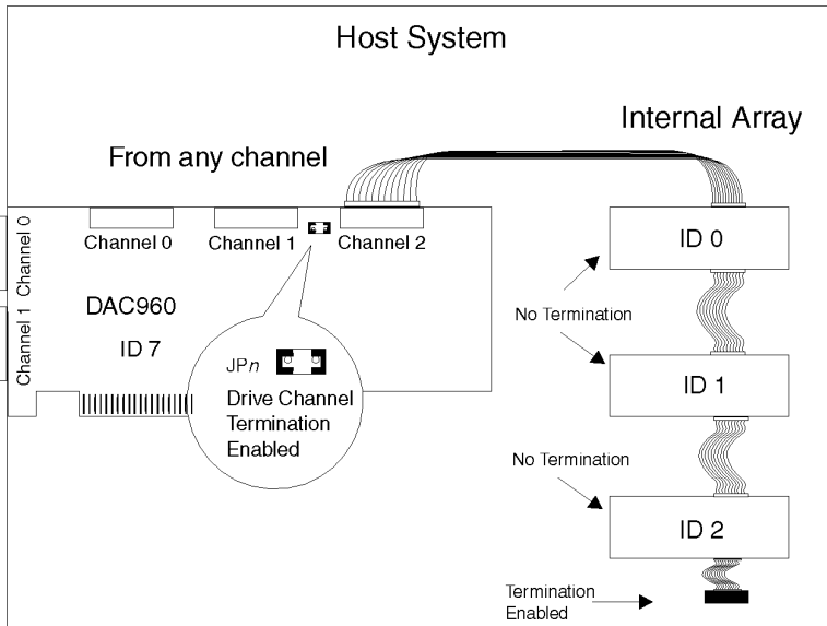
Figure 3-4. Internal Disk Array, Single-ended SCSI Termination
