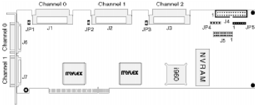
Figure 3-2. DAC960PL Component Locator
