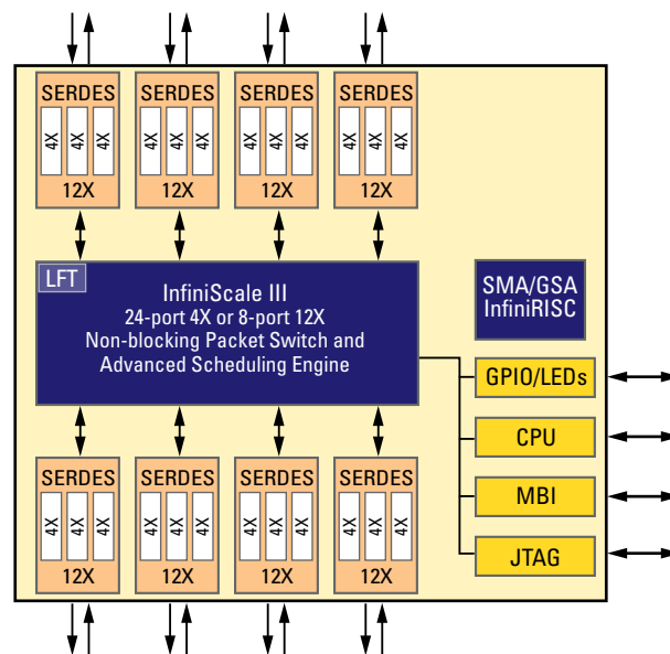
InfiniScale III Block Diagram
