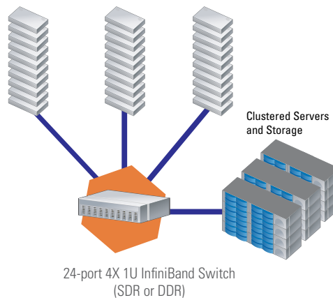
InfiniScale III based InfiniBand Switch Products from Mellanox as Production Development Kits (PDK)
