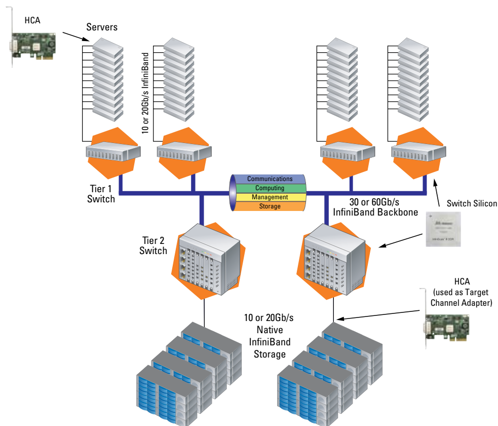
InfiniHost III Lx HCA Cards used in Compute and Storage Nodes for a Unified InfiniBand Network
