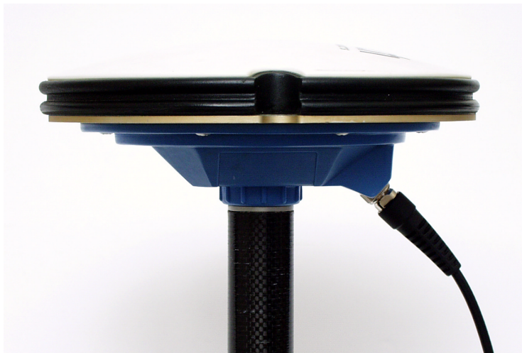
Figure 4.6 Geodetic IV GPS Antenna on Rover Pole
