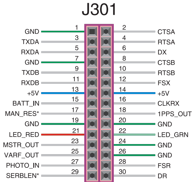
Figure 1.2. Pin Configuration of the J301 connector
