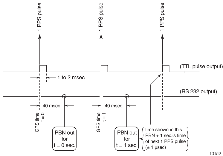
Figure 3.6. Relationship of GPS Time in PRN Record to Output of 1PPS Pulse
