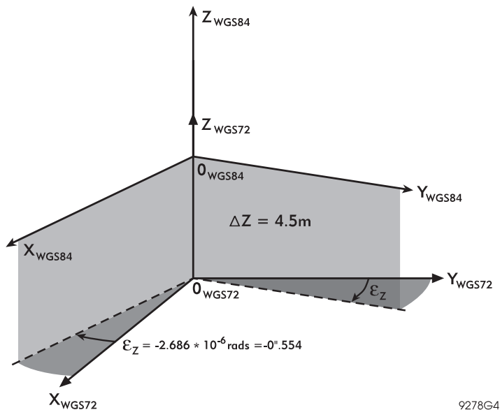
Figure 4.2. Rotation and Translation Between the WGS72 and WGS84 Coordinate Systems
