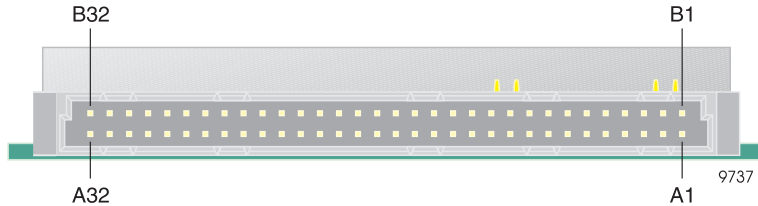
Figure 2.2: Z-Eurocard Interface Connector
