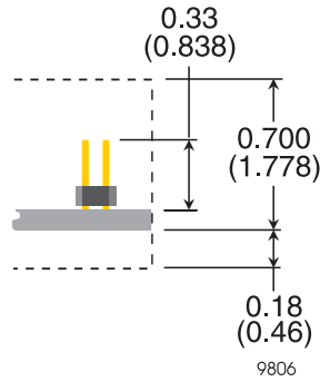
Figure 2.3: 64-Pin Straight Header Option
