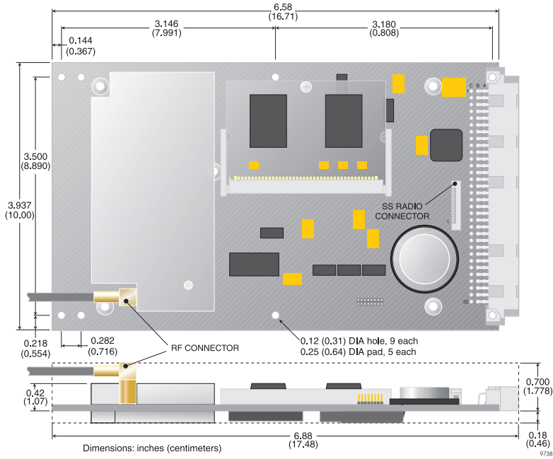
Figure 2.1: Z-Eurocard Dimensions
