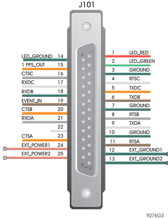
Figure 2.8: DB25 Connector
