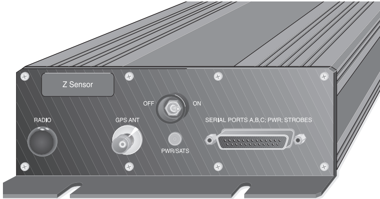
Figure 2.6: Z-Sensor Front Panel
