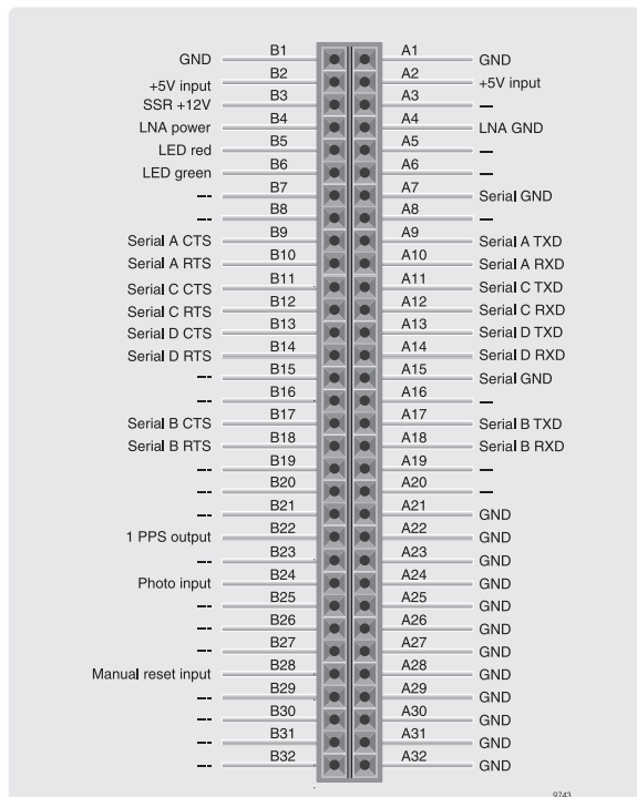
Figure 2.4: Interface Connector Pinouts
