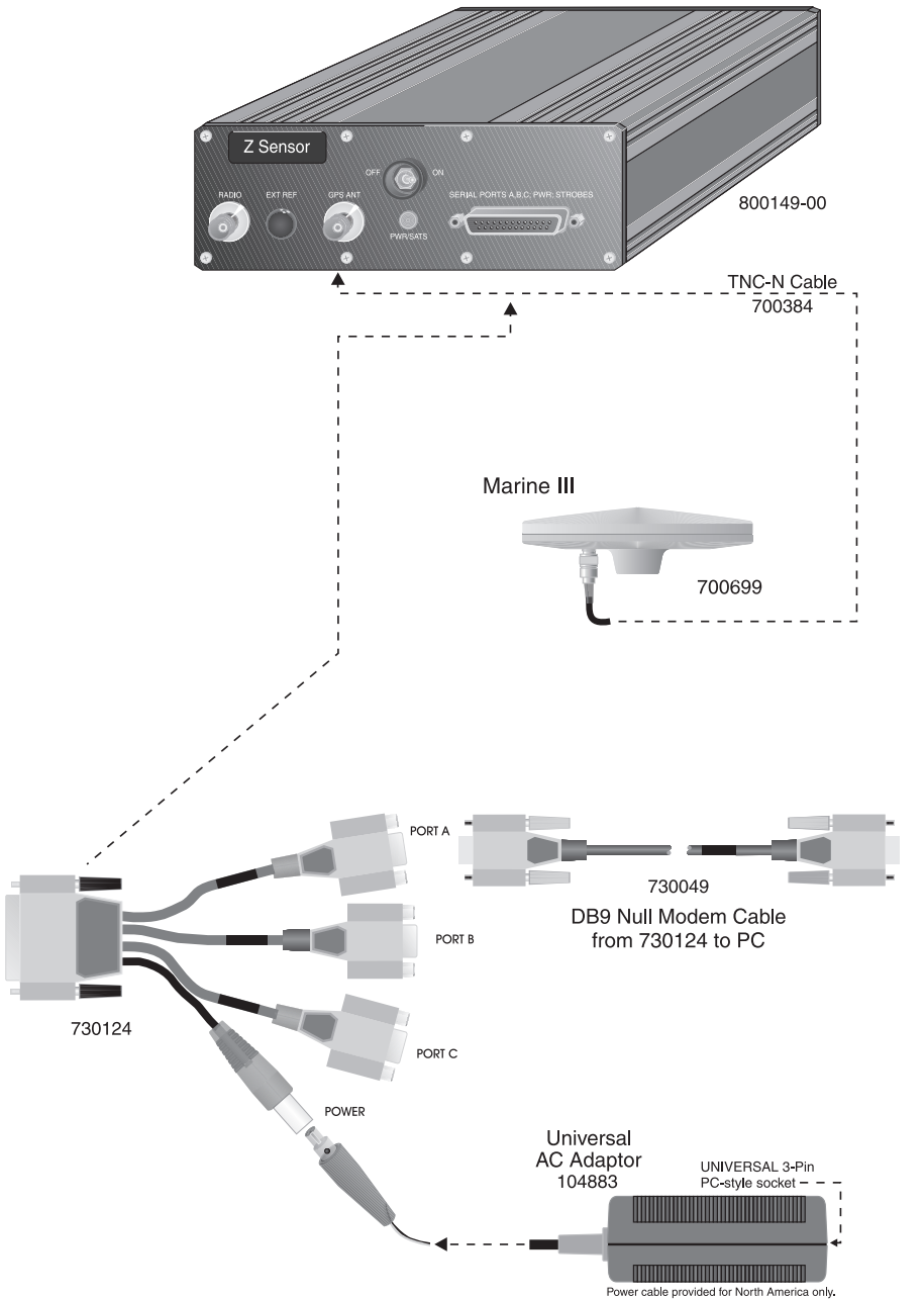
Figure 2.11: Z-Sensor Development Kit (B)
