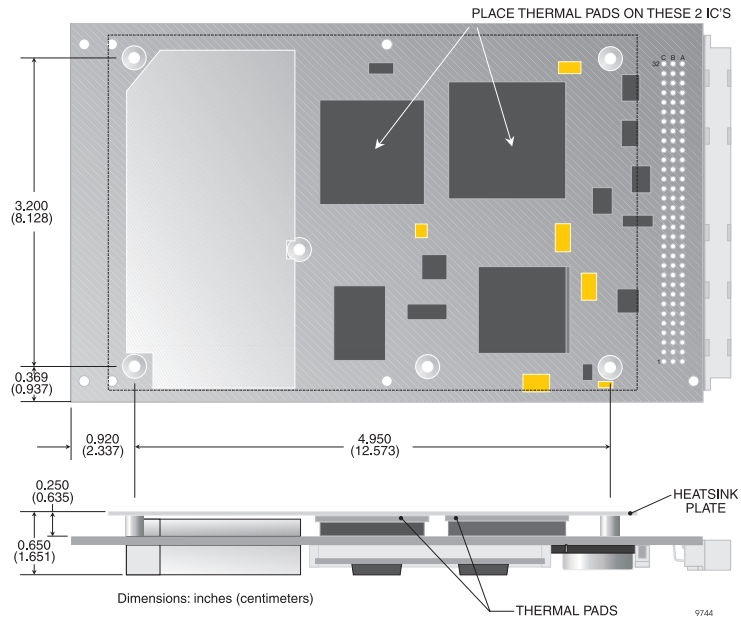
Figure 2.5: Z-Eurocard Mounted with Heat-Sink
