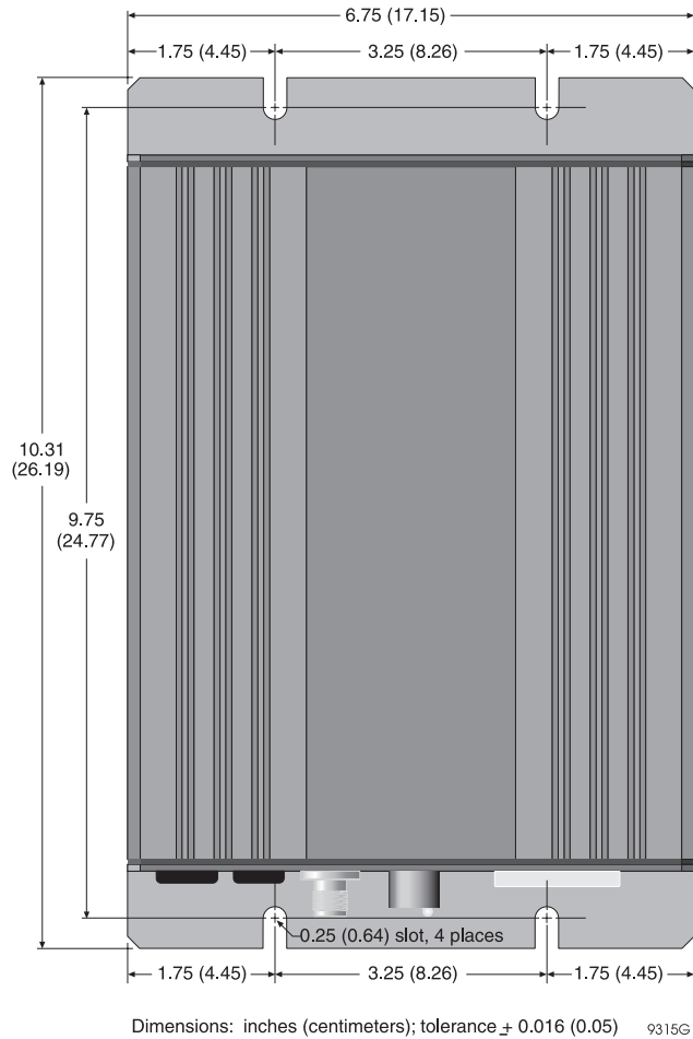
Figure 2.7: Z-Sensor Mounting Dimensions
