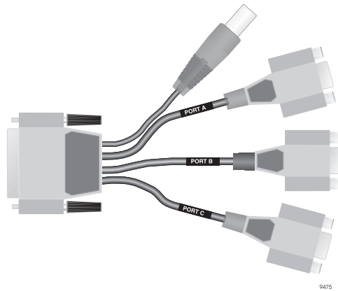
Figure 2.9: Z-Sensor Serial/Power Cable
