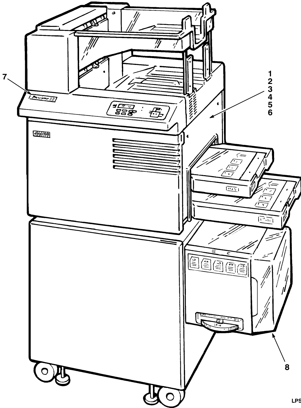
Figure 1. PrintServer 32 System
