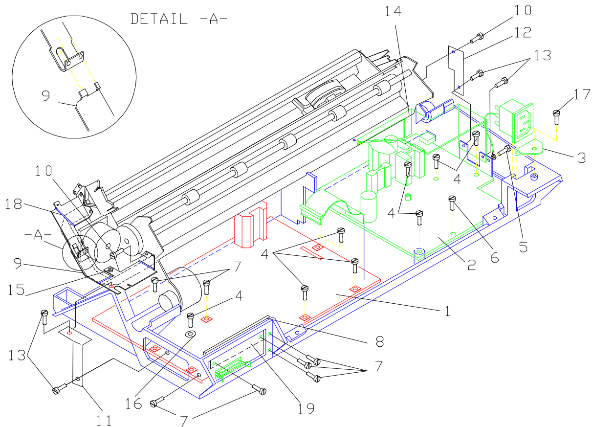
Figure 7 Boards Assembly
