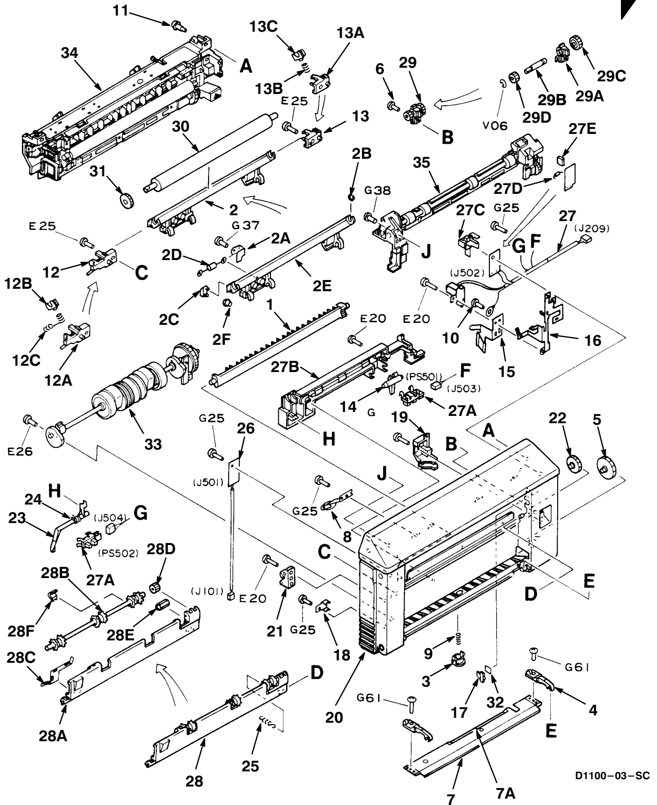
Figure 3. Cover Assembly, Front
