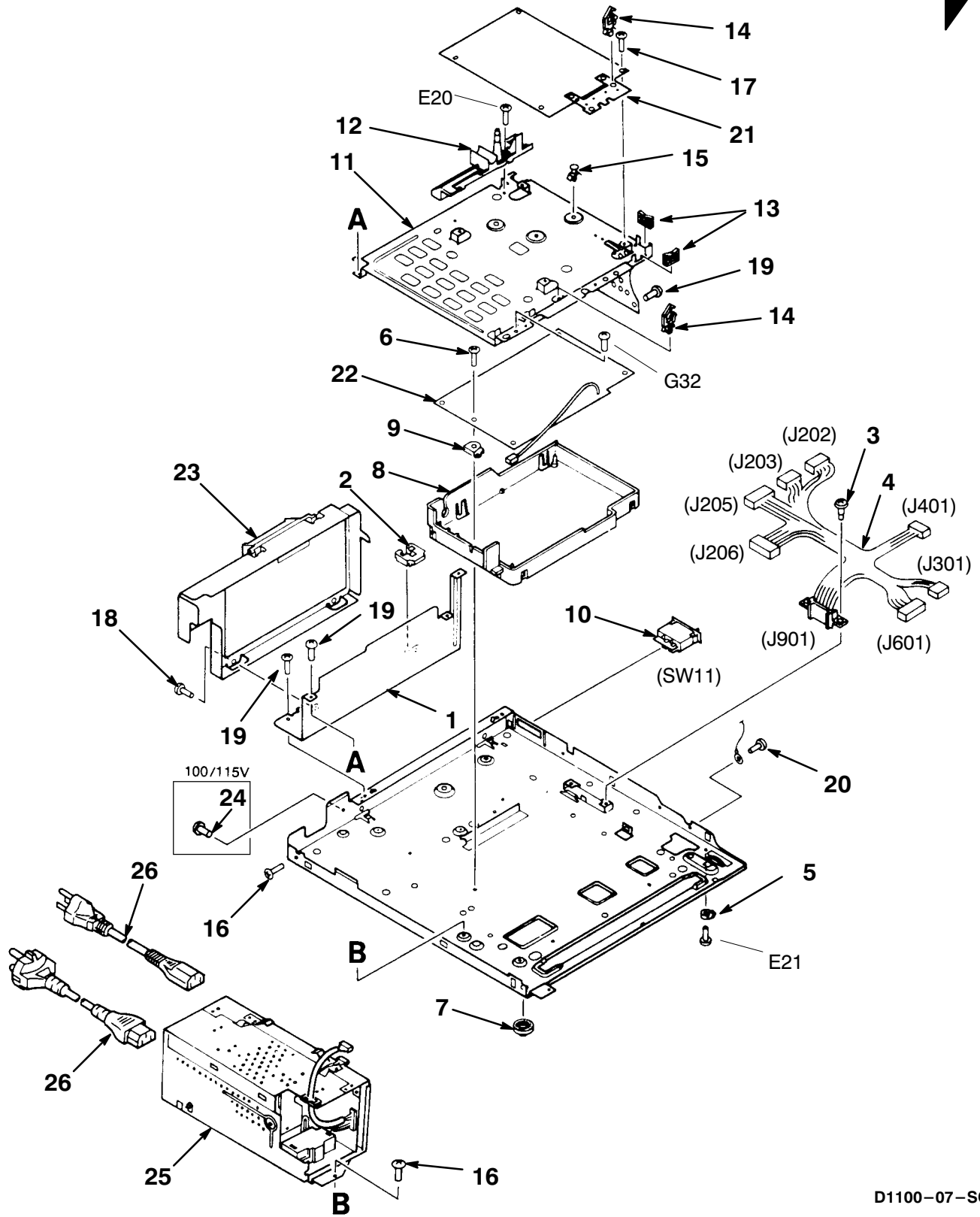
Figure 7. Plate Assembly, Machine Bottom
