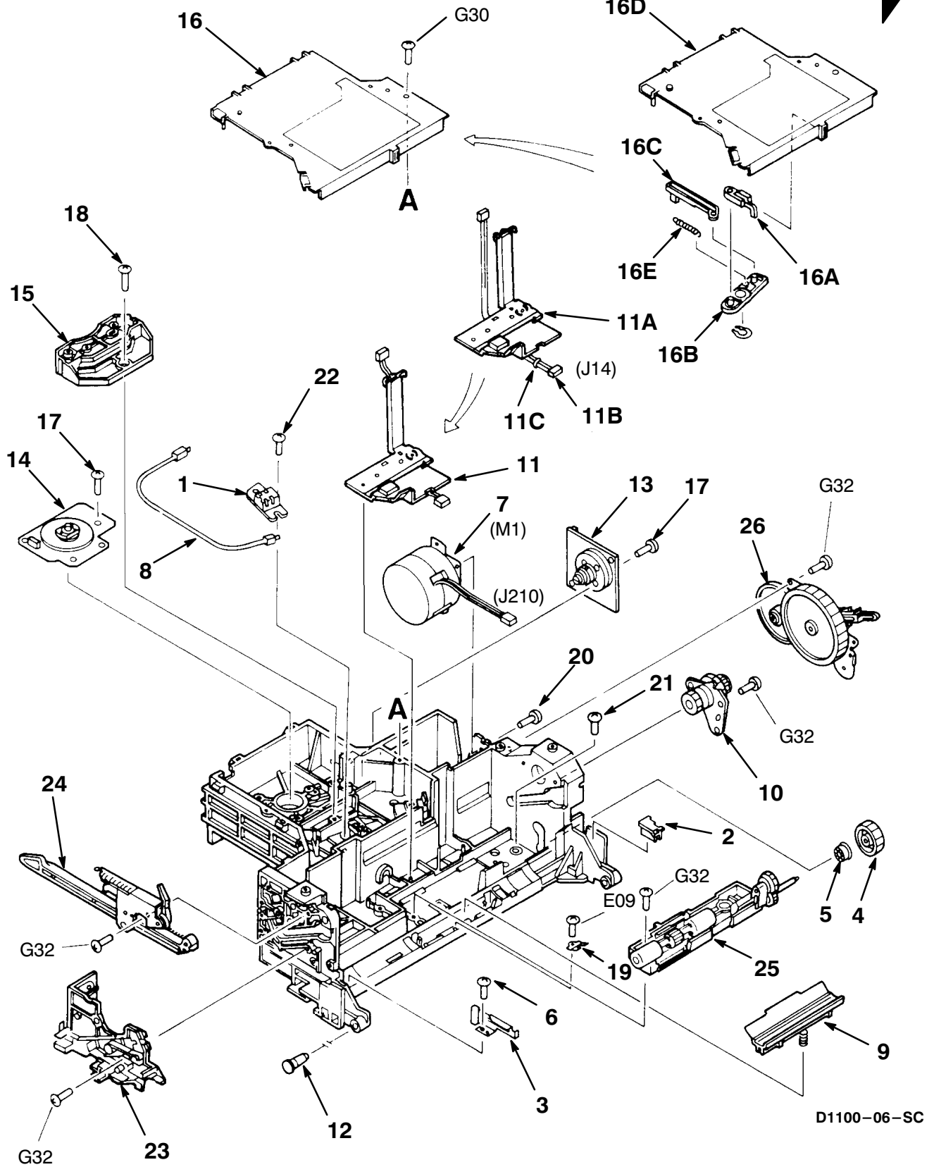
Figure 6. Components Assembly, Internal
