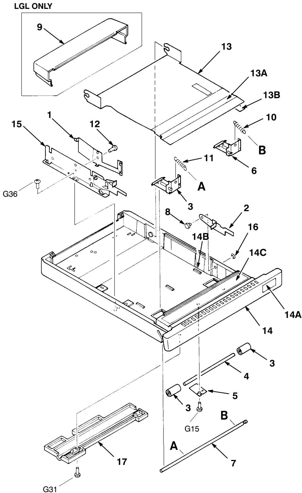
Figure 17. Cassette Assembly (A4, LGL)
