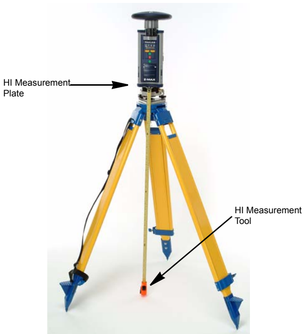
Figure 8 Measuring Instrument Height (HI)
