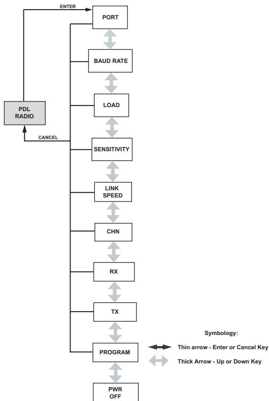
Figure 16 COM OPTN: PDL Radio Menu
