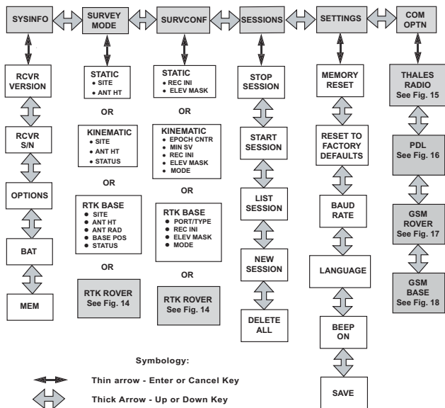
Figure 6 Display Main Menu
