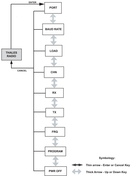
Figure 15 COM OPTN: THALES Radio Menu
