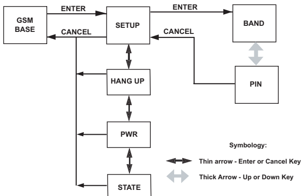
Figure 18 COM OPTN: GSM Base Menu
