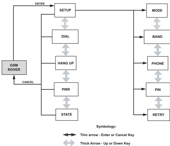
Figure 17 COM OPTN GSM Rover Menu
