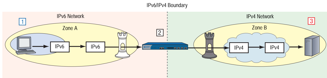
Figure 16: Network Address Translation (NAT) Across an IPv4/IPv6 Boundary
