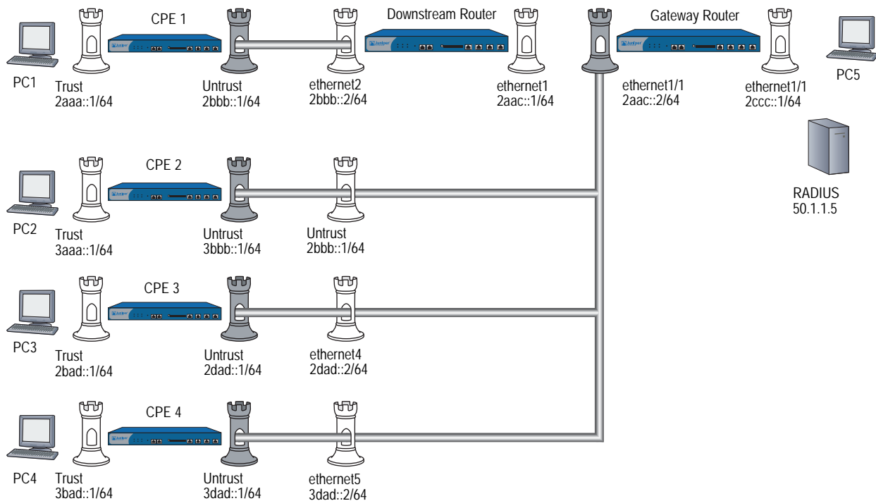
Figure 41: IPSec Access Session Example
