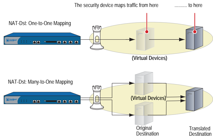
Figure 19: NAT-Dst—One-to-One and Many-to-One
