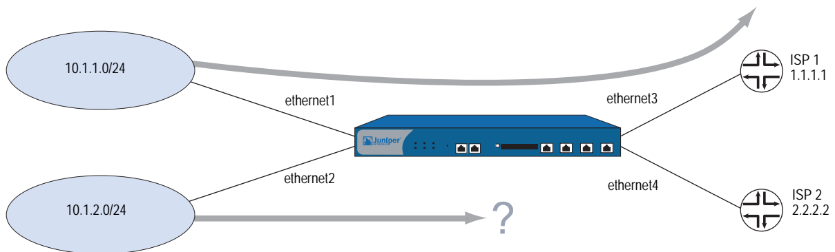
Figure 8: Route Lookup in Multiple VRs
