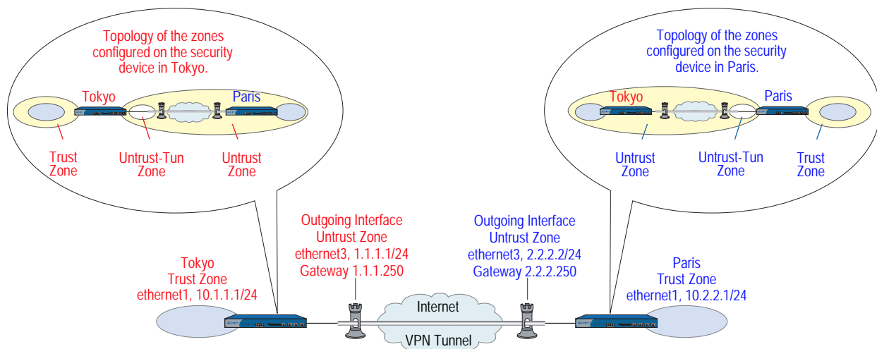
Figure 34: Policy-Based Site-to-Site VPN, Manual Key
