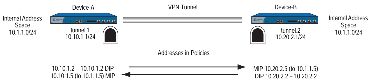
Figure 38: Overlapping Addresses at Peer Sites
