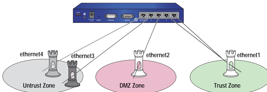
Figure 23: DMZ/Dual Untrust Port-Mode Interface to Zone Bindings
