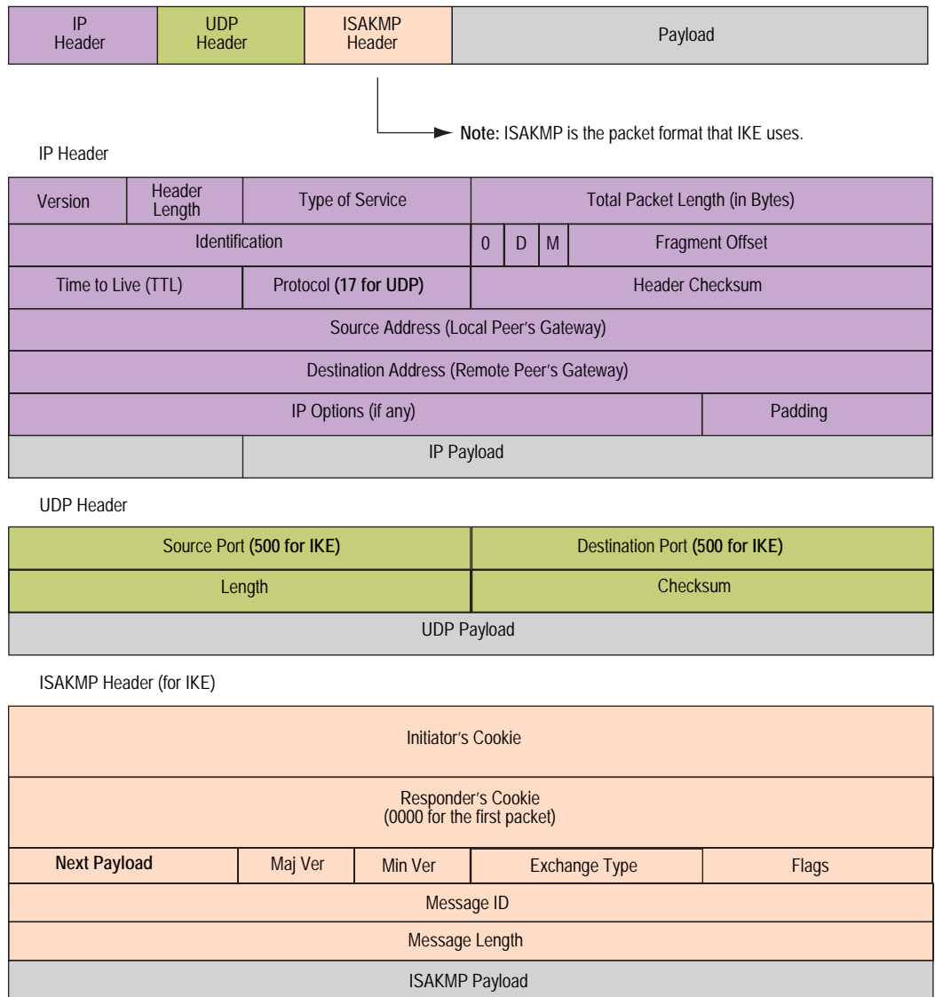
Figure 6: IKE Packet for Phases 1 and 2
