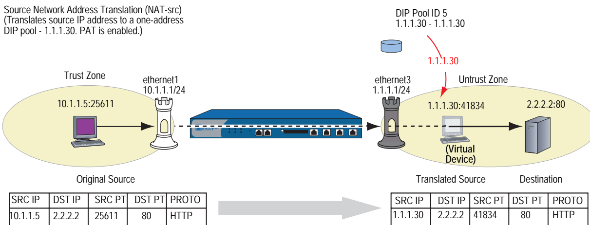
Figure 17: NAT-Src with PAT Enabled
