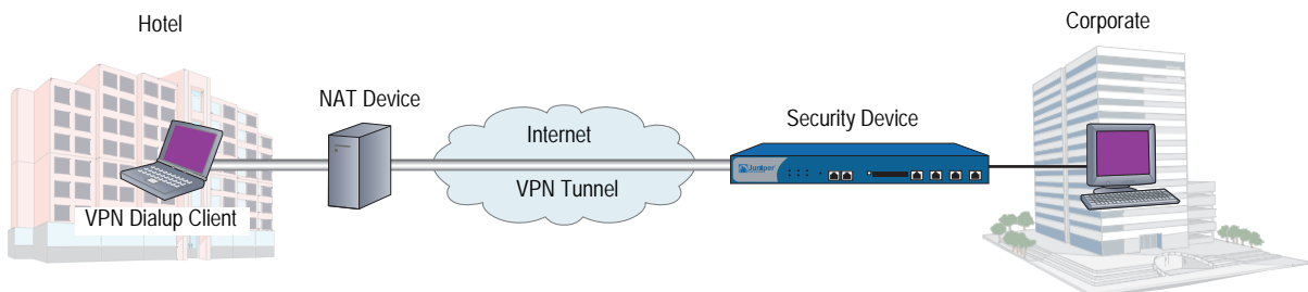
Figure 65: Enabling NAT-Traversal
