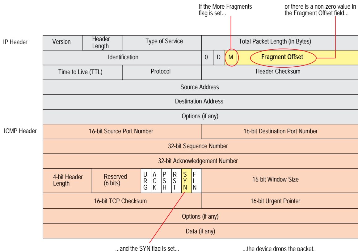
Figure 91: SYN Fragments
