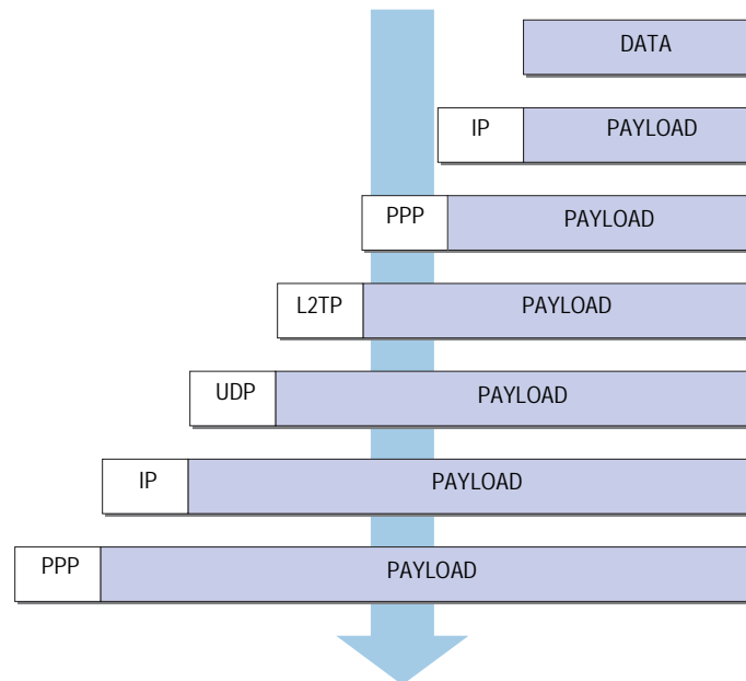
Figure 55: L2TP Packet Encapsulation
