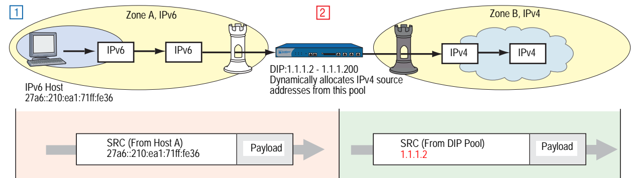
Figure 17: DIP from IPv6 to IPv4
