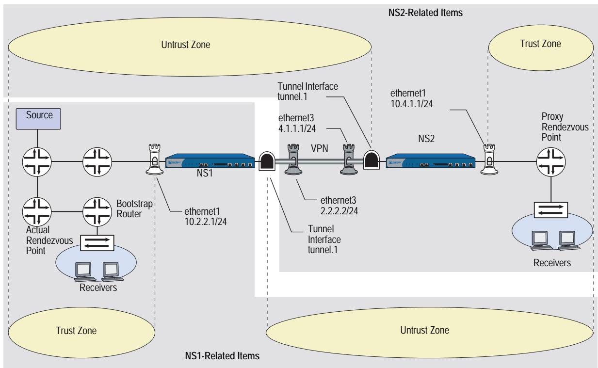
Figure 34: Proxy RP Configuration Example
