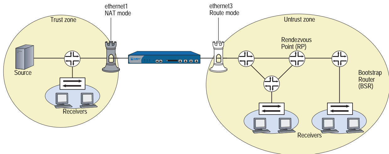
Figure 33: Proxy Rendezvous Point Example
