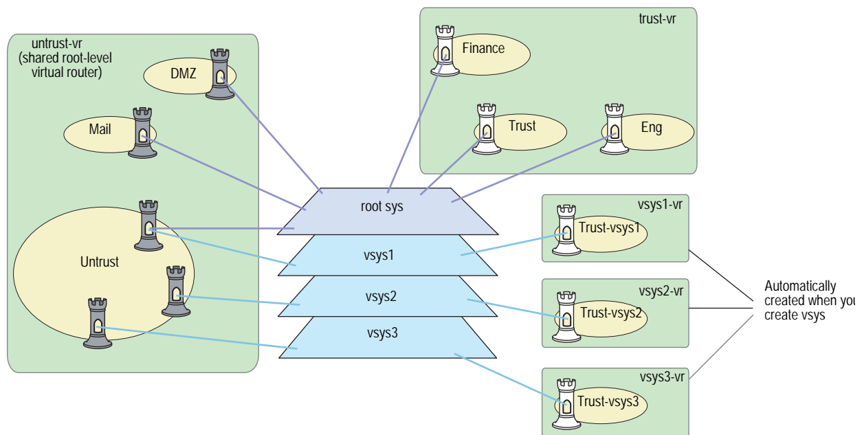
Figure 6: Virtual Routers Within a Vsys
