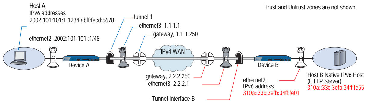
Figure 29: 6over6 Manual Tunneling
