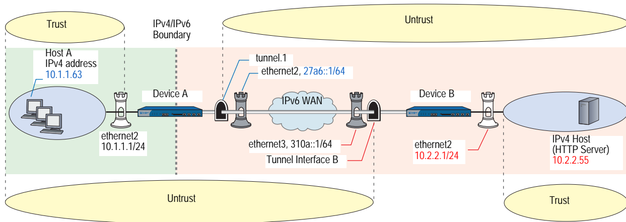
Figure 32: IPSec 4in6 Tunnel Example
