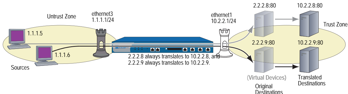
Figure 13: NAT-Dst Between Address Ranges
