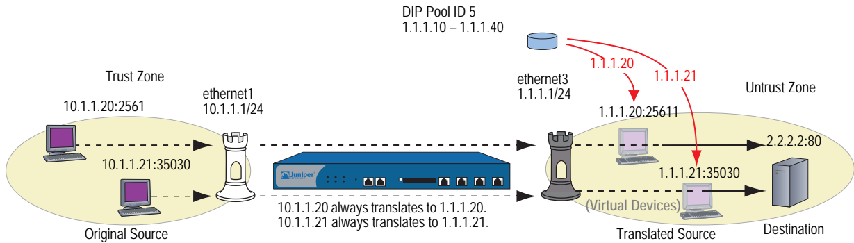
Figure 8: NAT-Src with Address Shifting
