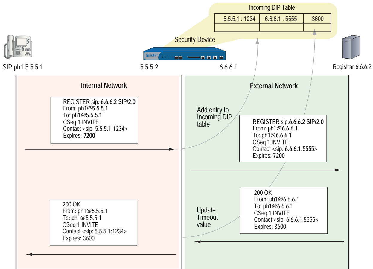
Figure 10: Incoming SIP
