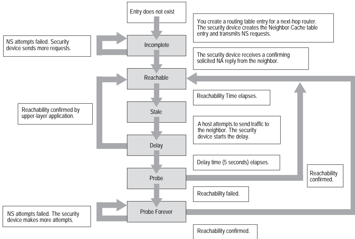
Figure 5: Next-Hop Gateway Router Reachability Transitions
