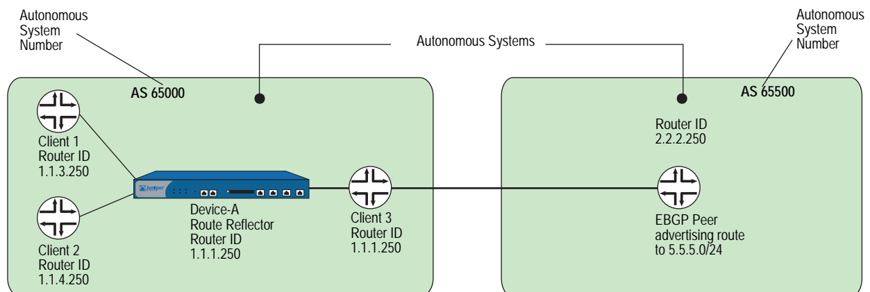
Figure 16: BGP Route Reflection Example
