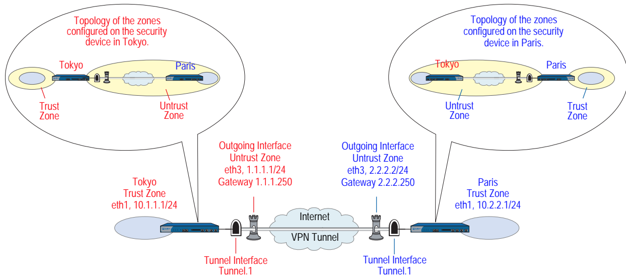
Figure 33: Route-Based Site-to-Site VPN, Manual Key
