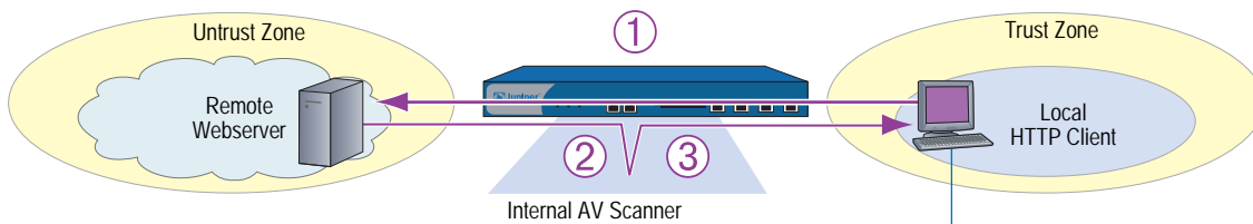
Figure 35: Antivirus Scanning for HTTP Webmail Traffic
