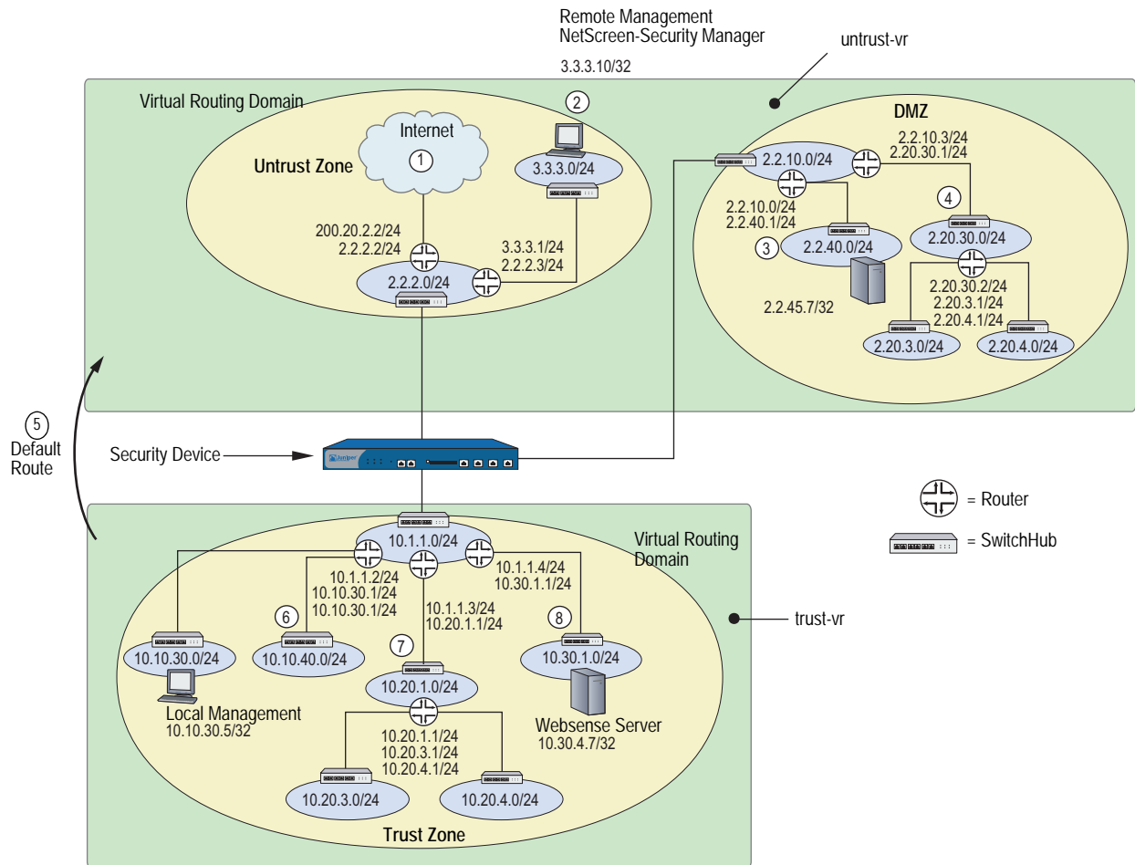
Figure 2: Static Route Configuration
