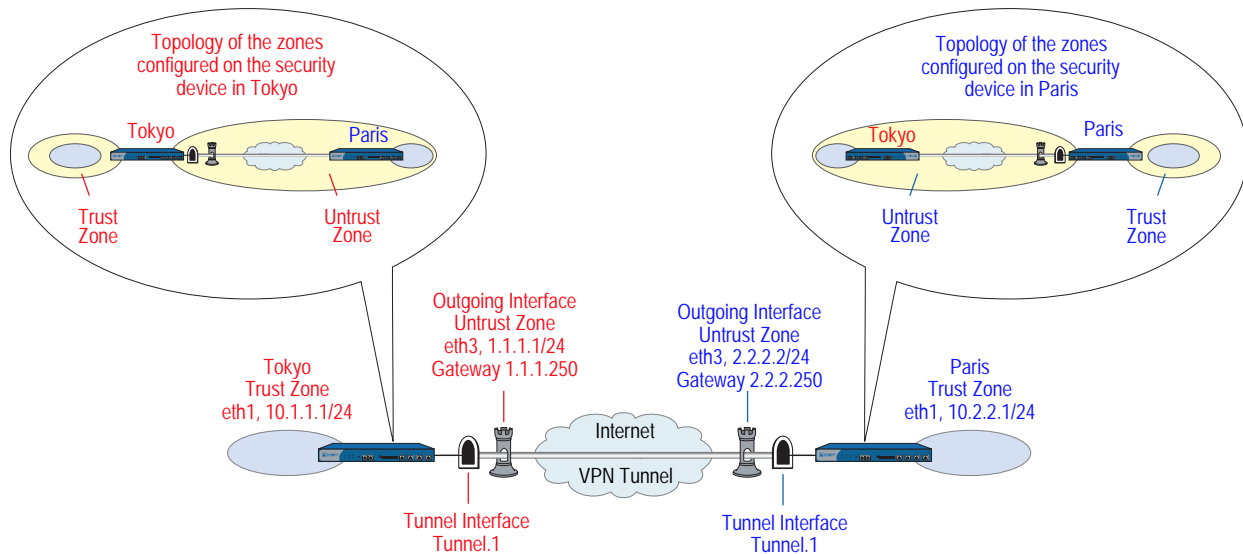
Figure 29: Route-Based Site-to-Site VPN, AutoKey IKE
