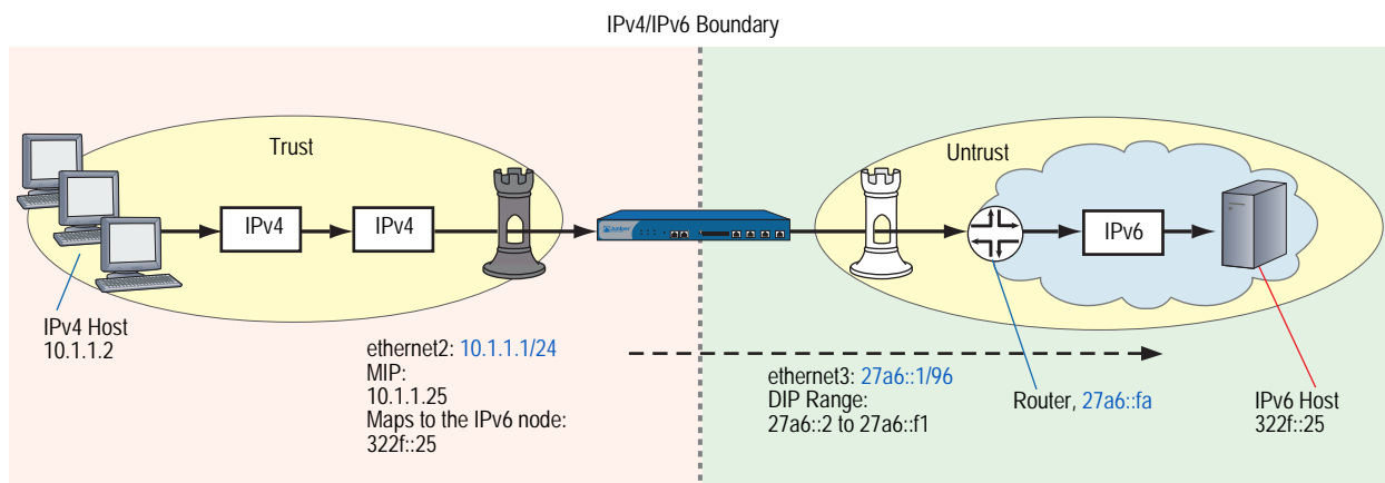
Figure 24: IPv4-to-IPv6 Host Mapping
