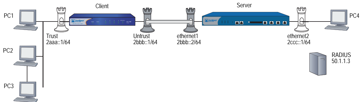
Figure 38: RADIUS with Multiple Hosts and a Single Server
