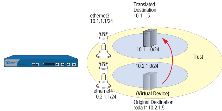
Figure 25: Original and Translated Addresses Using Different Egress Interfaces
