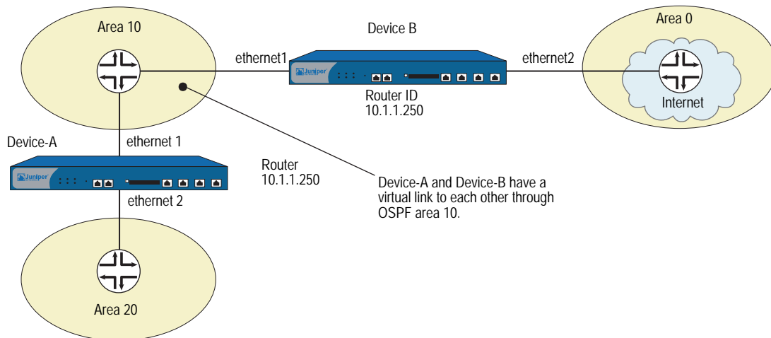
Figure 10: Creating a Virtual Link
