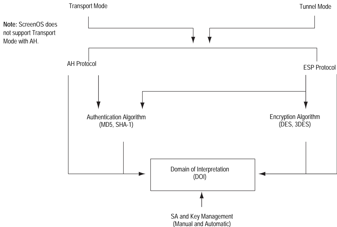
Figure 1: IPSec Architecture
