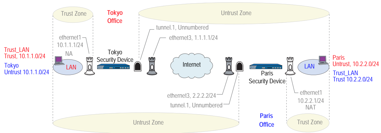
Figure 25: Site-to-Site Tunnel Configuration—Addresses
