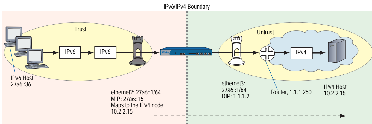
Figure 22: IPv6-to-IPv4 Host Mapping
