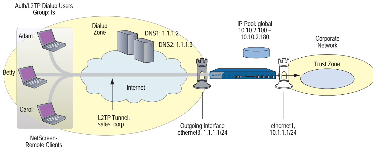
Figure 58: Configuring L2TP
