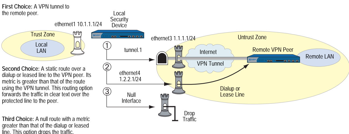
Figure 21: Routing Failover Alternatives for VPN Traffic
