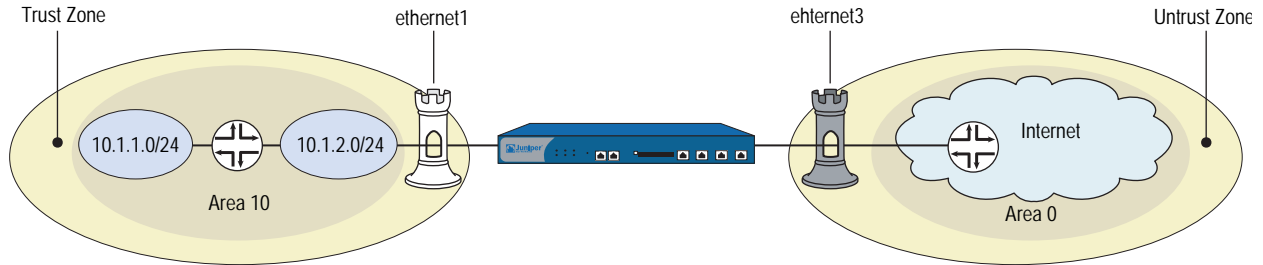
Figure 9: OSPF Configuration Example
