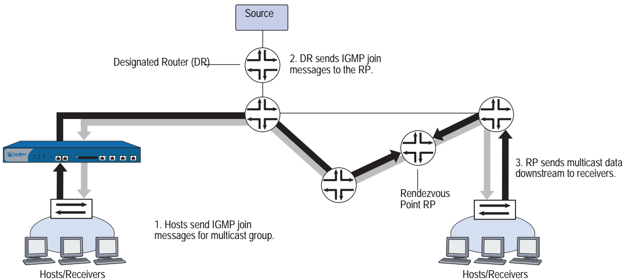
Figure 31: Host Joining a Group
