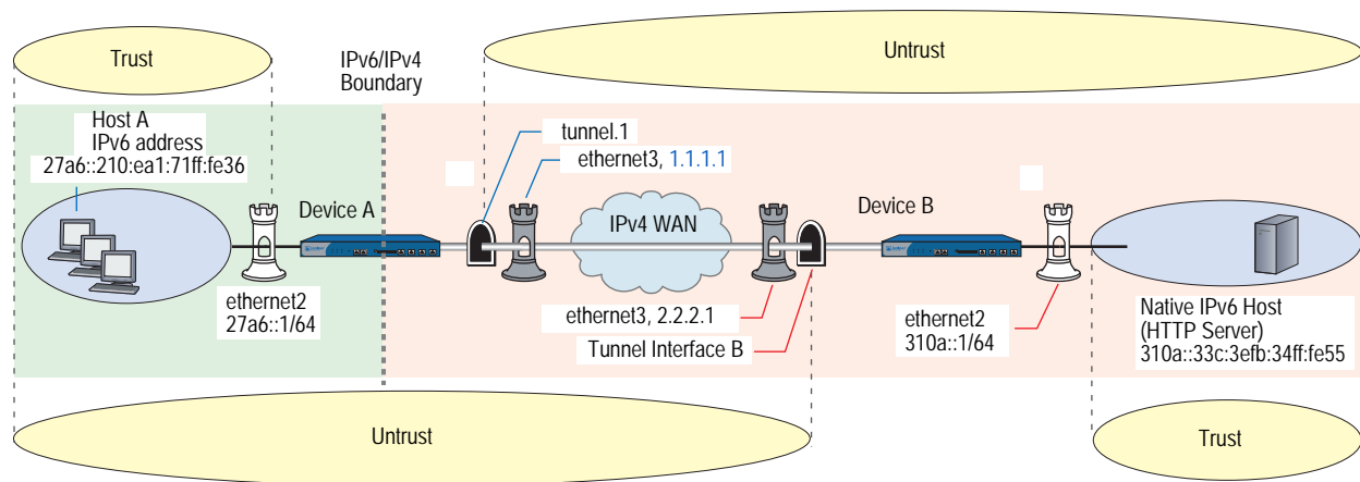
Figure 33: Tunnel Interface and Zone Example
