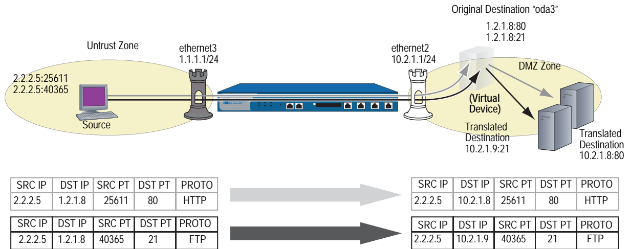
Figure 28: NAT-Dst—One-to-Many
