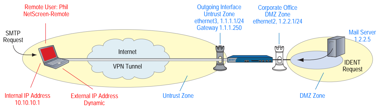
Figure 42: Policy-Based Dialup VPN, Dynamic Peer
