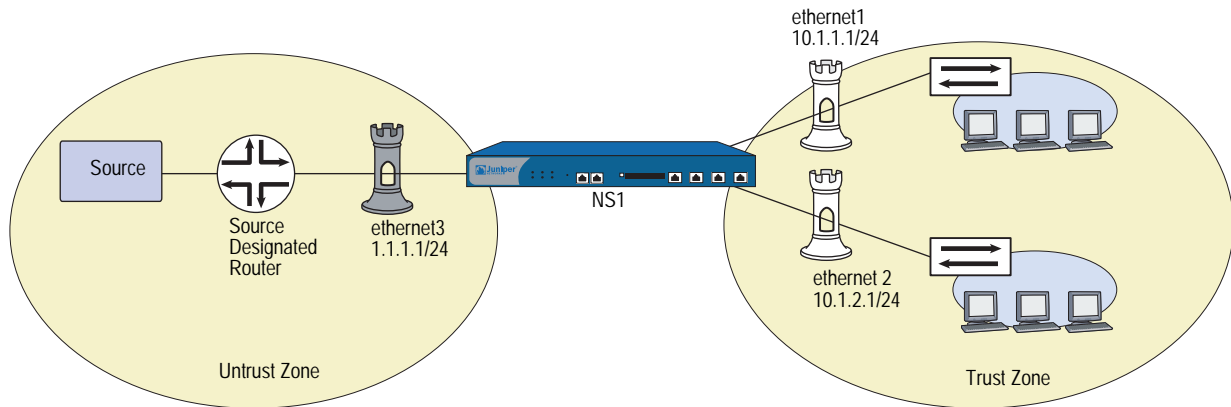
Figure 23: IGMP Configuration Example
