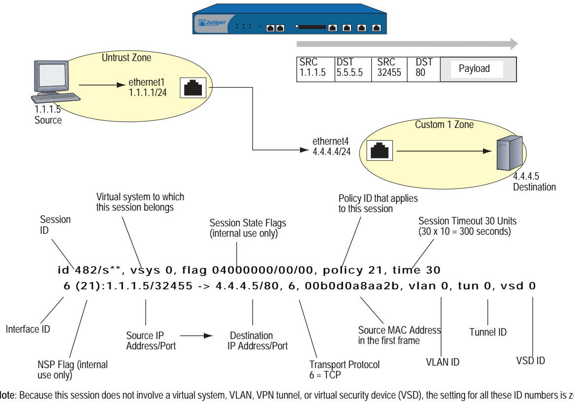
Figure 22: NAT-Dst Packet Flow—Packet Forwarding
