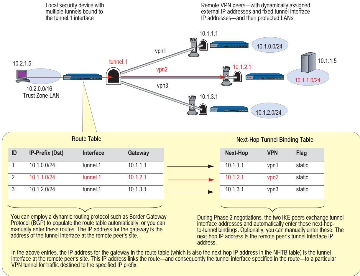
Figure 68: Route Table and Next-Hop Tunnel Binding (NHTB) Table
