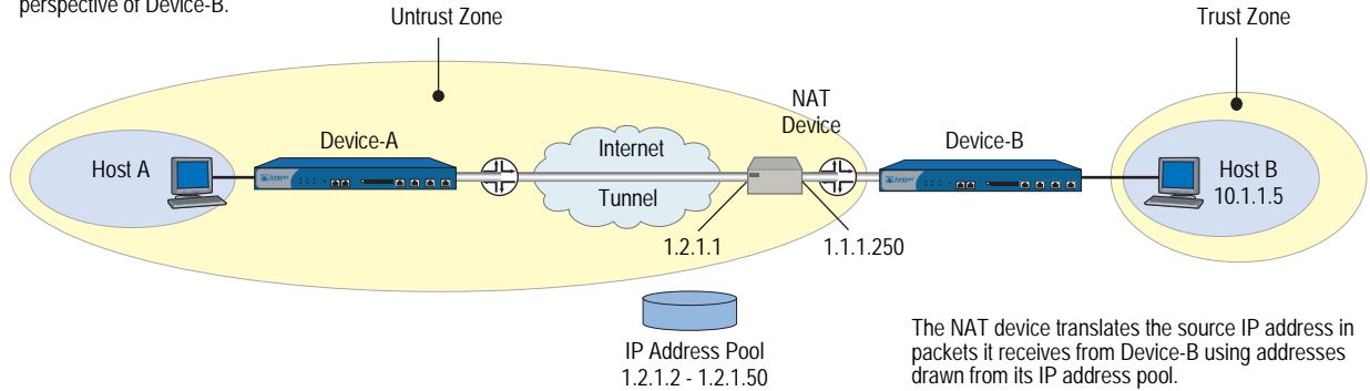
Figure 64: Security Device with a Dynamically Assigned IP Address Behind a NAT Device
