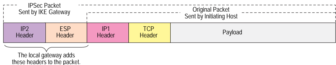
Figure 9: IPSec Packet—Encapsulating Security Payload (ESP) in Tunnel Mode
