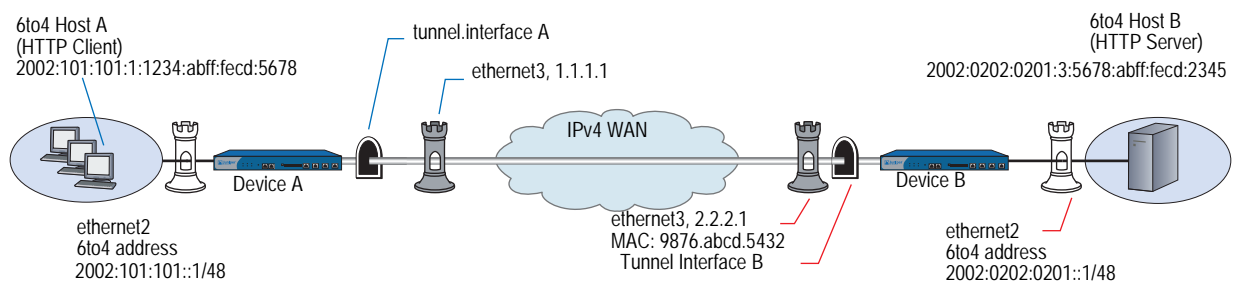
Figure 30: 6to4 Tunnel
