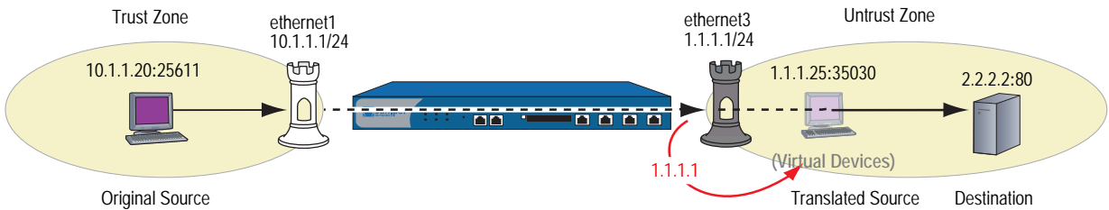
Figure 9: NAT-Src Using the Egress Interface IP Address
