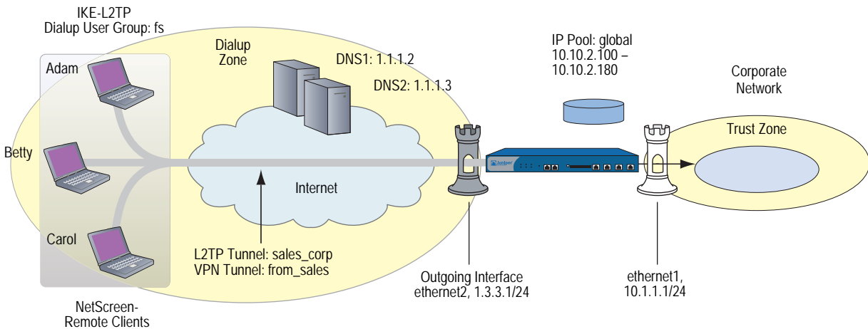
Figure 59: Configuring L2TP-over-IPSec
