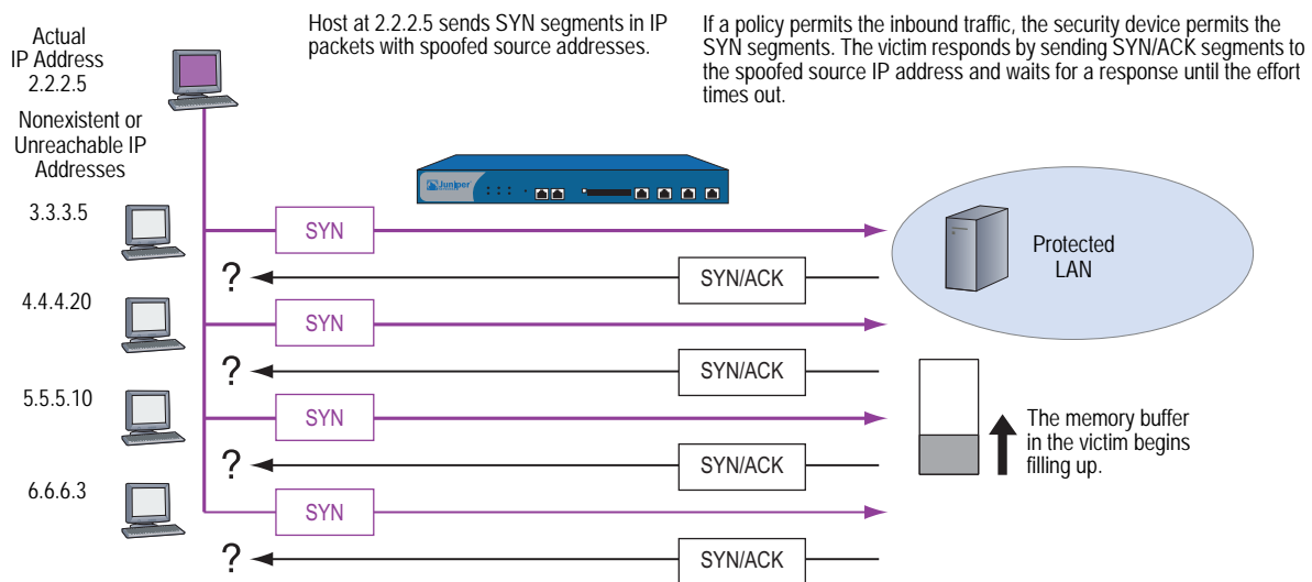
Figure 19: SYN Flood Attack
