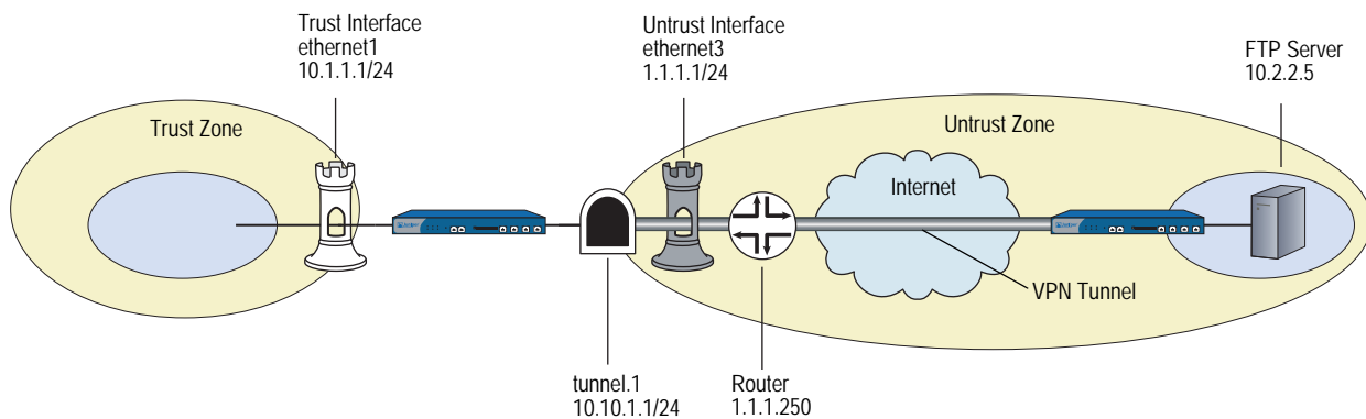
Figure 3: Static Route for a Tunnel Interface
