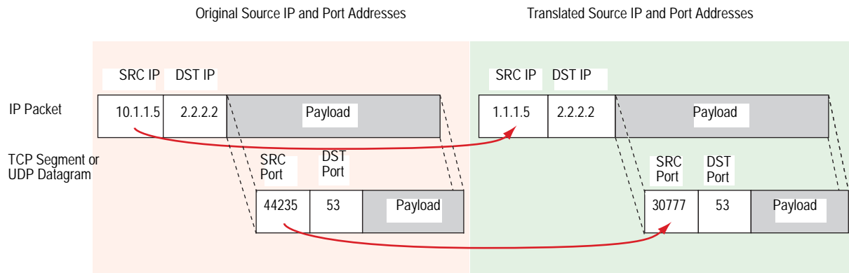
Figure 2: Source IP and Source Port Address Translation
