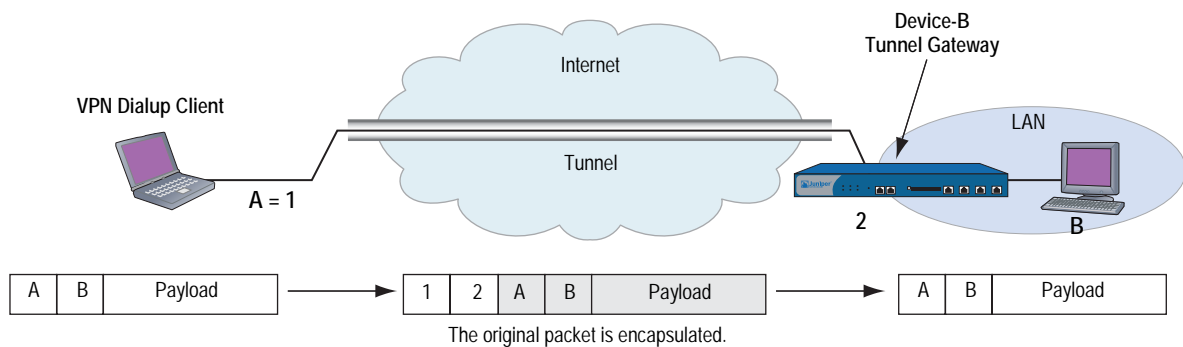
Figure 5: Dialup VPN in Tunnel Mode
