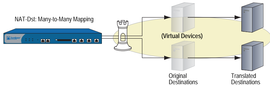
Figure 20: NAT-Dst—Many-to-Many
