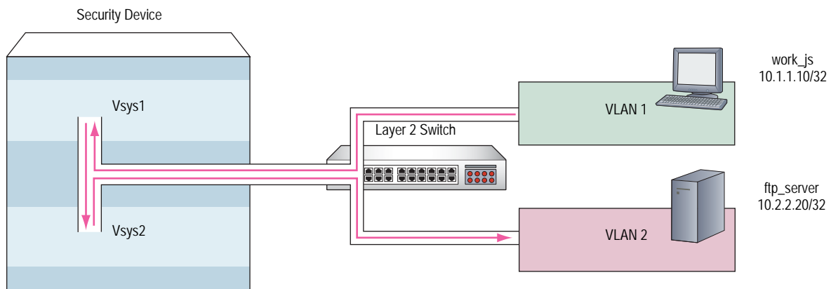
Figure 12: InterVsys Communication
