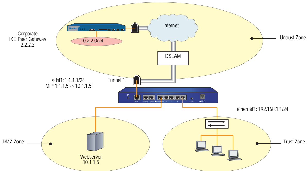
Figure 19: VPN Tunnel Through ADSL Interface
