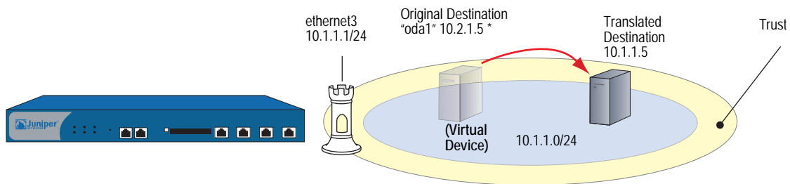
Figure 23: Original and Translated Addresses Using the Same Egress Interface
