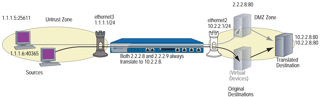
Figure 12: NAT-Dst from an Address Range to a Single IP Address
