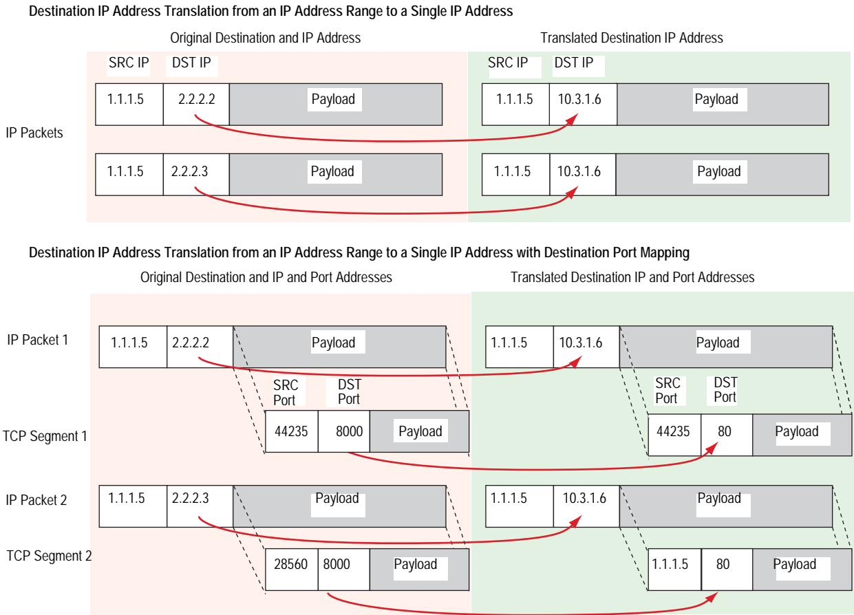
Figure 4: NAT-Dst from an IP Address Range to a Single IP Address
