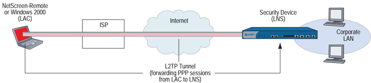
Figure 52: L2TP Tunnel Between VPN Client (LAC) and Security Device (LNS)
