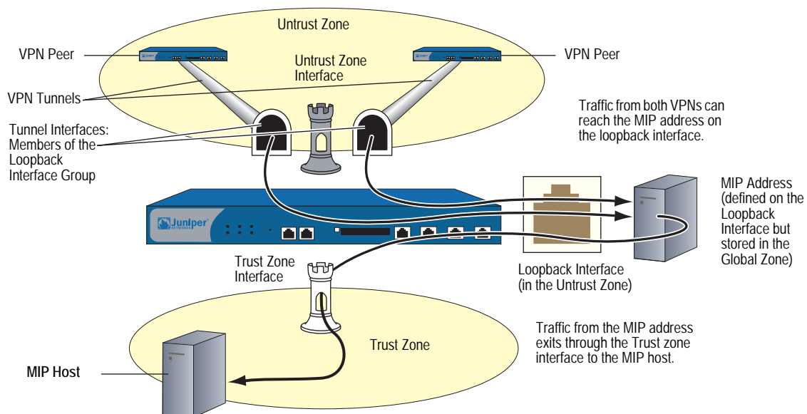
Figure 35: MIP on the Loopback Interface
