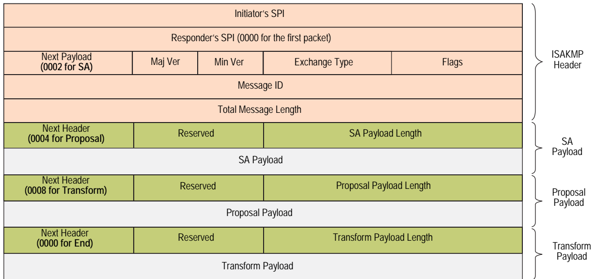
Figure 8: ISAKMP Header with Generic ISAKMP Payloads
