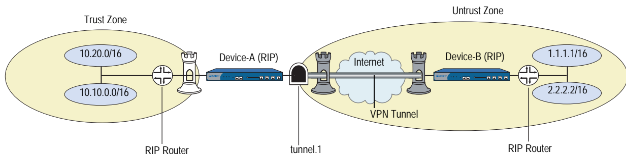
Figure 12: Tunnel Interface with RIP Example
