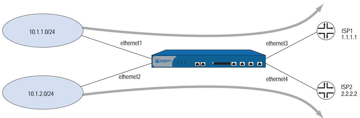
Figure 5: Source Interface-Based Routing (SIBR) Example
