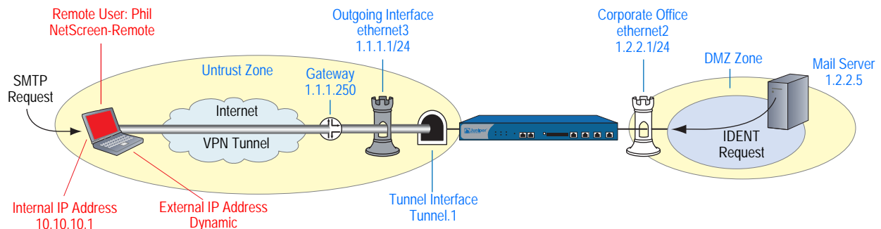
Figure 41: Route-Based Dialup VPN, Dynamic Peer
