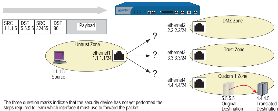
Figure 21: NAT-Dst Packet Flow—Packet Arrival
