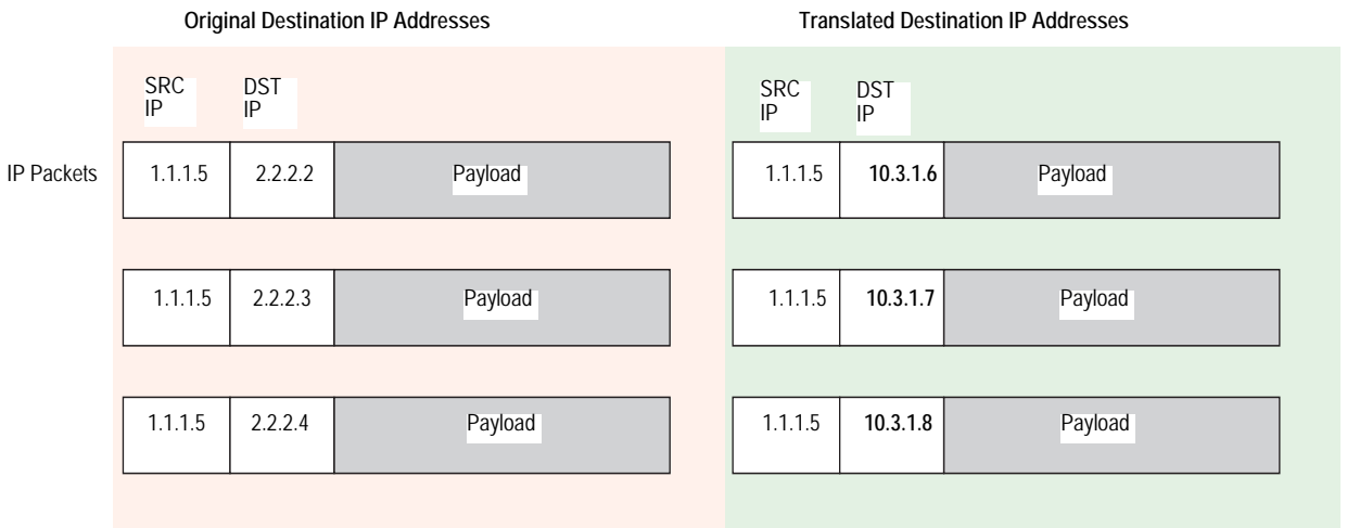
Figure 5: NAT-Dst with Address Shifting
