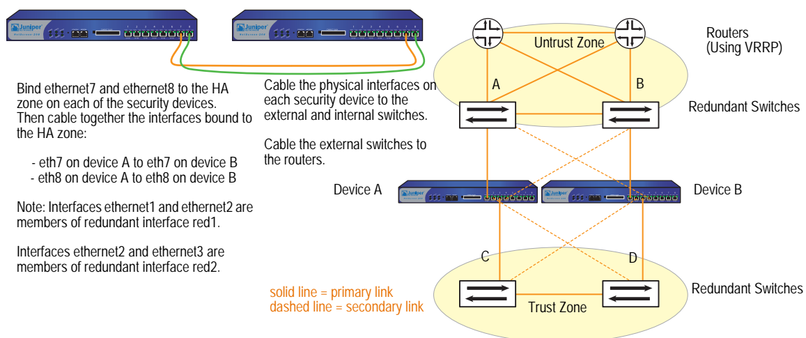
Figure 14: Security Devices Using Network Interfaces for HA Links
