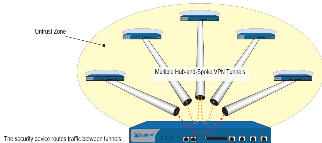
Figure 85: Multiple Tunnels in a Hub-and-Spoke VPN Configuration
