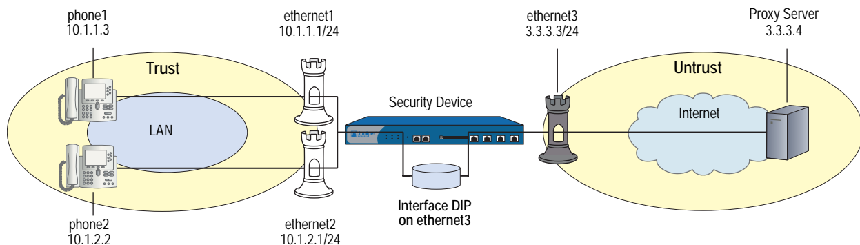
Figure 18: Trust Intrazone
