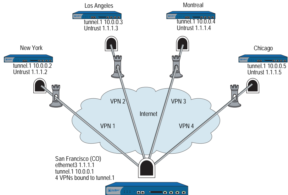
Figure 13: Point-to-MultiPoint with Tunnel Interface Network Example
