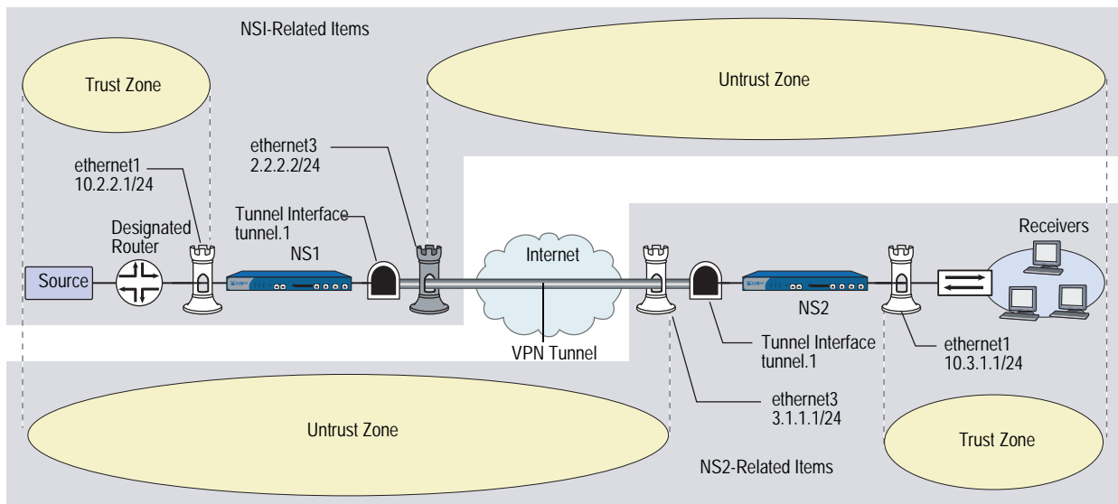
Figure 25: IGMP Proxy Configuration Between Two Devices
