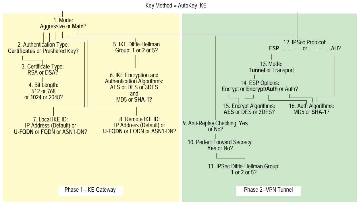
Figure 19: Cryptographic Options for a Dialup VPN Tunnel
