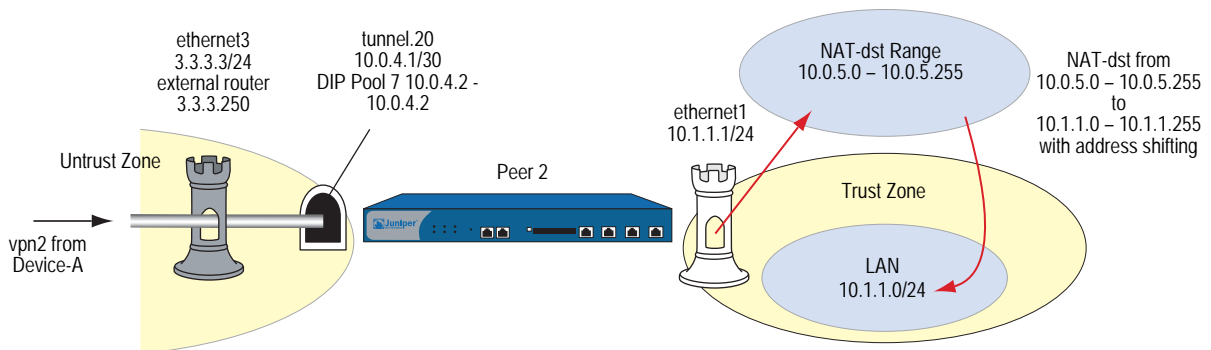
Figure 72: Peer2
