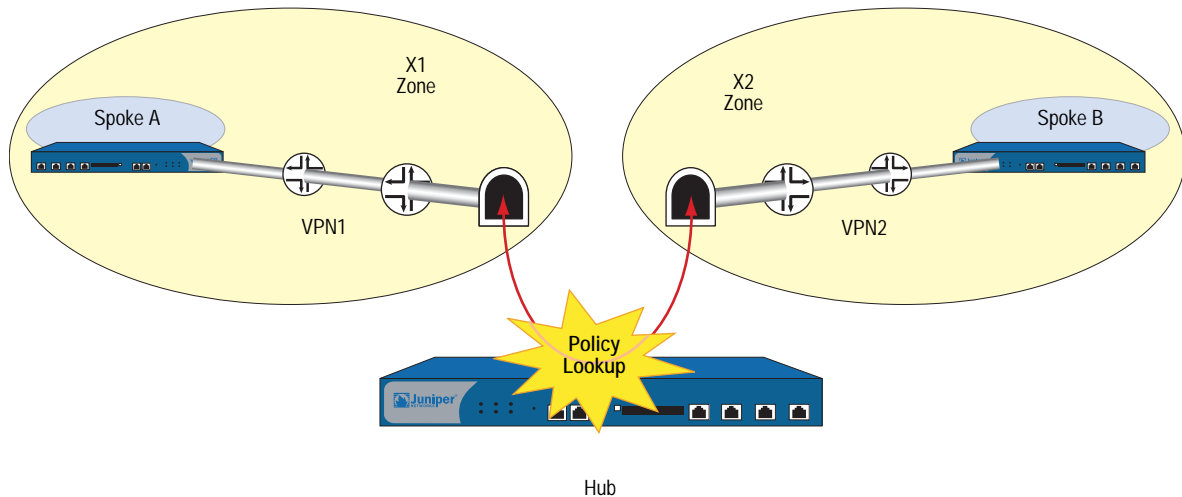
Figure 83: Back-to-Back VPNs
