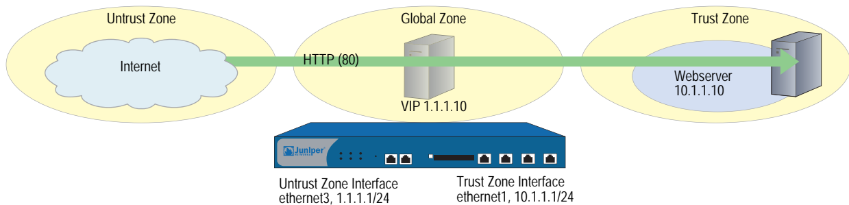
Figure 38: Virtual IP Server
