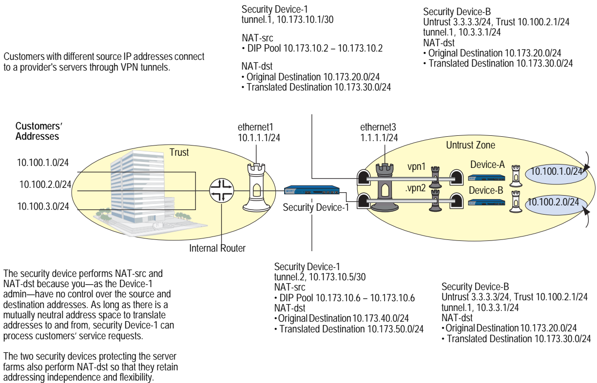
Figure 31: NAT-Src and NAT-Dst Combined
