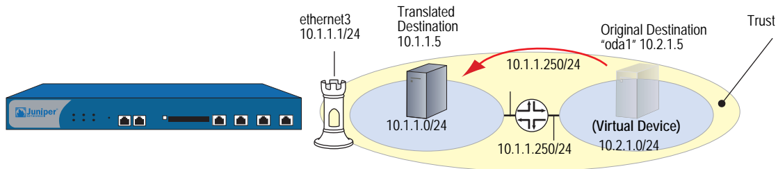
Figure 24: Original and Translated Addresses Separated by a Router
