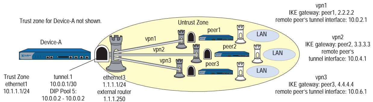
Figure 70: Tunnel.1 interface Bound to Three VPN Tunnels
