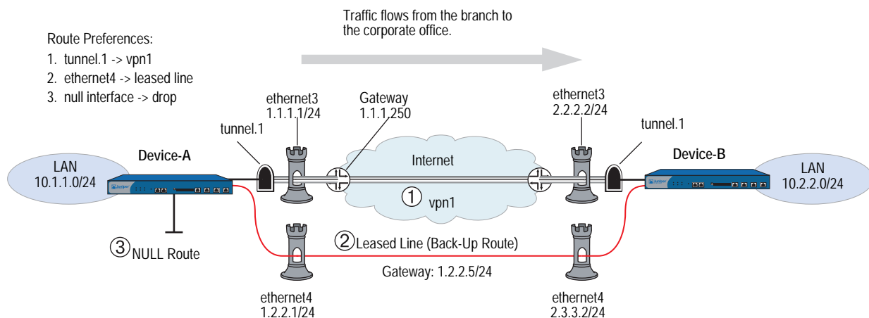
Figure 22: Routing Failover to a Leased Line and Then to a Null Route
