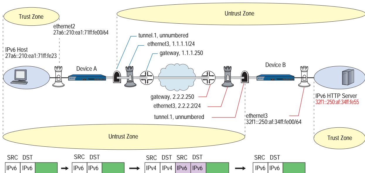
Figure 26: IPv6 Tunneling Using IPv4 Encapsulation Example
