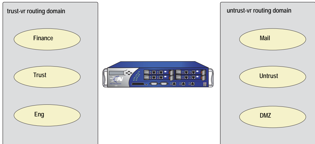
Figure 11: Zone-to-Virtual Router Bindings
