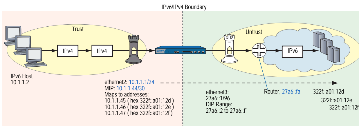
Figure 23: IPv4-to-IPv6 Network Mapping
