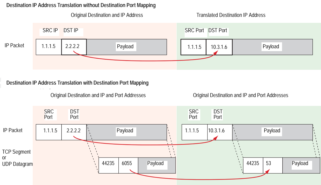
Figure 3: Destination IP Address Translation
