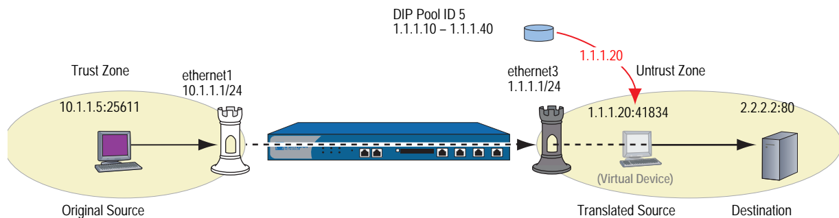
Figure 7: NAT-Src Without Port Address Translation
