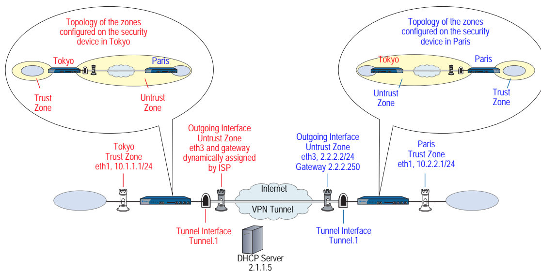
Figure 31: Route-Based Site-to-Site VPN, Dynamic Peer
