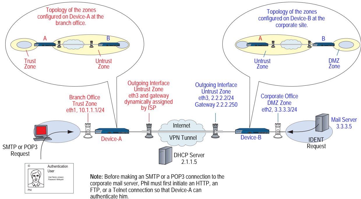
Figure 32: Policy-Based Site-to-Site VPN, Dynamic Peer
