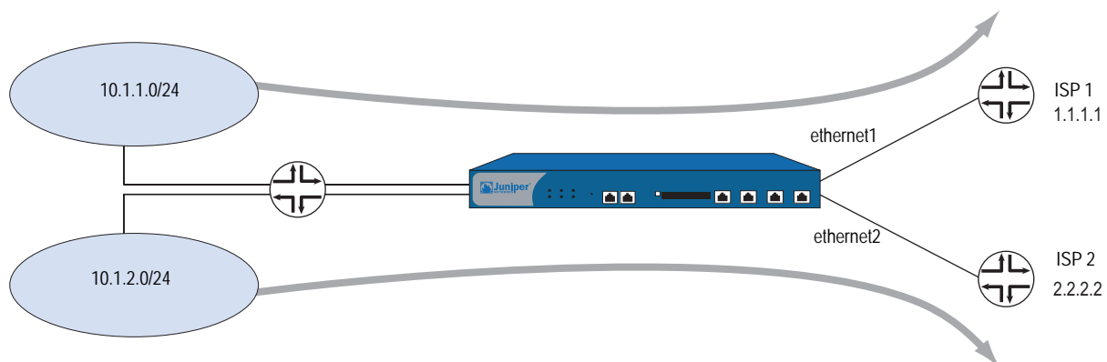
Figure 4: Source-Based Routing Example
