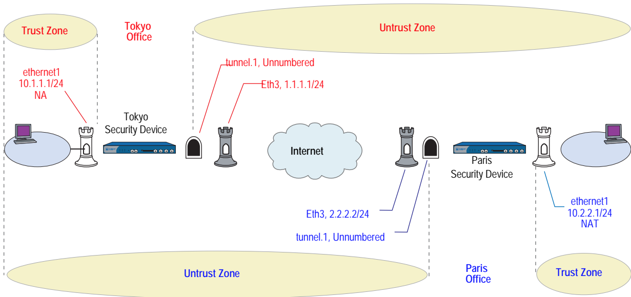
Figure 24: Site-to-Site Tunnel Configuration—Interfaces
