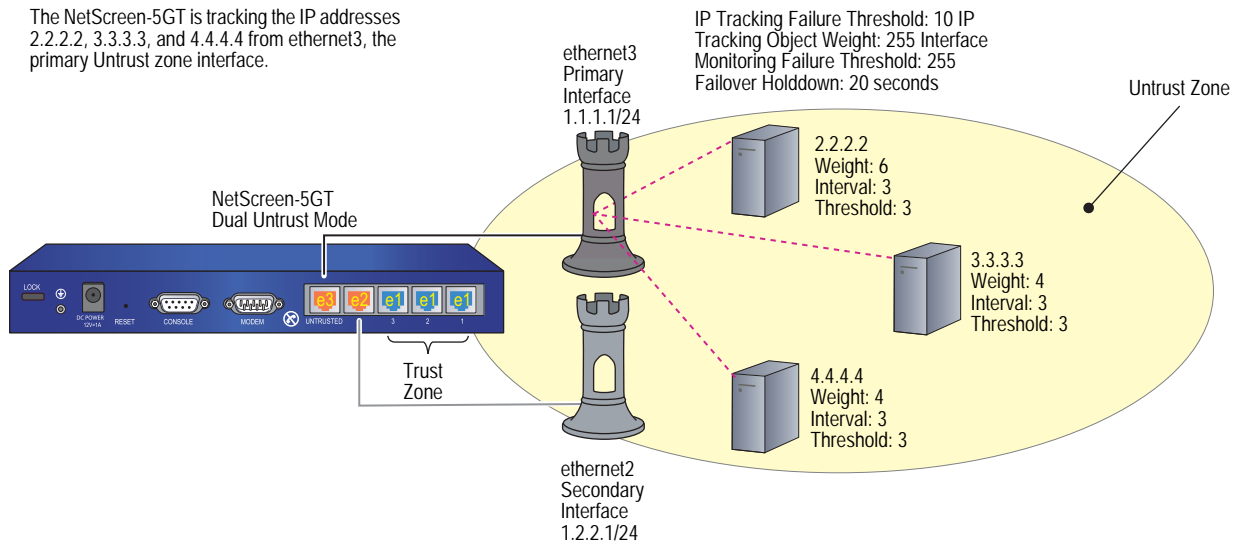
Figure 19: Interface Failover
