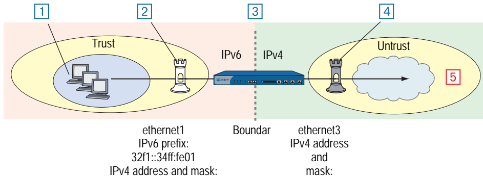
Figure 2: Packet Flow Across IPv6/IPv4 Boundary
