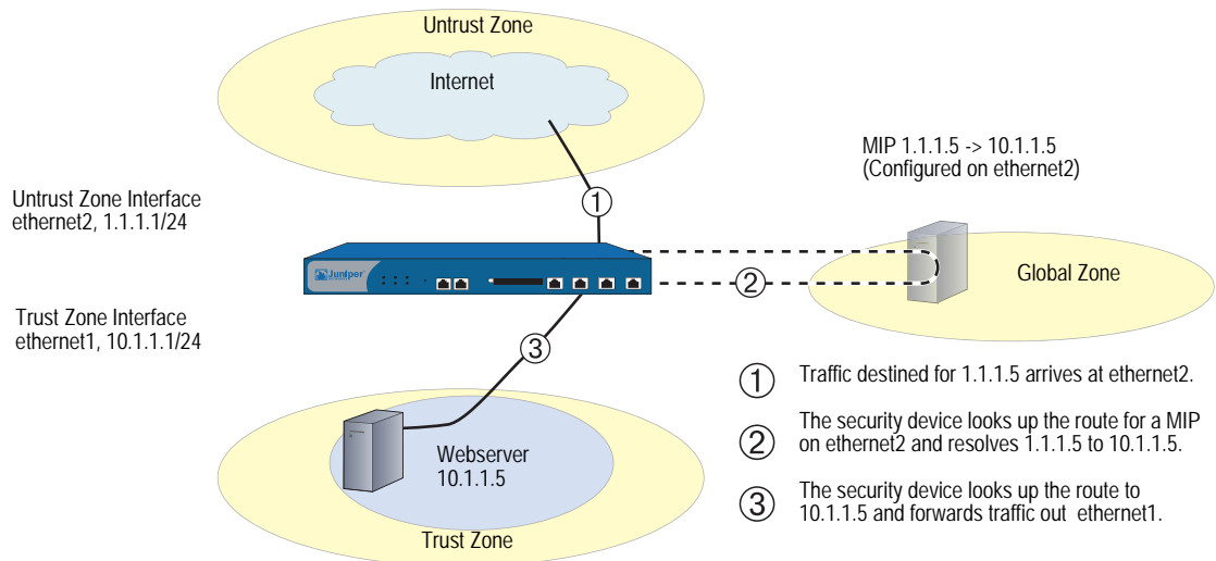
Figure 33: MIP on Untrust Zone Interface
