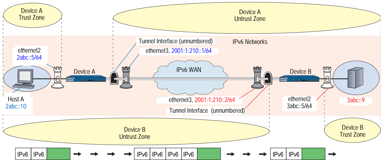
Figure 31: IPSec with 6in6 Tunnel Example
