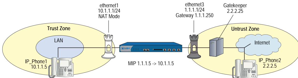
Figure 6: Gatekeeper in the Untrust Zone
