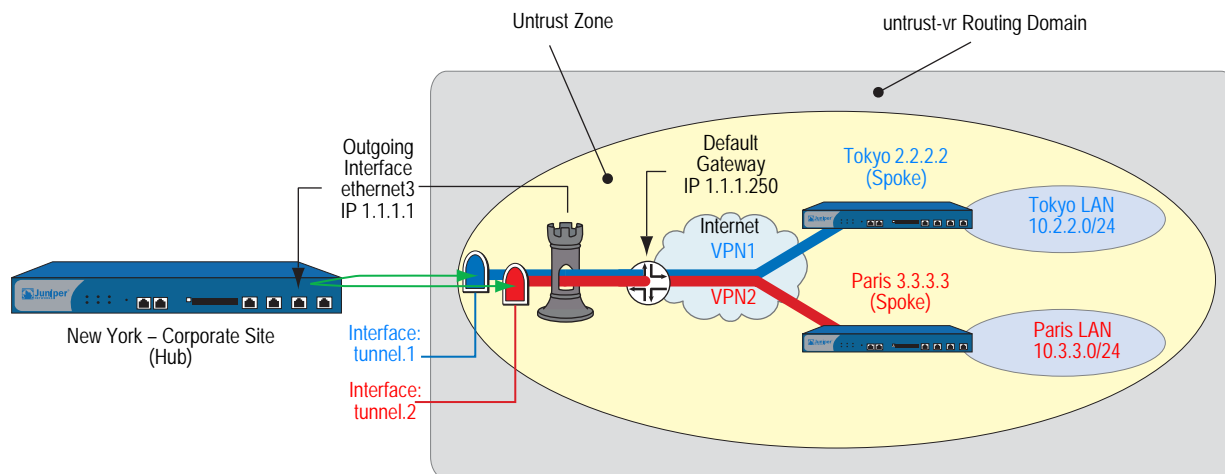
Figure 86: Hub-and-Spoke VPNs
