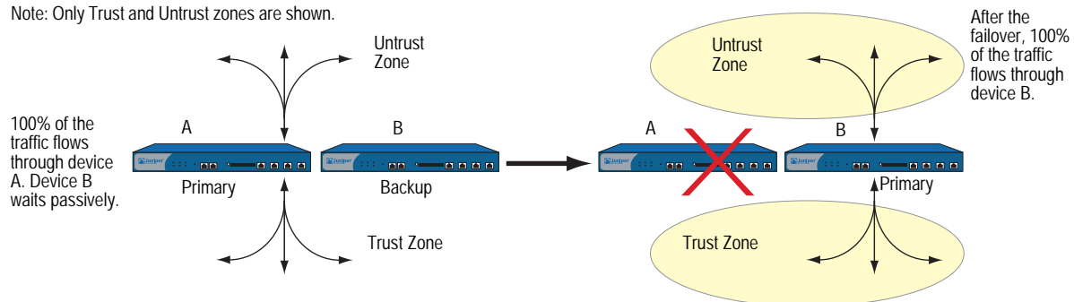
Figure 3: Active/Passive Failover
