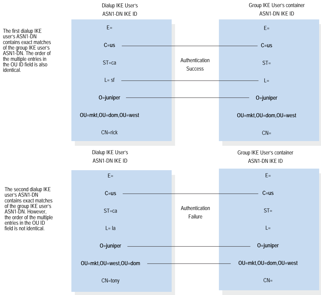
Figure 46: Authentication Success and Failure Using Container ASN1-DN IDs
