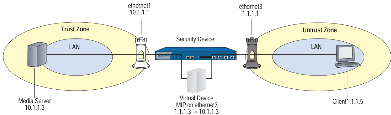
Figure 60: RTSP Private Domain
