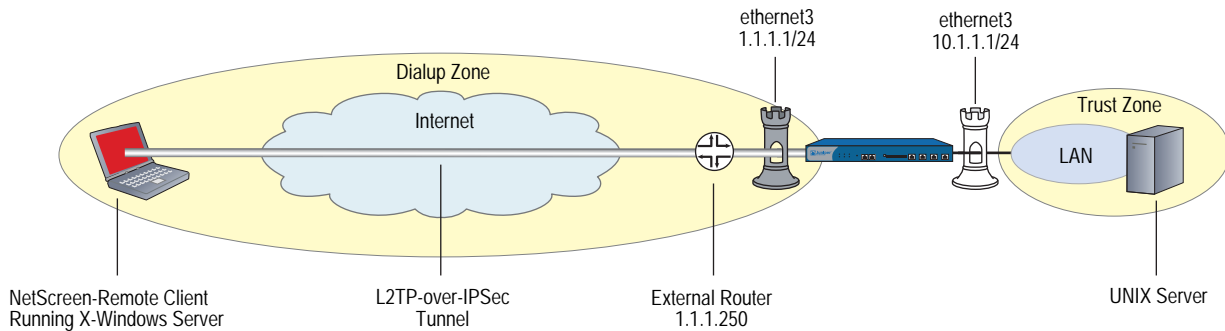
Figure 60: Bidirectional L2TP-over-IPSec
