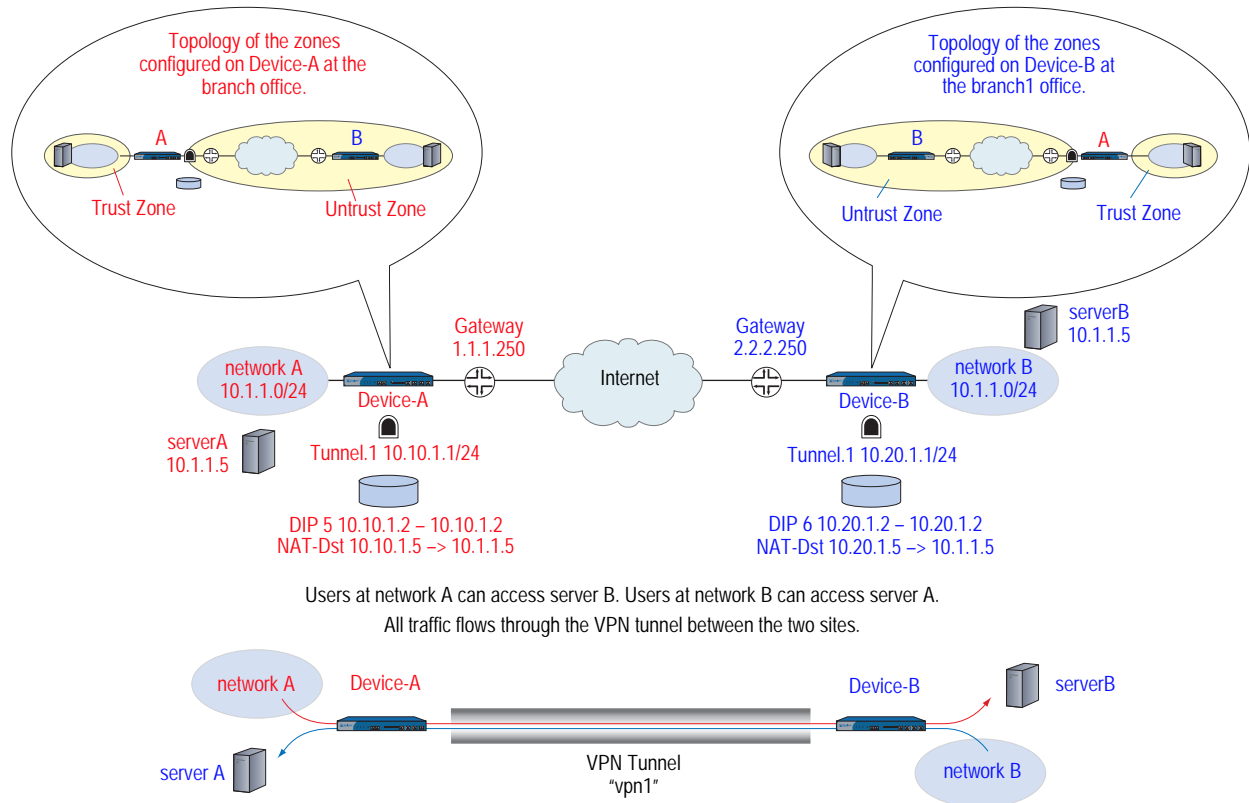
Figure 39: Tunnel Interface with NAT-Src and NAT-Dst
