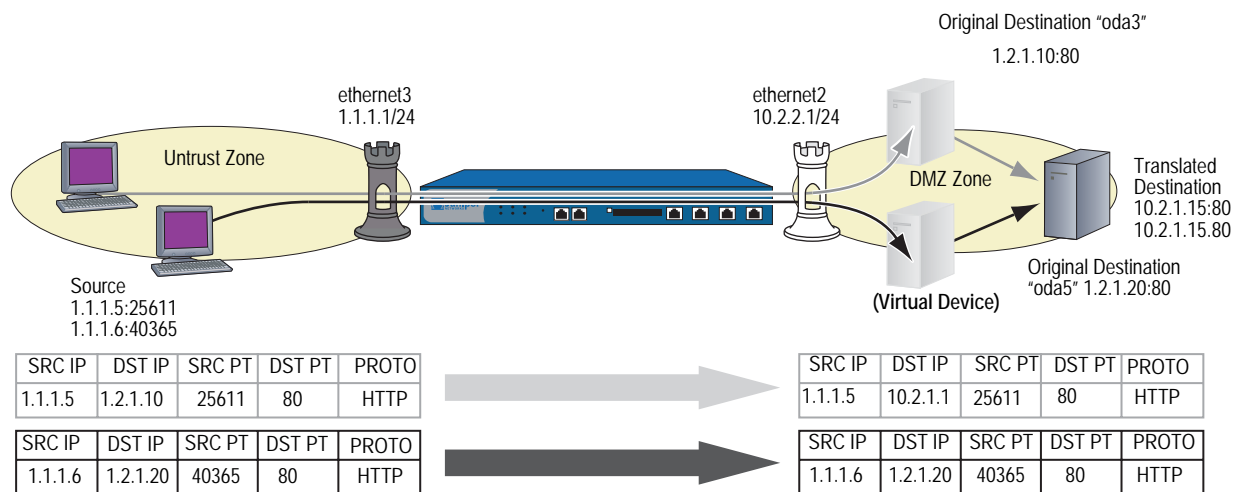
Figure 29: NAT-Dst—Many-to-One
