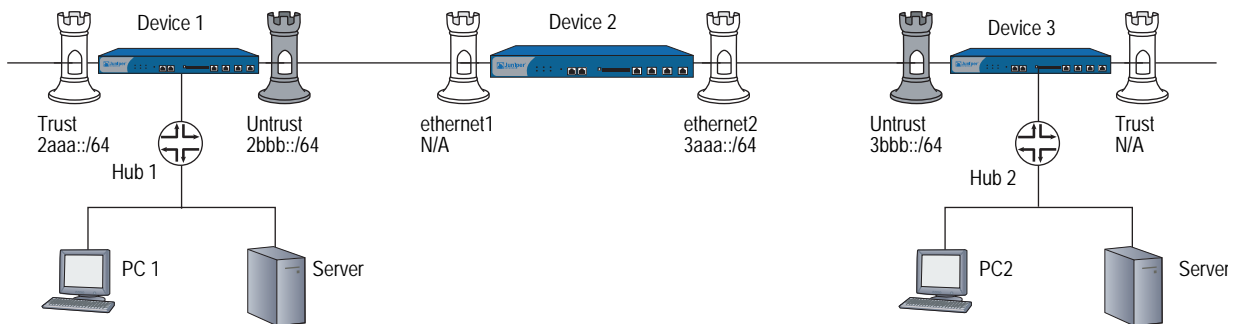
Figure 34: Manual Tunneling Example
