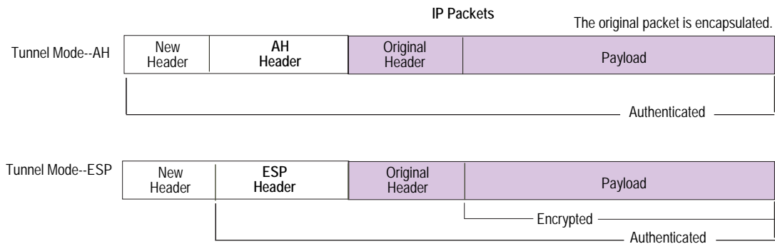
Figure 3: Tunnel Modes
