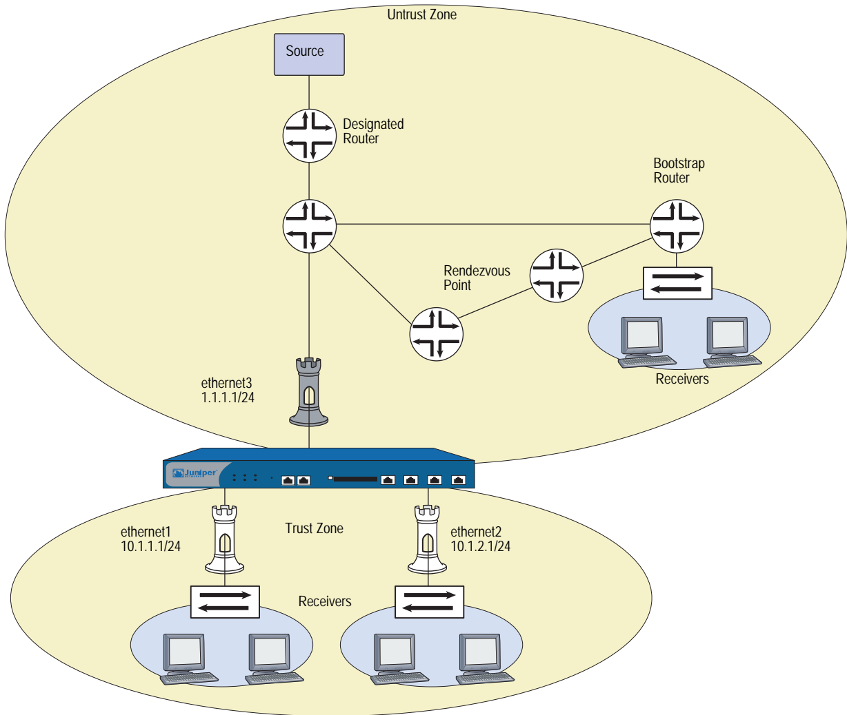
Figure 32: Basic PIM-SM Configuration
