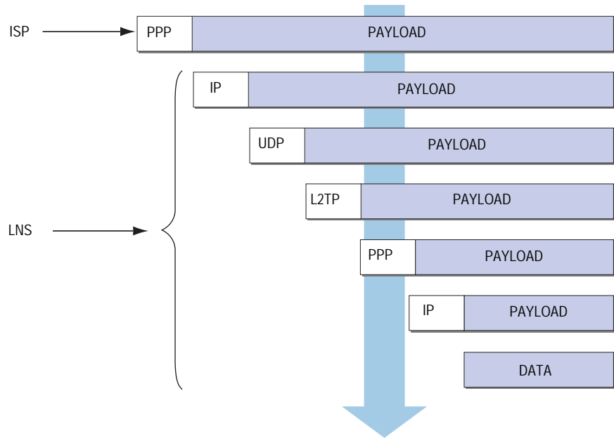
Figure 56: L2TP Packet Decapsulation
