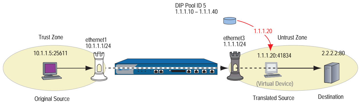
Figure 6: NAT-Src with Port Address Translation
