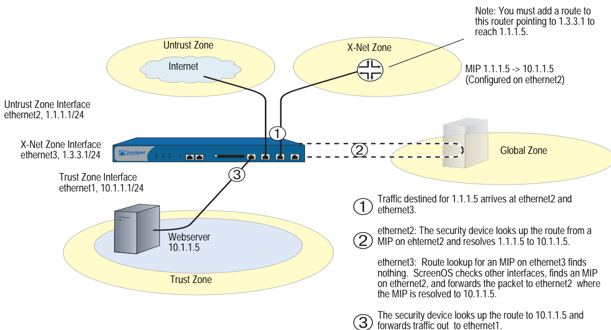
Figure 34: Reaching a MIP from Different Zones
