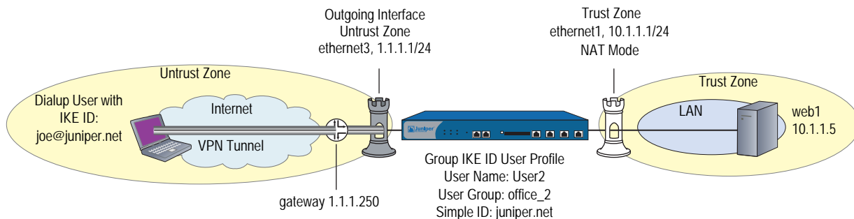
Figure 49: Group IKE ID (Preshared Keys)
