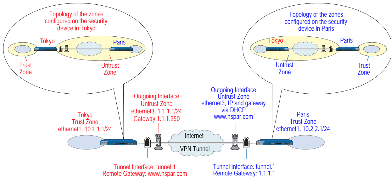
Figure 37: AutoKey IKE Peer with FQDN
