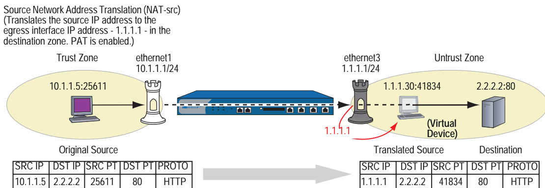
Figure 18: NAT-Src Without DIP
