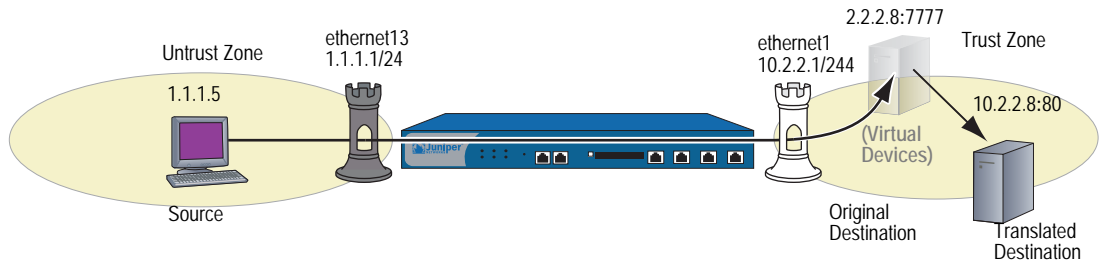
Figure 11: NAT-Dst Without Port Mapping
