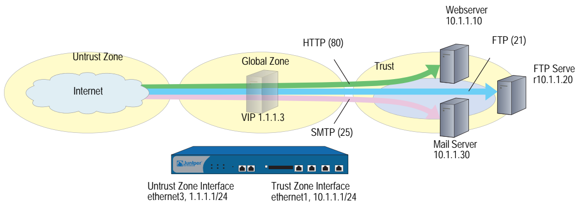
Figure 37: Virtual IP Address
