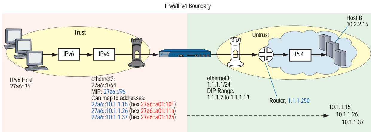
Figure 21: IPv4-Mapped Addresses
