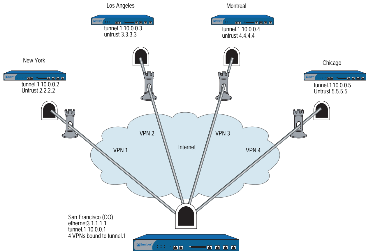
Figure 11: Point-to-MultiPoint Network Example
