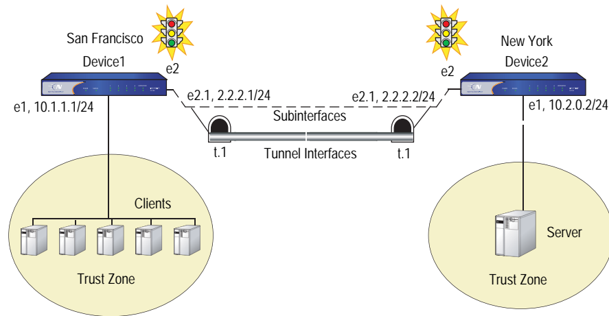
Figure 76: Route-Based VPN
