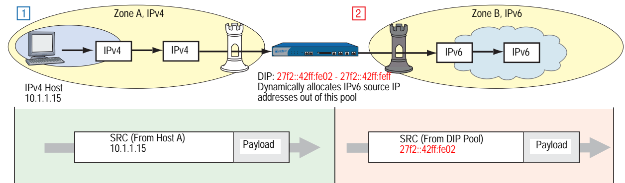
Figure 18: DIP from IPv4 to IPv6
