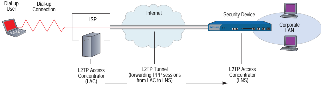
Figure 51: L2TP Tunnel Between ISP (LAC) and Security Device (LNS)
