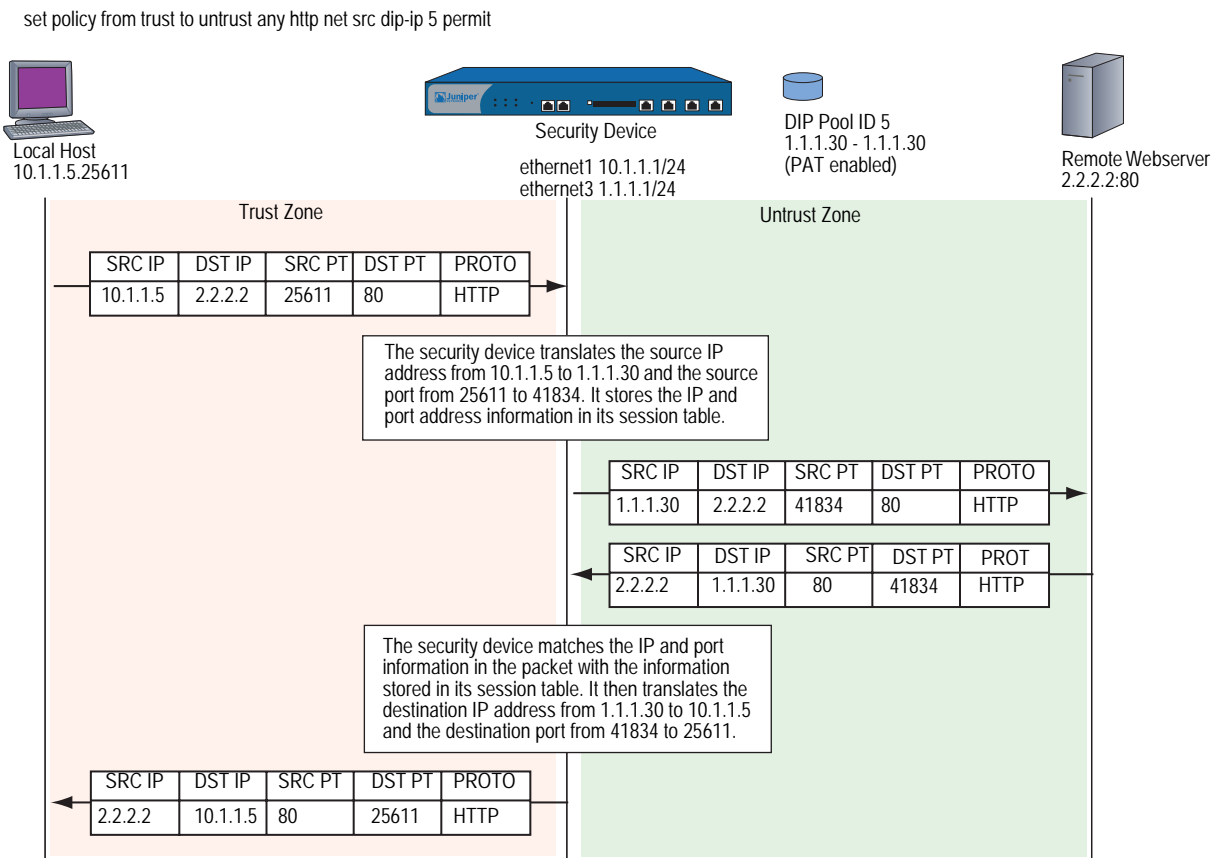
Figure 16: NAT-Src Using a DIP Pool with PAT Enabled
