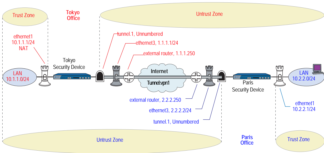
Figure 23: Site-to-Site VPN Tunnel Configuration
