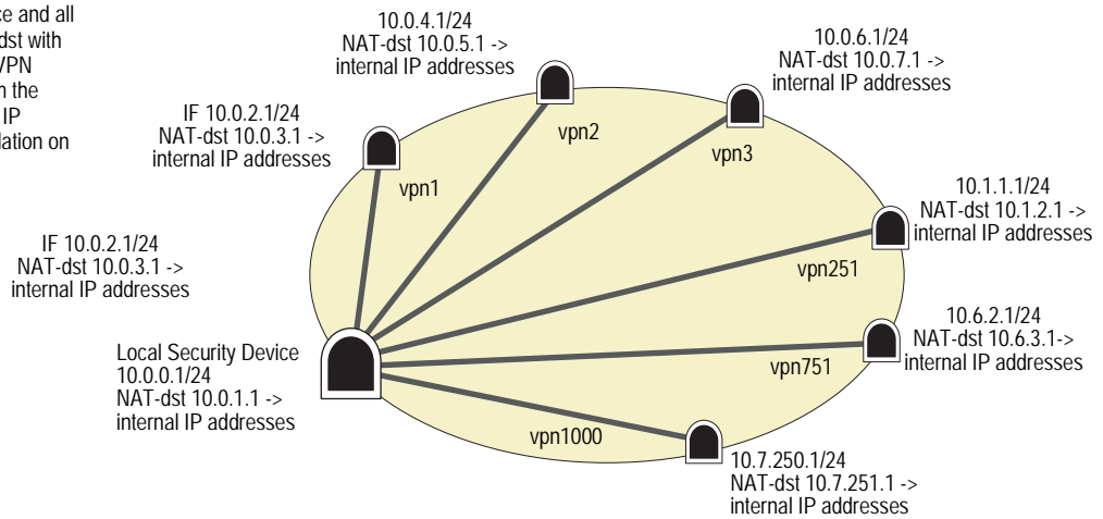
Figure 69: Multiple Tunnels Bound to a Single Tunnel Interface with Address Translation
