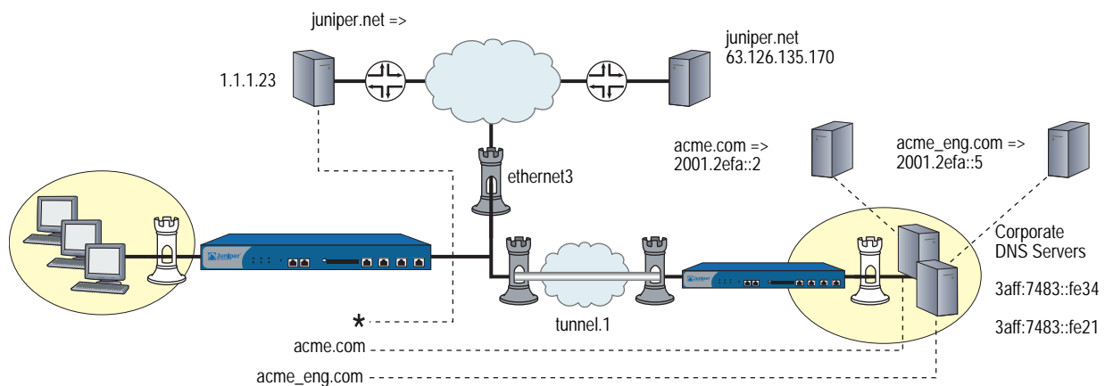
Figure 11: Proxy DNS Using Split Servers
