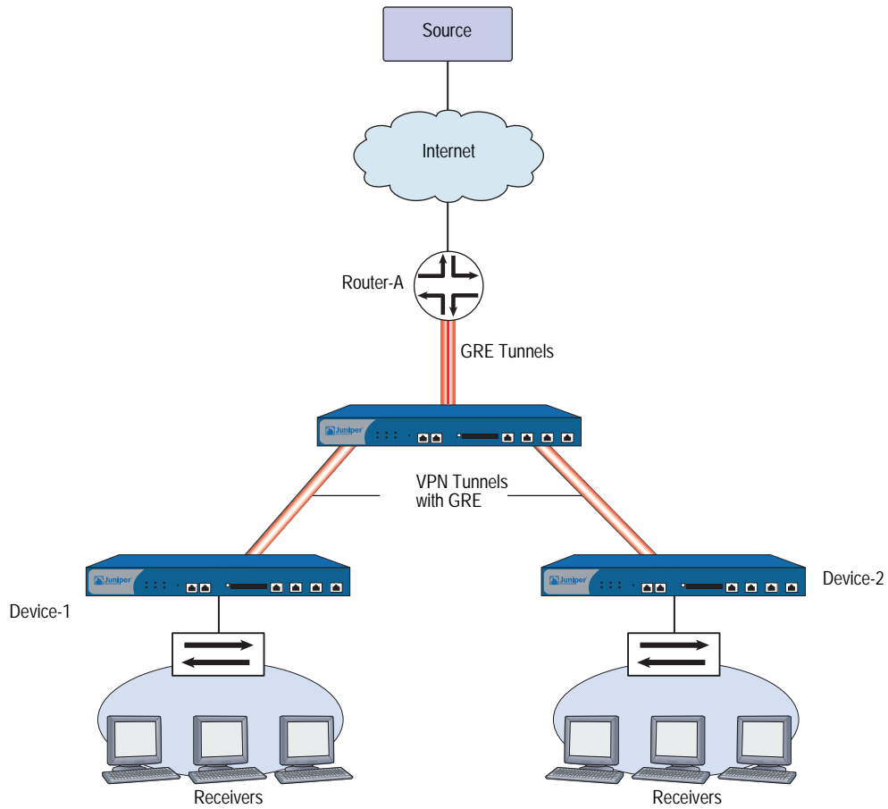
Figure 22: GRE on Tunnel Interfaces
