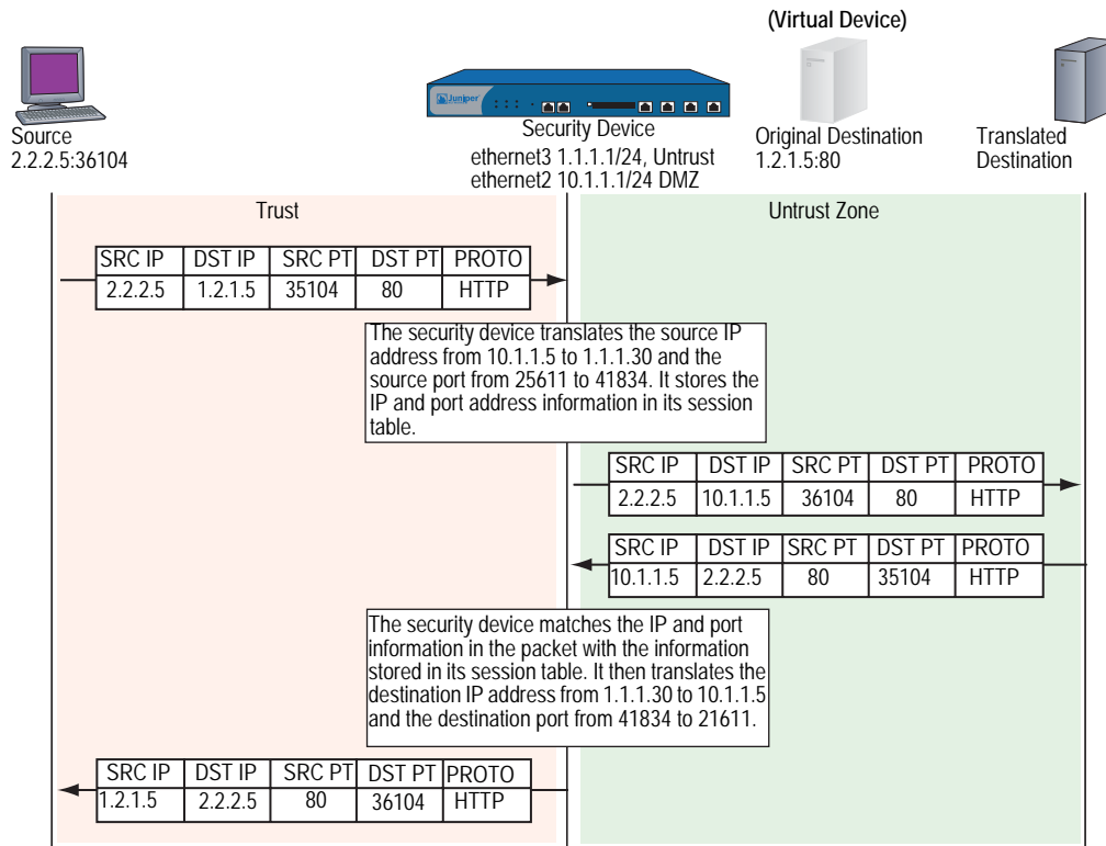
Figure 26: One-to-One NAT-Dst
