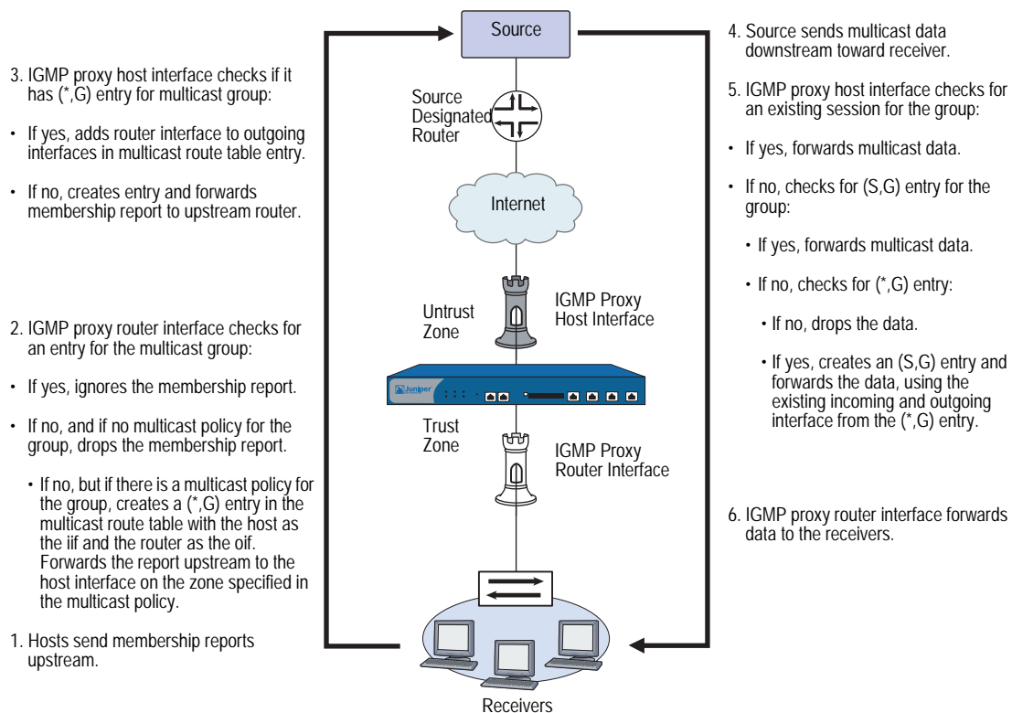
Figure 24: IGMP Proxy Host Configuration
