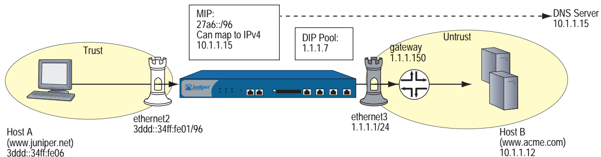
Figure 25: NAT-PT DNS Example
