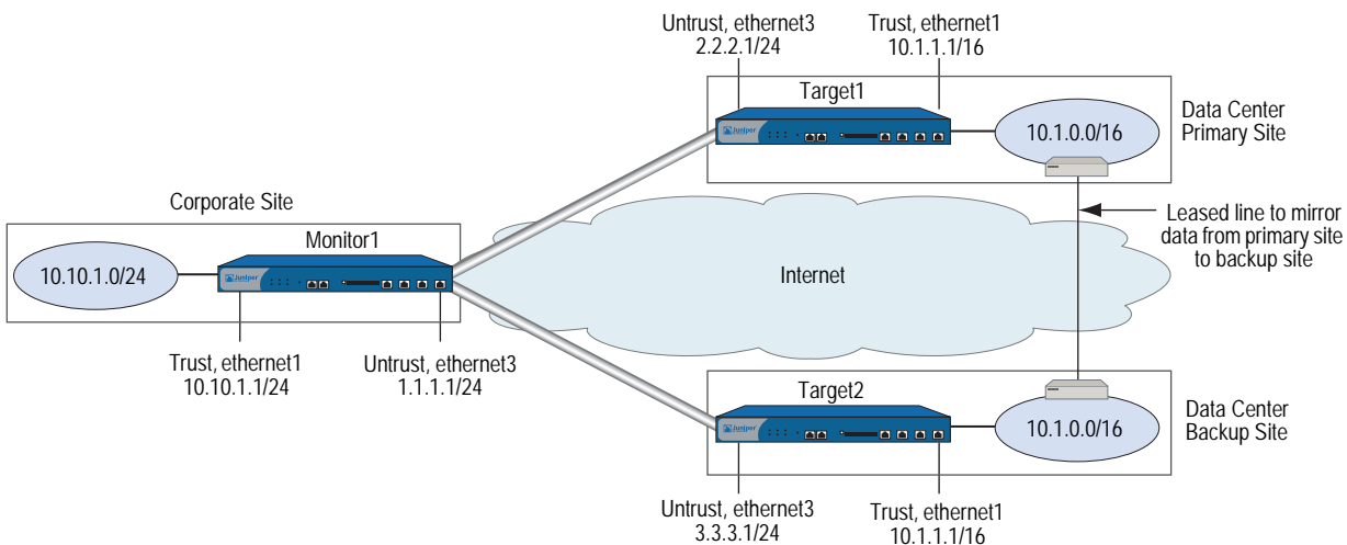
Figure 82: Redundant VPN Gateways
