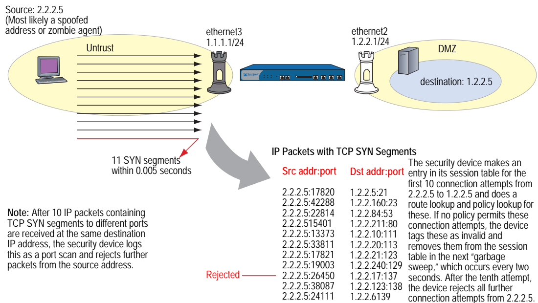
Figure 2: Port Scan
