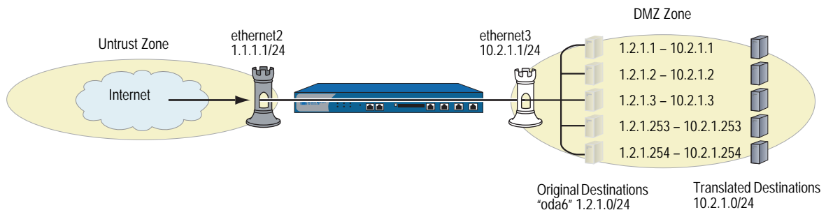
Figure 30: NAT-Dst—Many-to-Many
