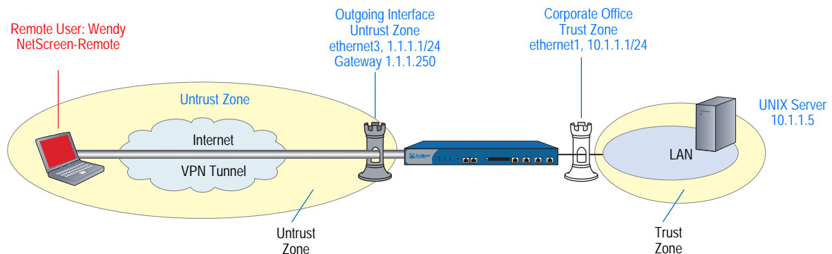
Figure 40: Policy-Based Dialup VPN, AutoKey IKE
