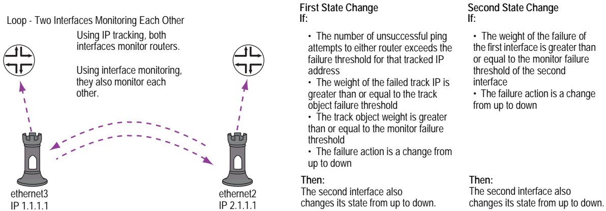
Figure 36: Loop Monitoring
