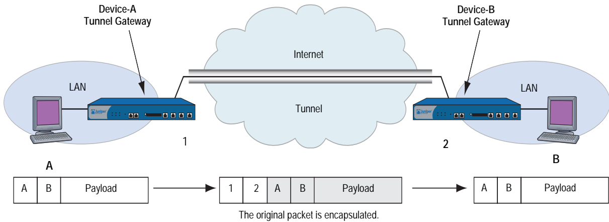
Figure 4: Site-to-Site VPN in Tunnel Mode
