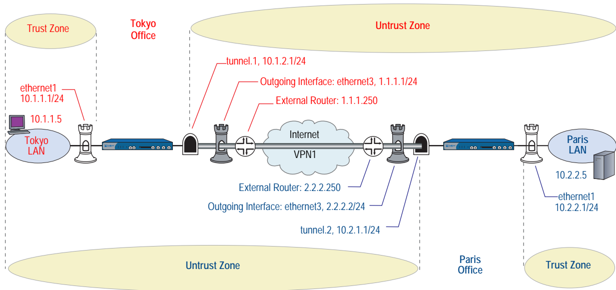
Figure 20: Site-to-Site VPN Tunnel
