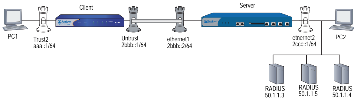
Figure 37: RADIUS with a Single Client and Multiple Servers
