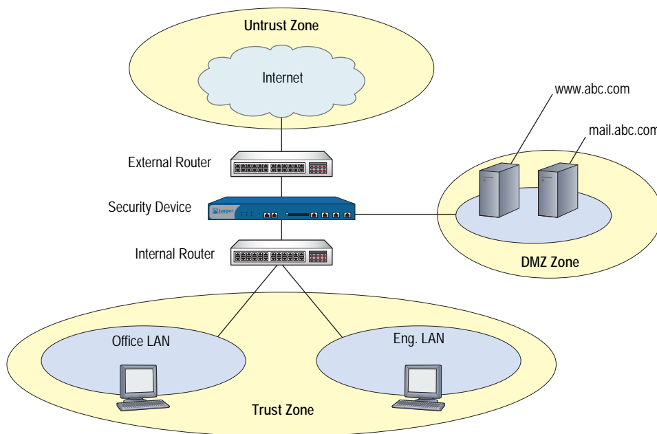
Figure 70: Interzone Policy Set
