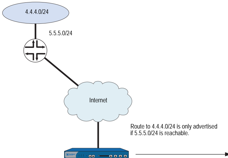
Figure 15: Conditional BGP Route Advertisement Example
