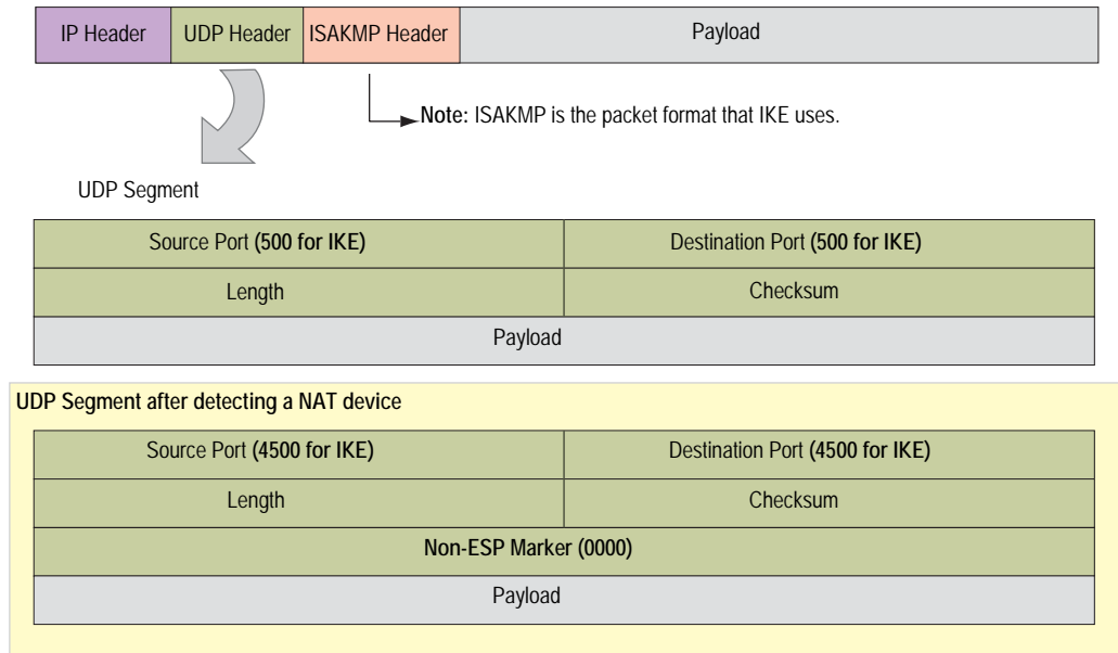
Figure 62: IKE Packet (for Phases 1 and 2)
