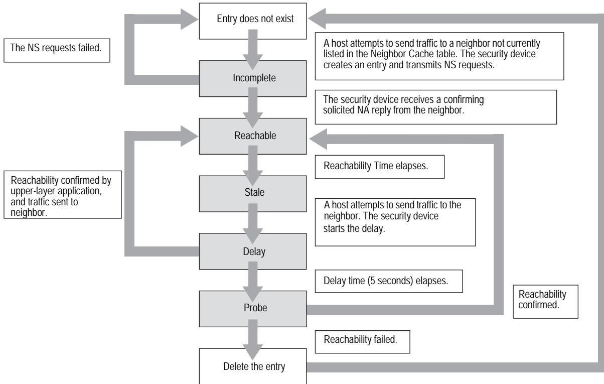
Figure 4: Endpoint Host Reachability Transitions
