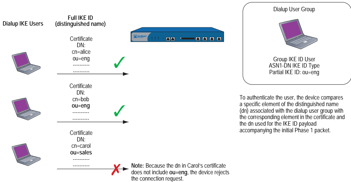
Figure 43: Group IKE ID with Certificates
