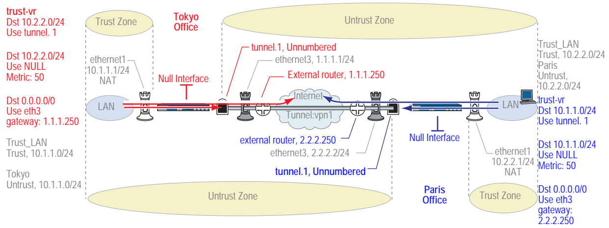
Figure 27: Site-to-Site Tunnel Configuration—Routes
