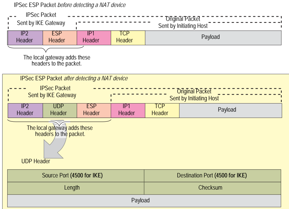
Figure 63: IPSec ESP Packet Before and After NAT Detection
