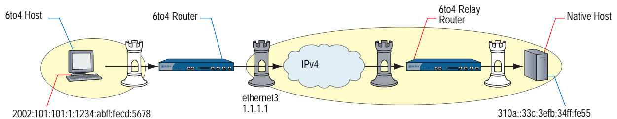
Figure 28: 6to4 Routers with Native Addresses
