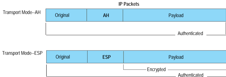
Figure 2: Transport Modes
