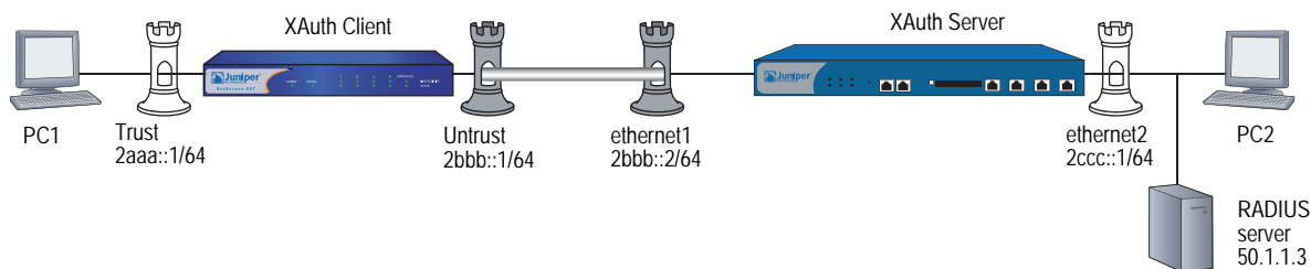
Figure 35: RADIUS with a Single Client and Single Server
