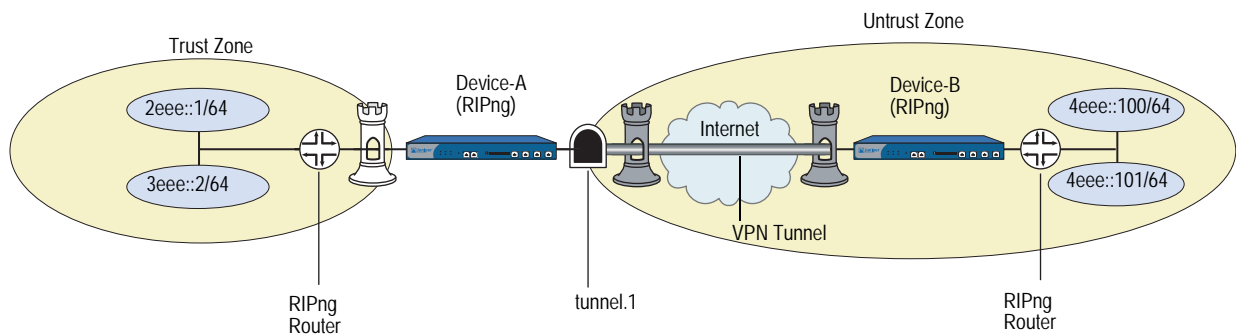
Figure 14: Tunnel Interface with RIPng Example
