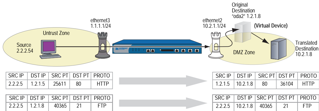
Figure 27: NAT-Dst—One-to-One
