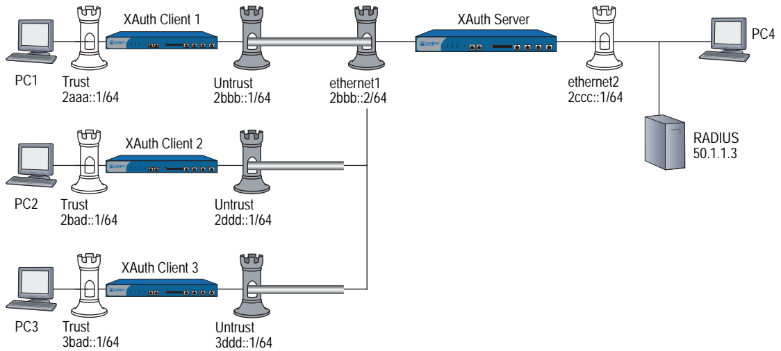
Figure 36: RADIUS with Multiple Clients and a Single Server
