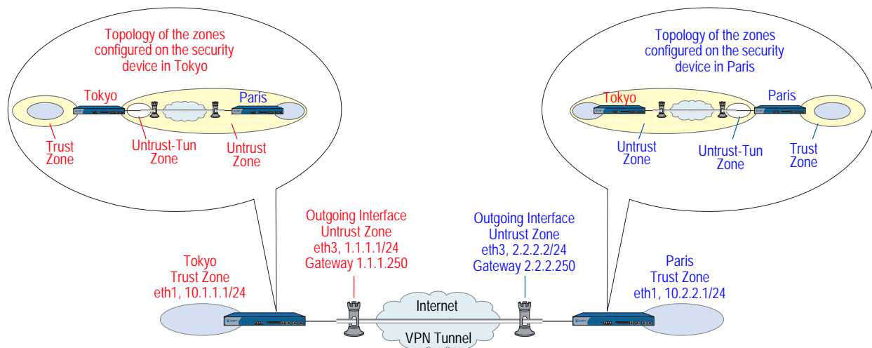
Figure 30: Policy-Based Site-to-Site VPN, AutoKey IKE
