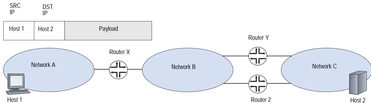
Figure 1: Static Routing Example
