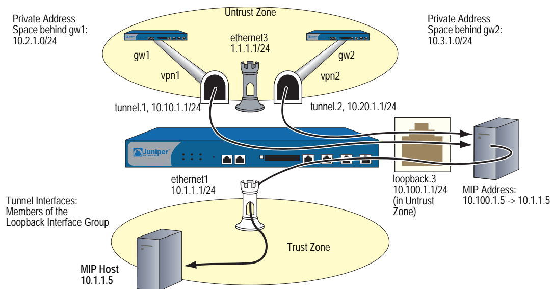
Figure 36: MIP for Two Tunnel Interfaces
