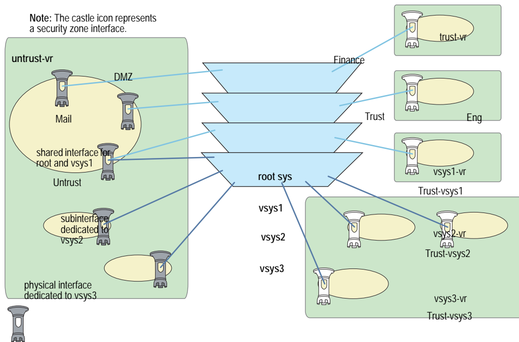
Figure 9: Vsys Architecture
