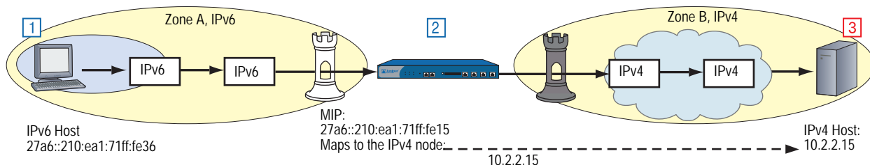
Figure 19: MIP from IPv6 to IPv4
