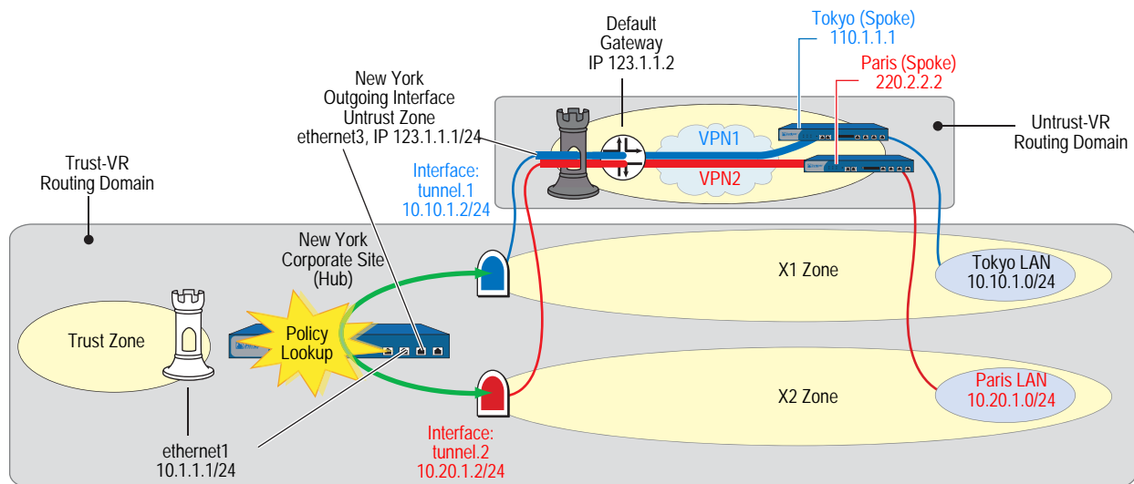
Figure 84: Back-to-Back VPNs with Two Routing Domains and Multiple Security Zones
