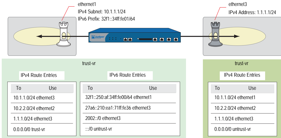
Figure 13: Dual-Stack Router Behavior
