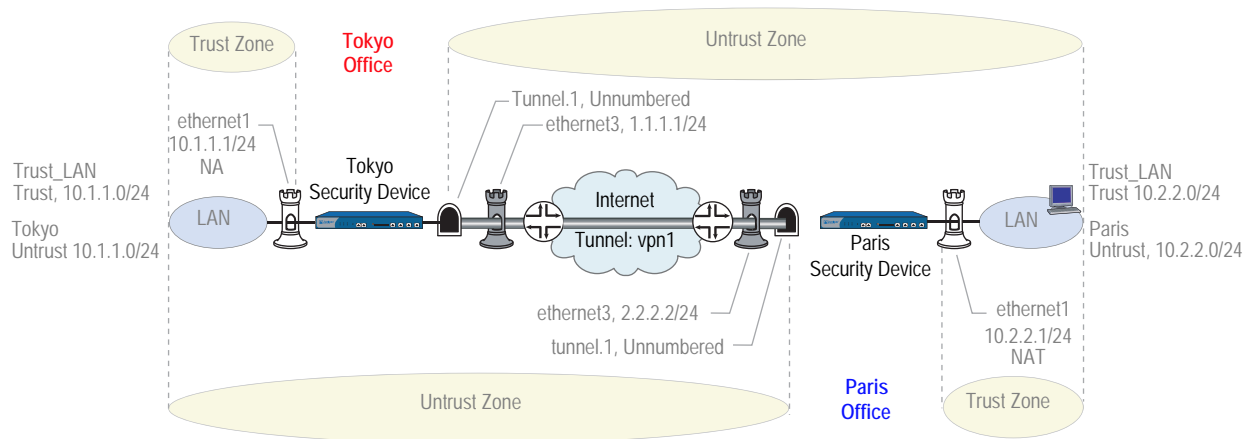
Figure 26: Site-to-Site Tunnel Configuration—VPN Tunnel
