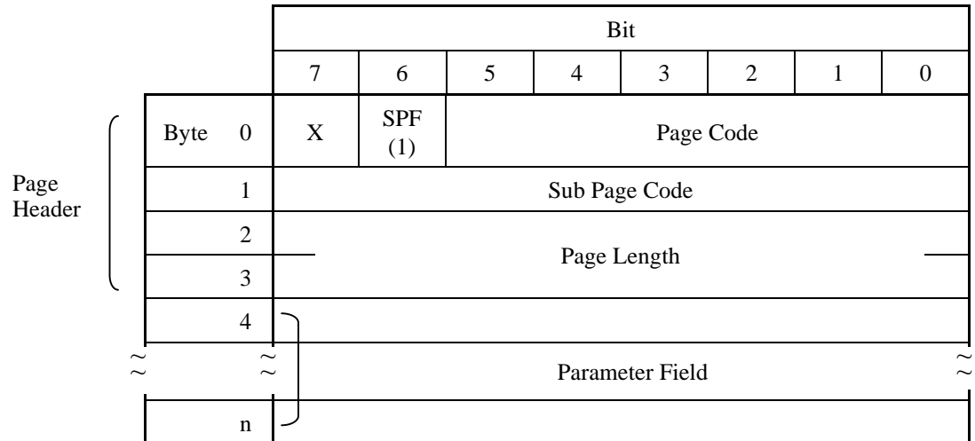
Figure 3.11 MODE SENSE command (Group 0) parameter configuration (2 of 2)
