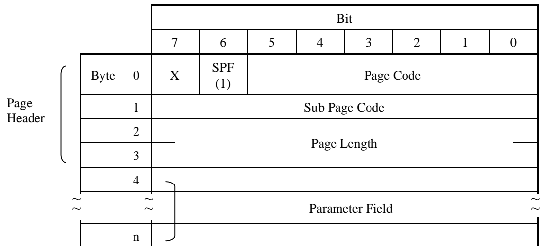
Figure 3.10 MODE SELECT EXTENDED command (Group 2) parameter configuration
