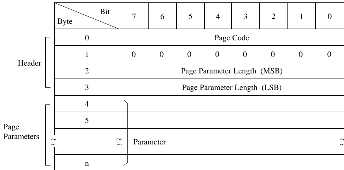
Figure 3.32 RECEIVE DIAGNOSTIC RESULTS command: Response data configuration
