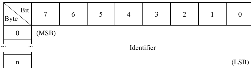
Figure 3.21 SET DEVICE IDENTIFER: parameter list
