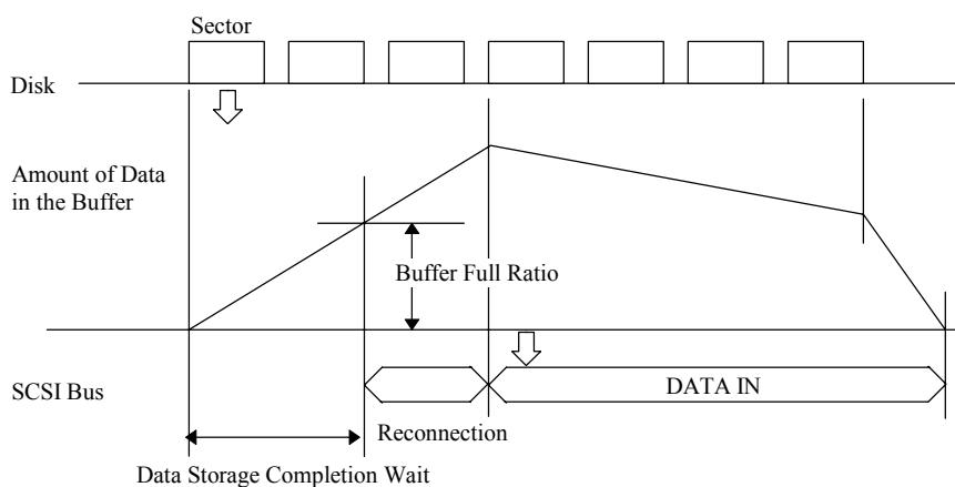
Figure 2.2 Example of data buffer operation during read
