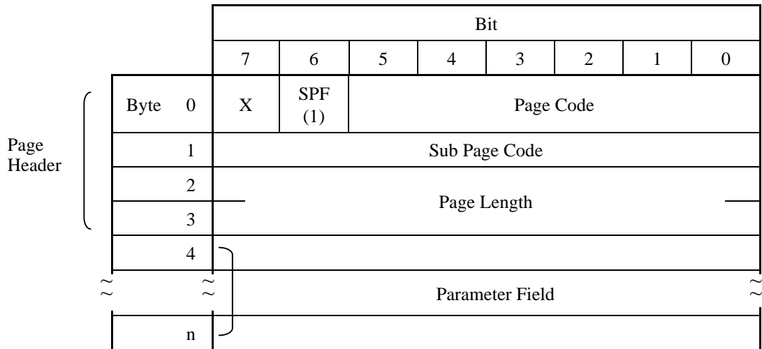
Figure 3.12 MODE SENSE EXTENDED command (Group 2) parameter configuration (2 of 2)
