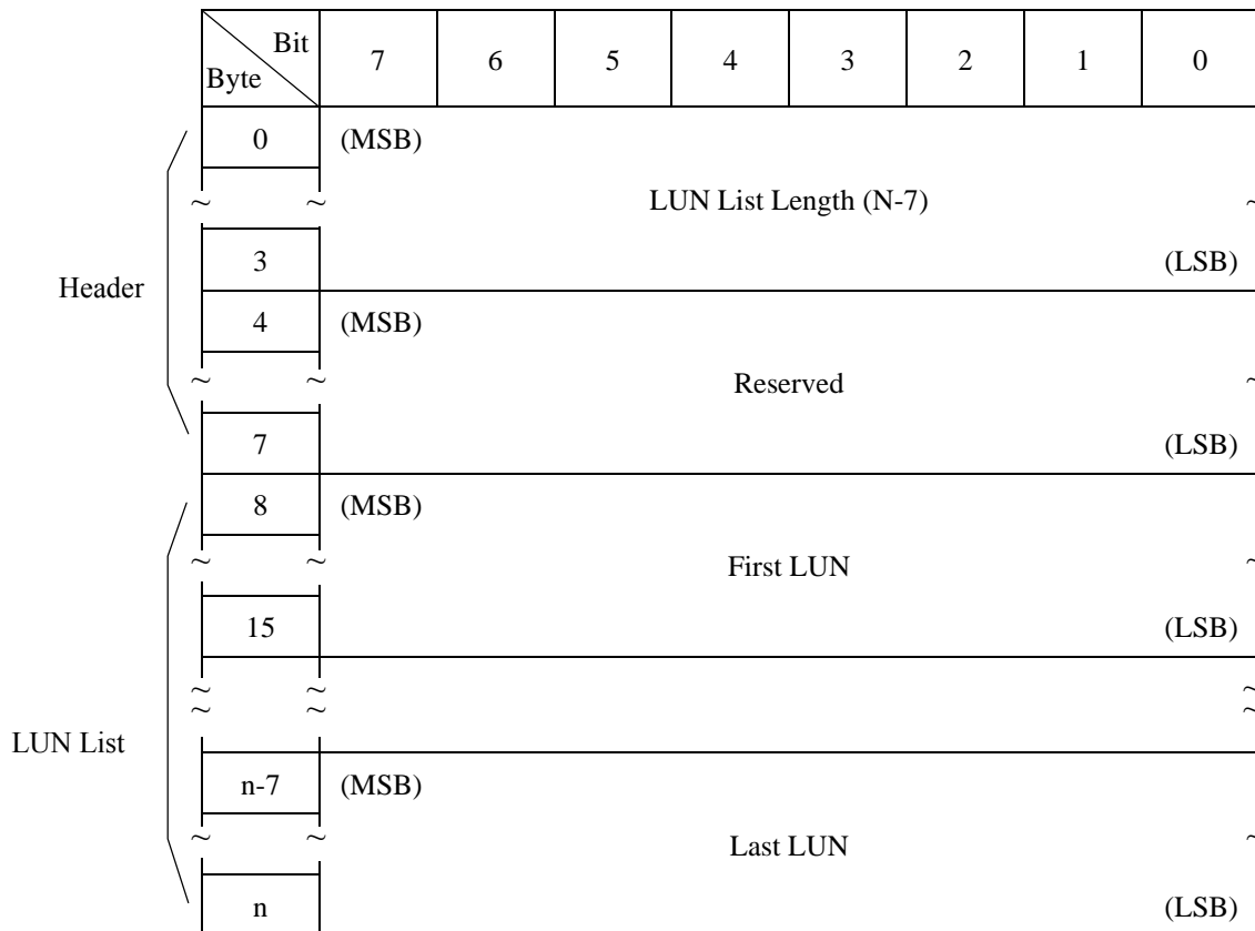
Figure 3.19 REPORT LUNS command: parameter list
