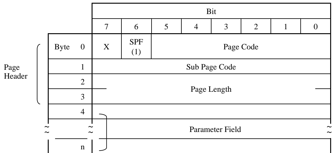
Figure 3.9 MODE SELECT command (Group 0) parameter configuration
