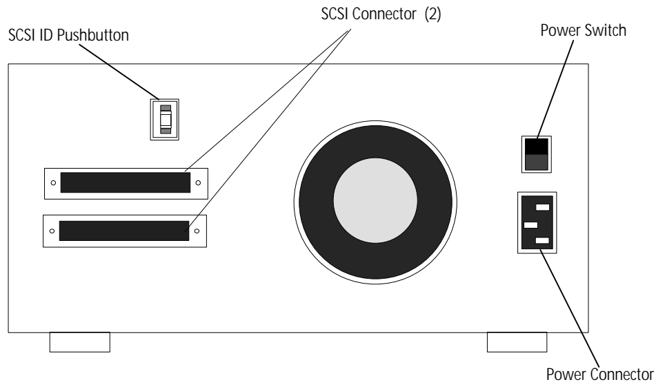
Figure 2-6 Tabletop Back Panel
