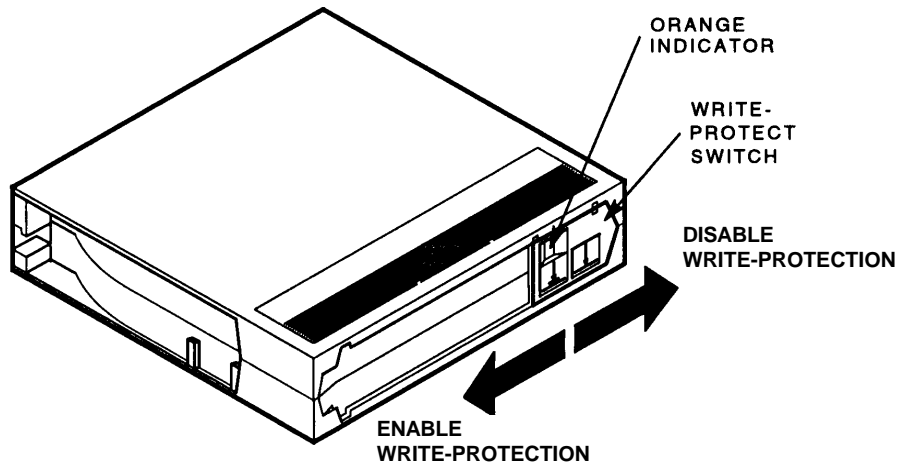
Figure D-5 Write-Protect Switch on Tape Cartridge
