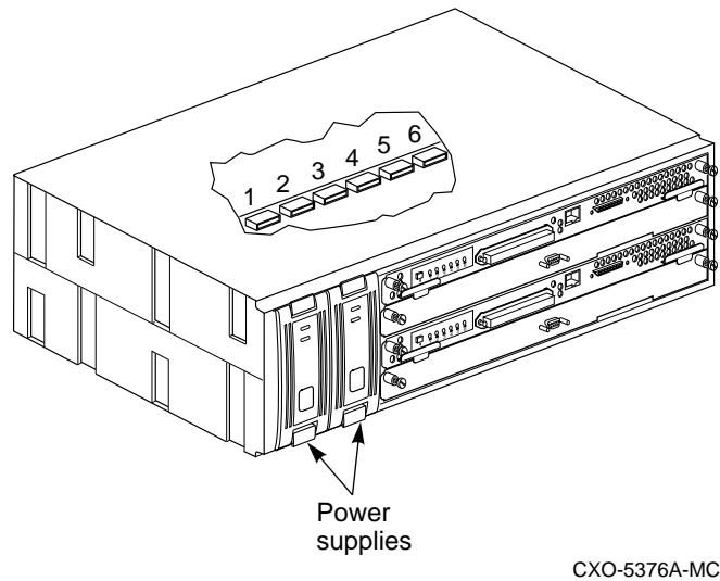
Figure 4-3 Controller Shelf with I/O Connectors
