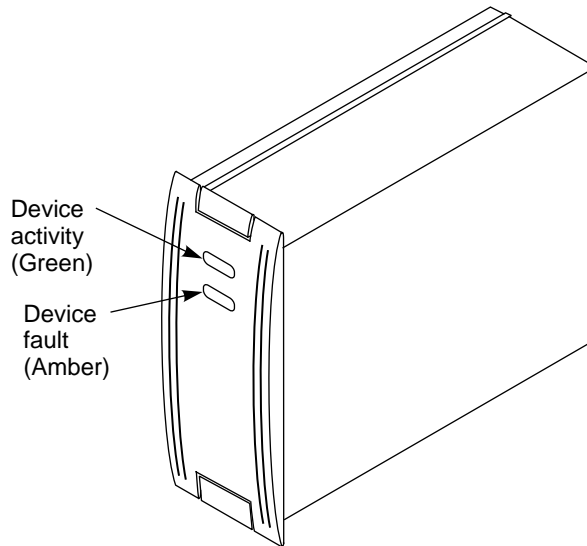
Figure 2-5 4.3 GB Disk Drive SBB
