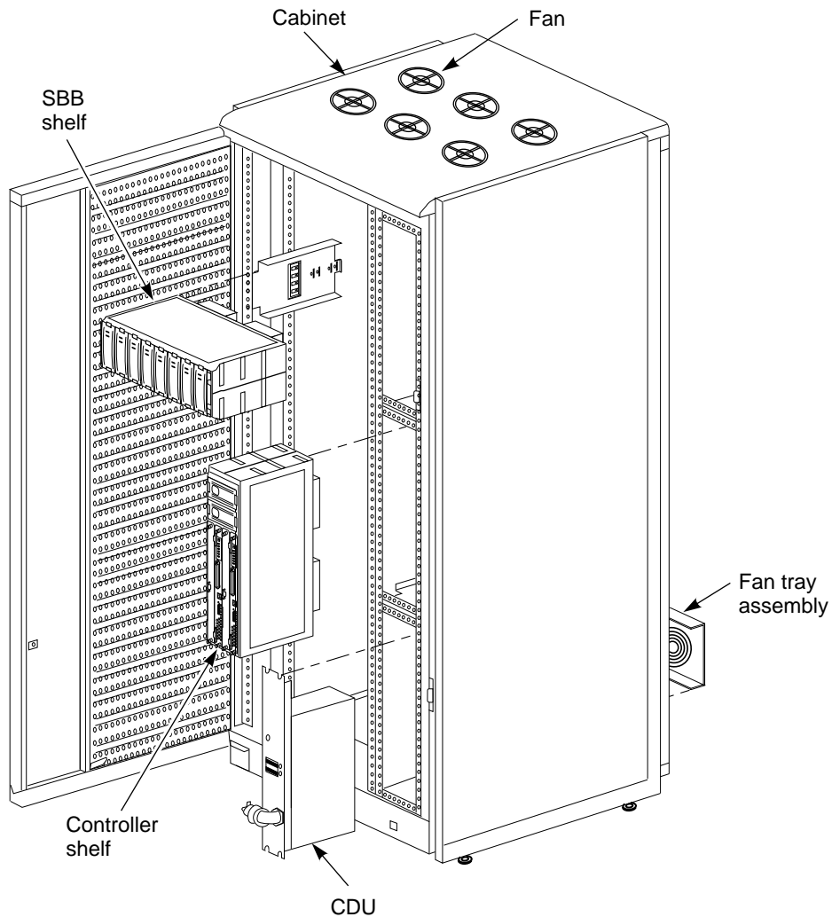
Figure 1-1 ESA Major Components
