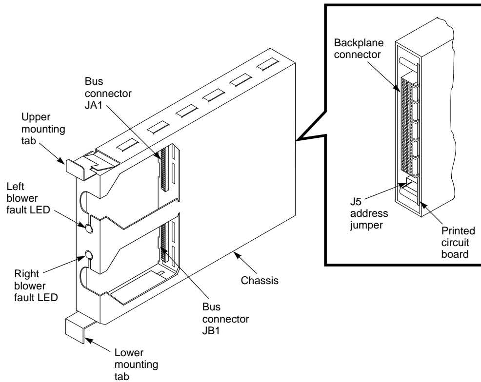
Figure 2-7 I/O Module Features
