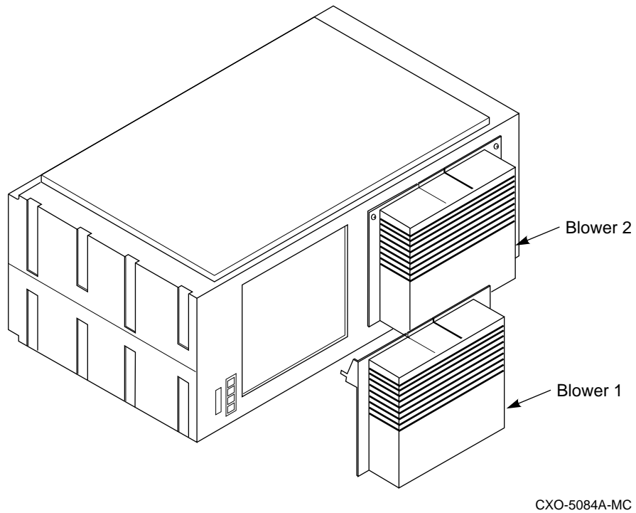
Figure 2-3 Blower Assembly
