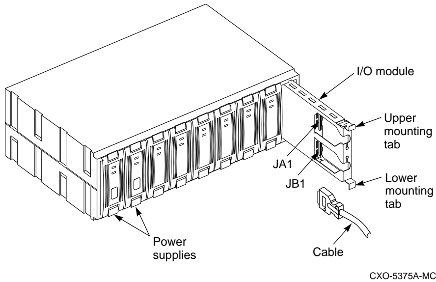
Figure 4-3 Controller Shelf with I/O Connectors
