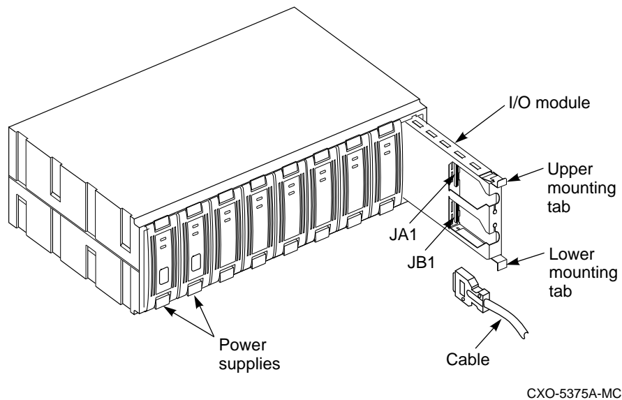
Figure 2-2 SBB Shelf with I/O Module
