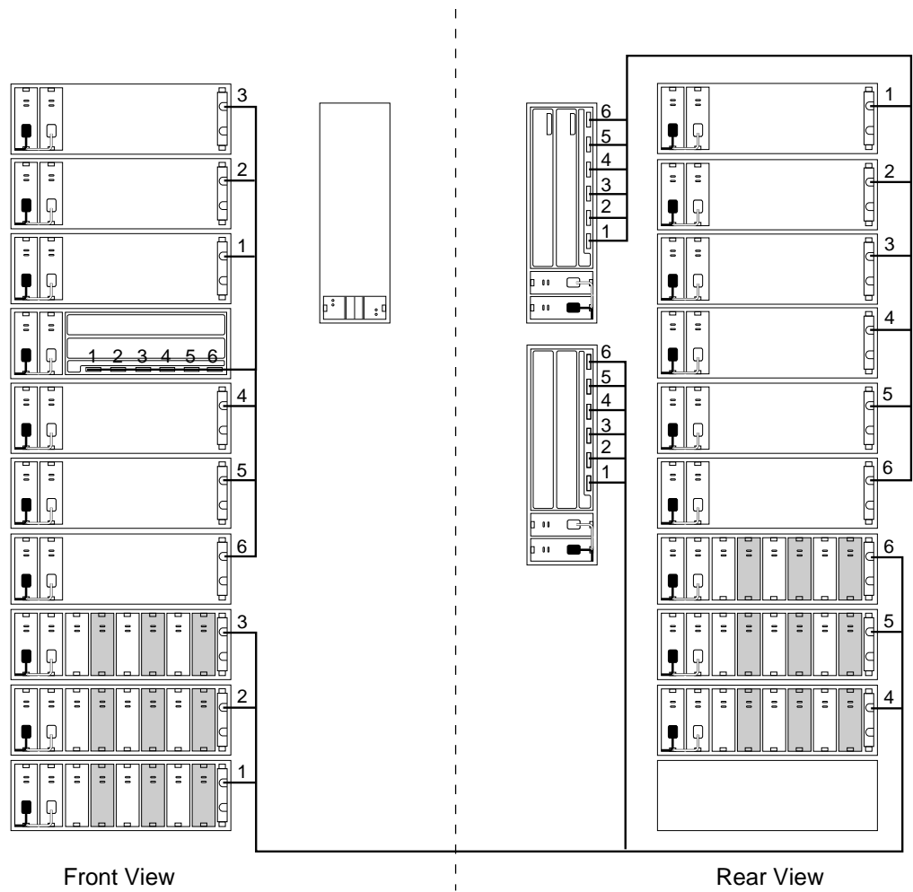
Figure 4-4 Model ESxxx-C4 (Part # SW8T1)
