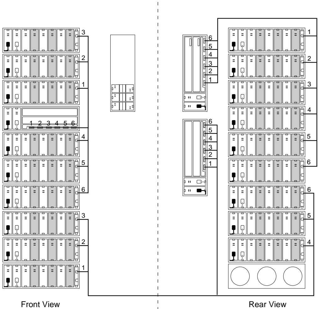
Figure 4-5 Model ESxxx-C4 (Part # SW8T2, 3, and 4 )
