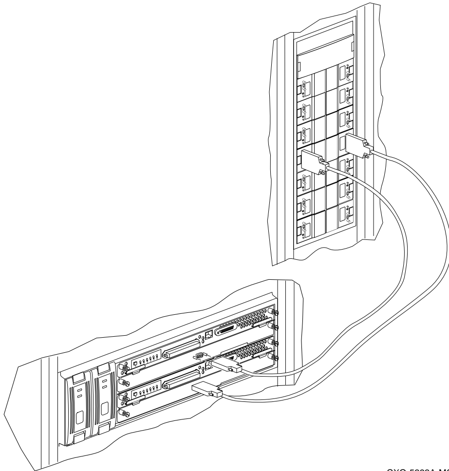
Figure 2-9 Cache to ECB Connection
