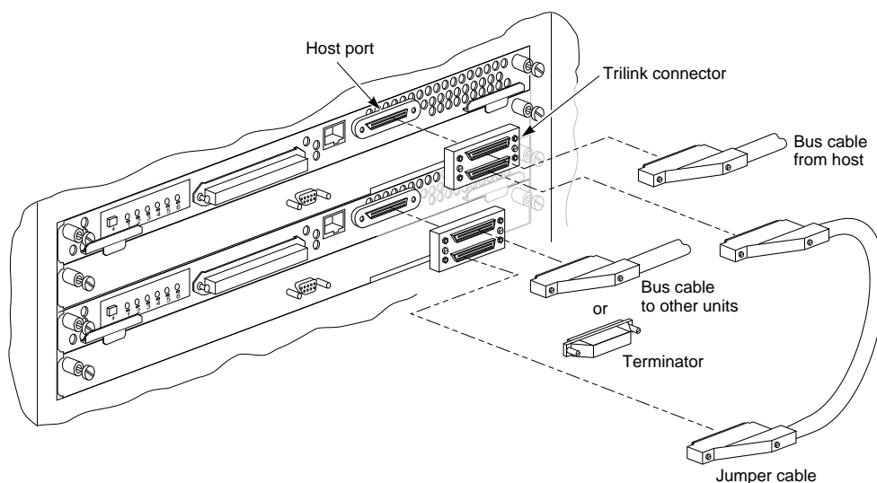
Figure 3-1 Horizontal Mounted Controllers with Cache and Trilink Connectors
