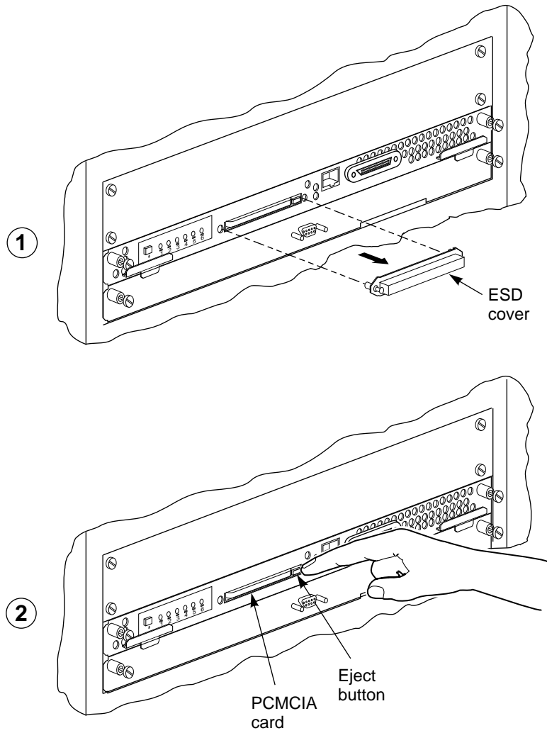
Figure 3-3 Location of Program Card ESD Cover
