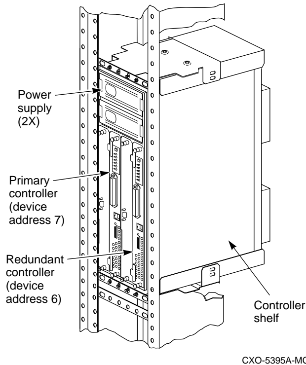
Figure 3-2 Vertical Mounted Controllers with Cache
