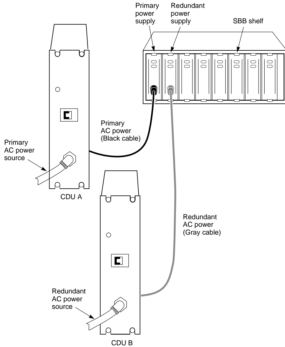
Figure 4-1 Dual CDU Power Configuration
