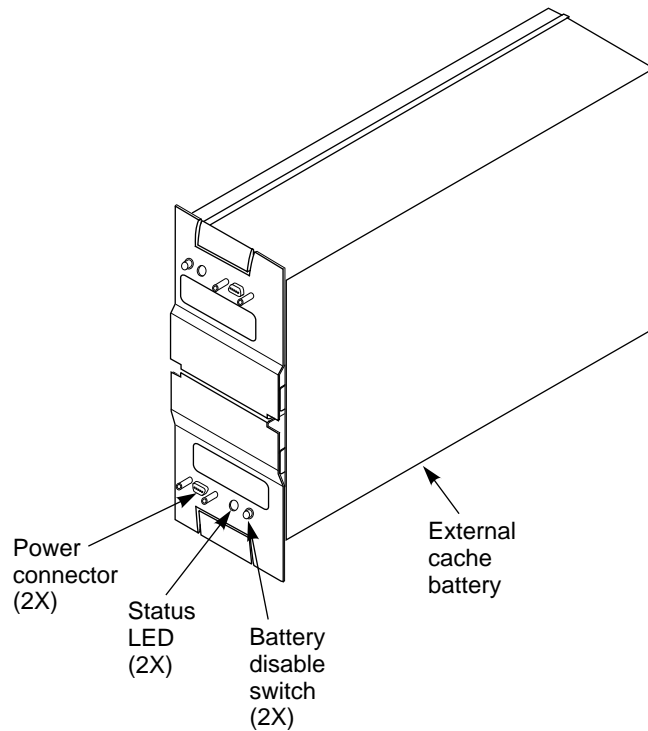
Figure 2-10 ECB SBB
