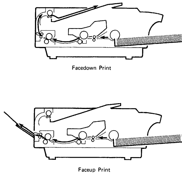
Figure 1-6: 2100 Paper Paths
