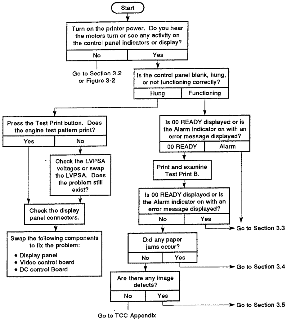
Figure 3-1: Start FIP
