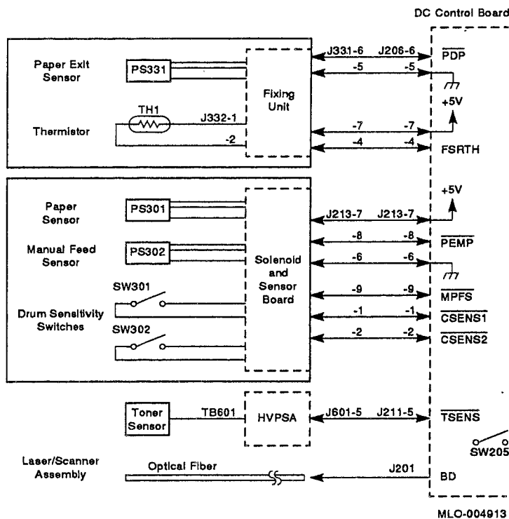
Figure 1-9: 2100 DC Control Board Input Signals
