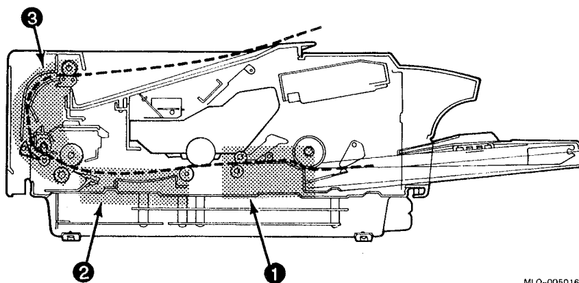
Figure 3-4: 2100 Jam Areas
