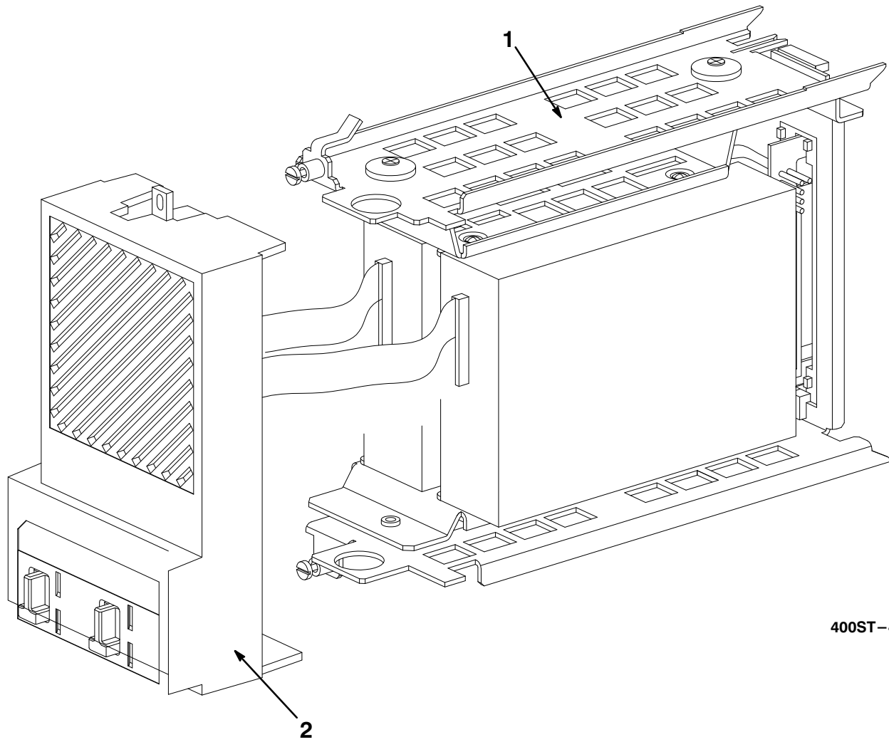
Figure 42. Storage Element, RZ262 Dual
