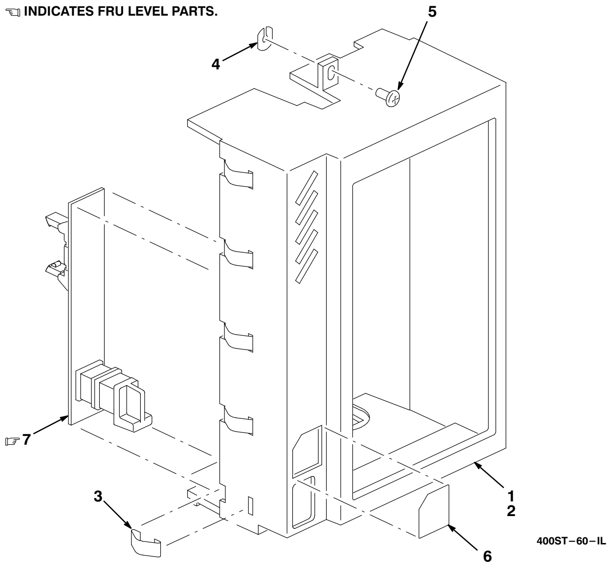
Figure 60. Bezel Assembly, Tape Drive
