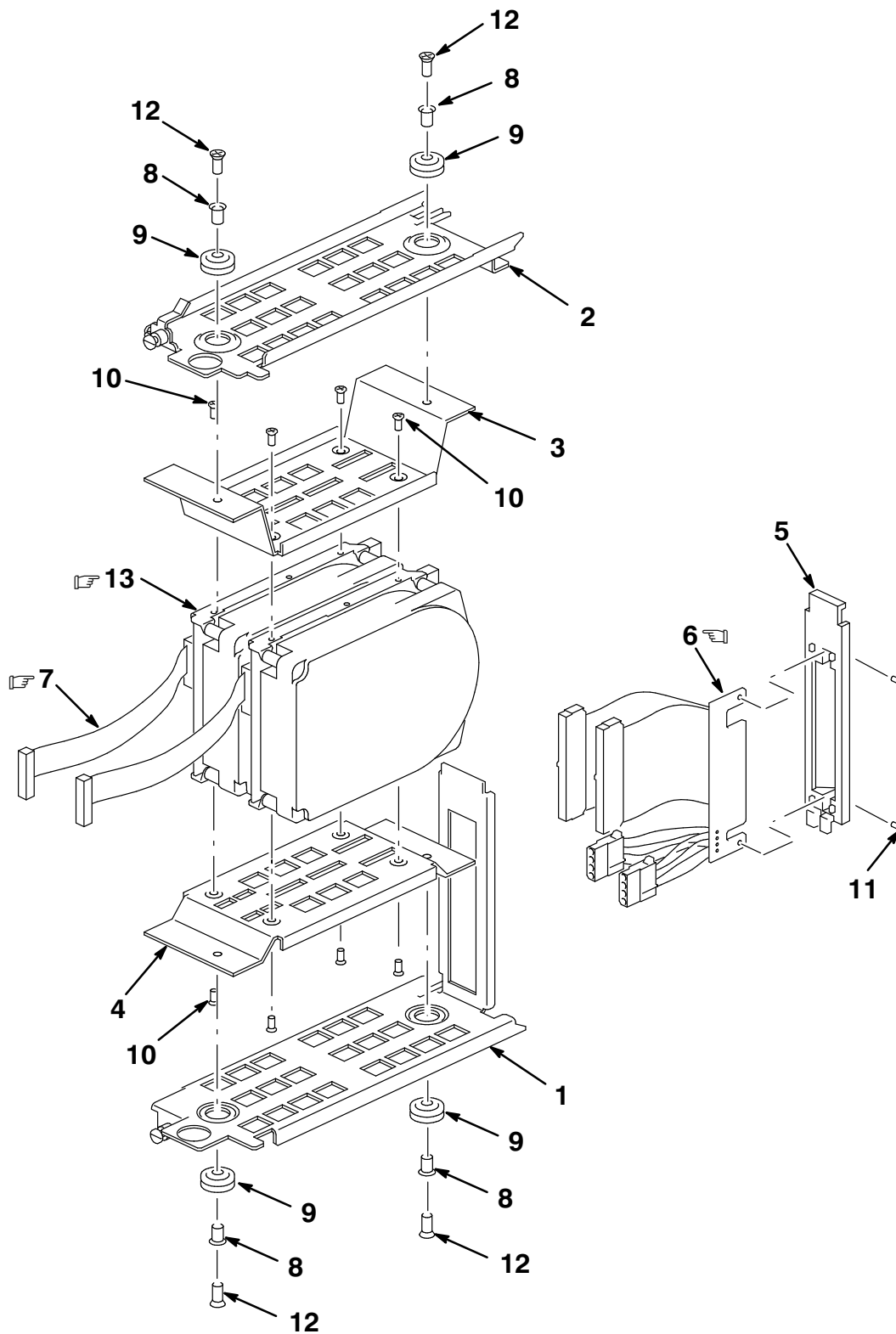
Figure 40. Drive Assembly, BA400 SCSI
