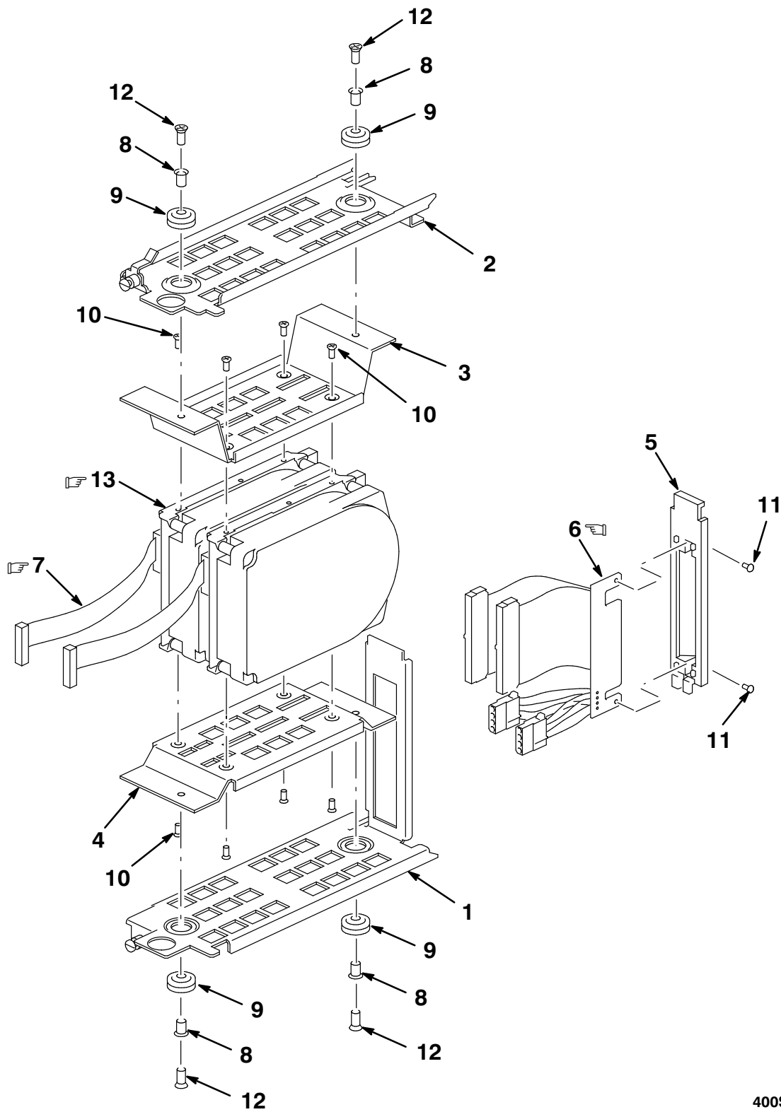
Figure 43. Drive Assembly, BA400 SCSI
