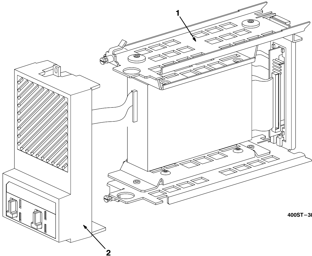
Figure 38. Storage Element, RZ28E
