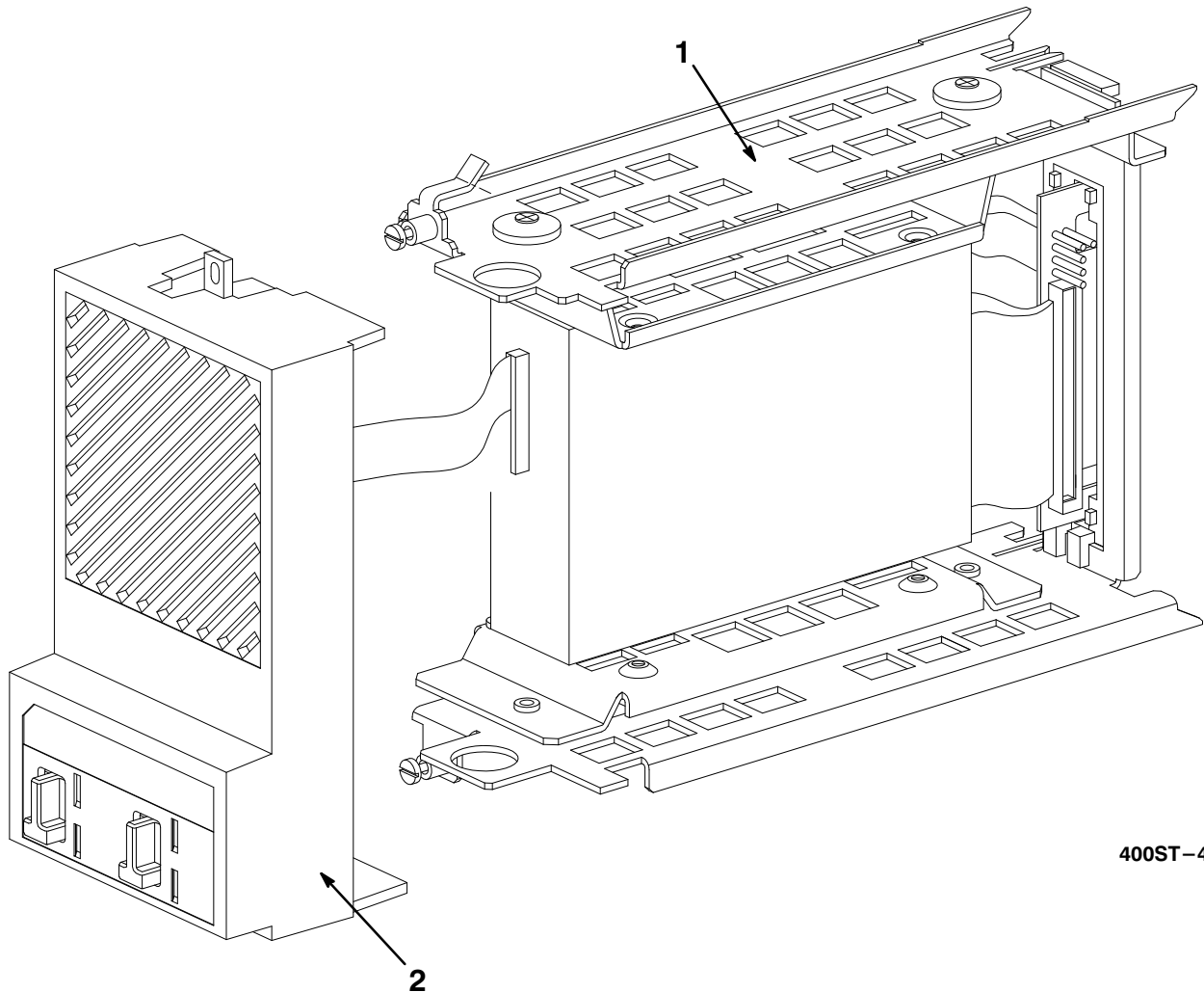
Figure 41. Storage Element, RZ26L
