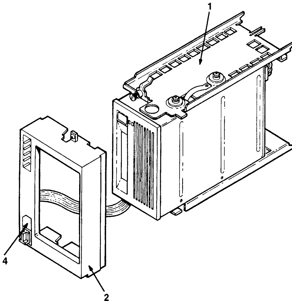
Figure 46. Storage Element, TLZ04
