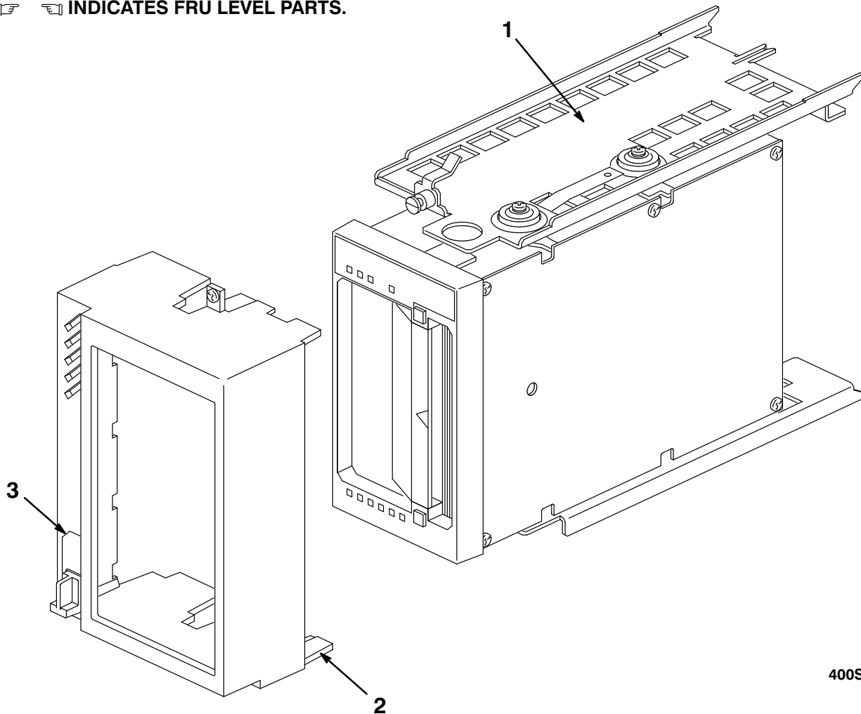
Figure 53. Storage Element, TZ87
