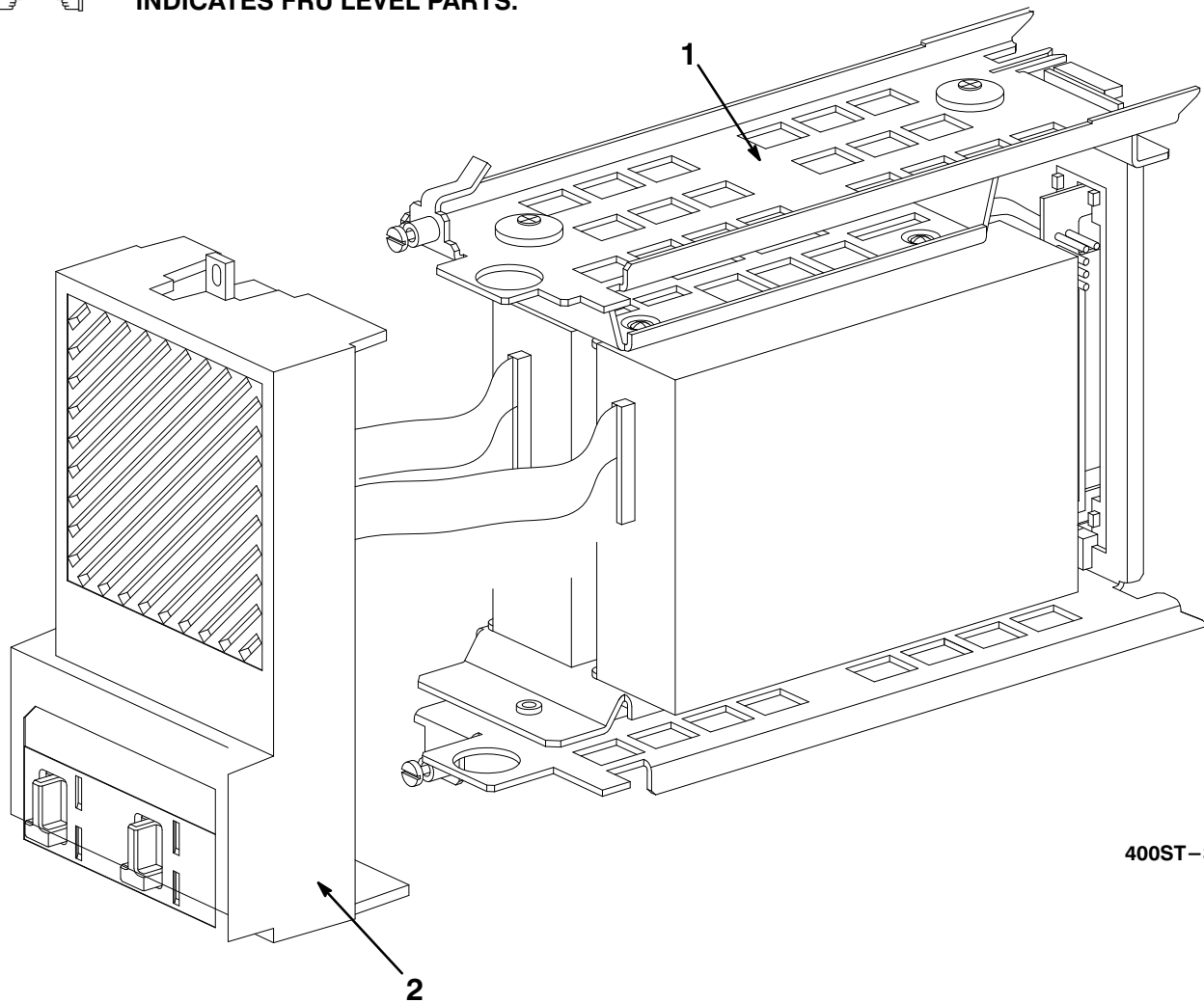
Figure 39. Storage Element, RZ282 Dual
