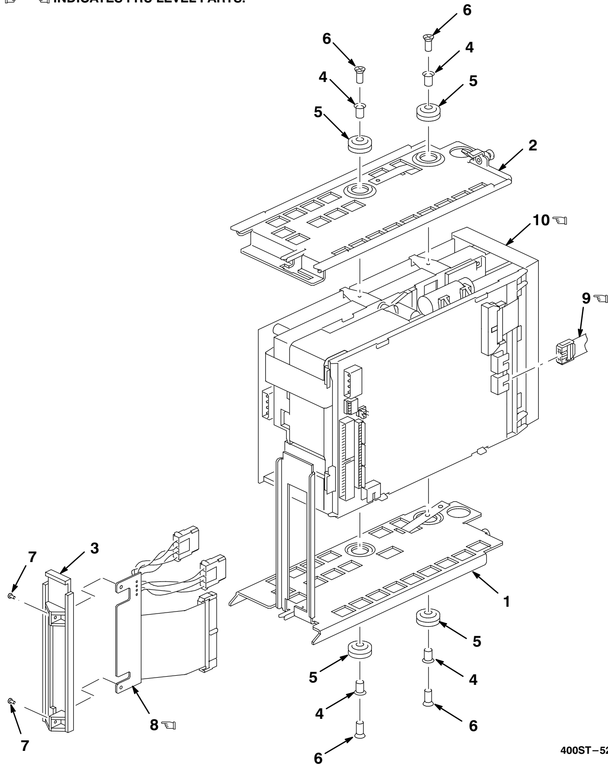
Figure 52. Mounting Assembly, TZ86
