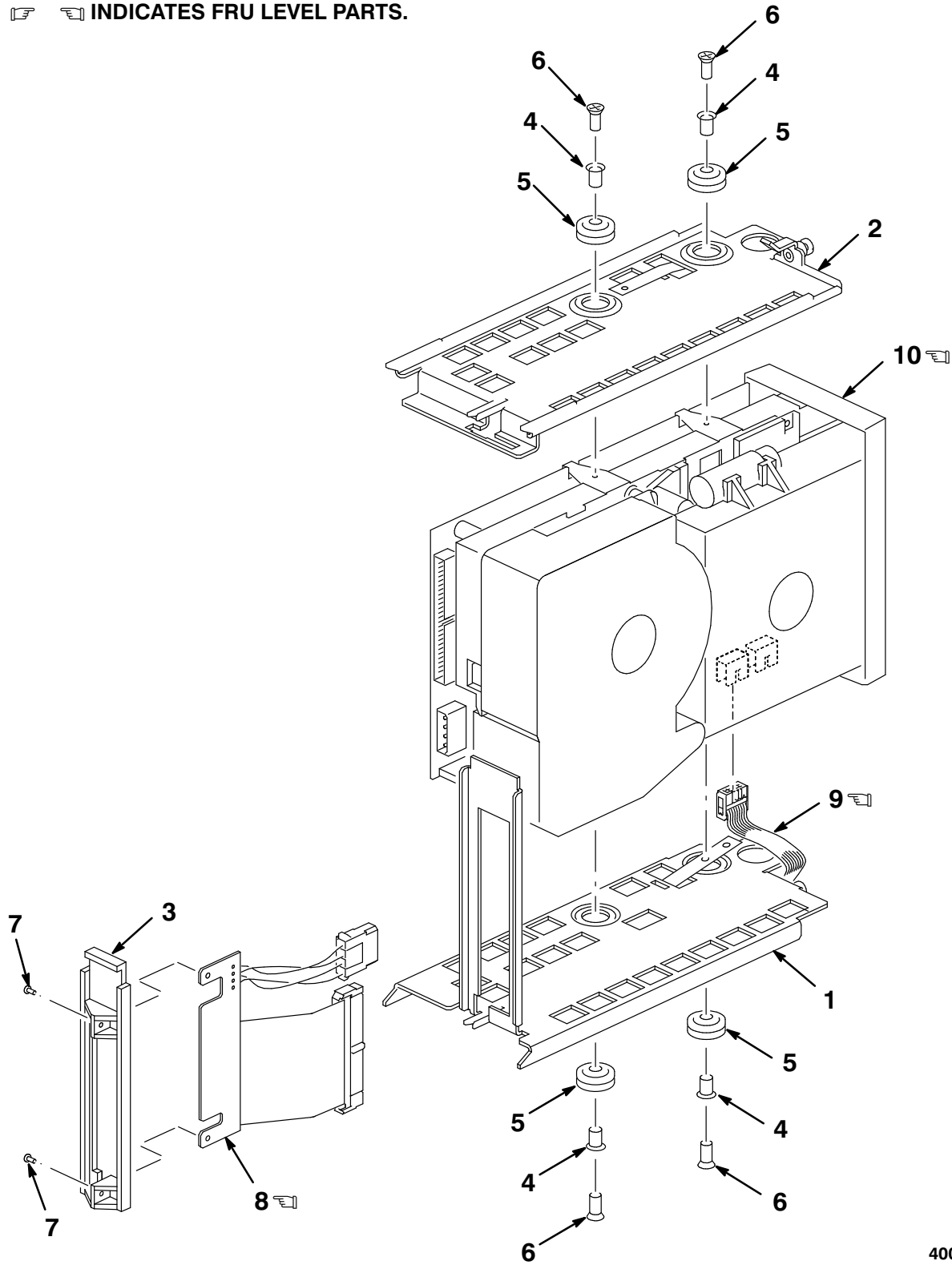
Figure 54. Mounting Assembly, TZ87
