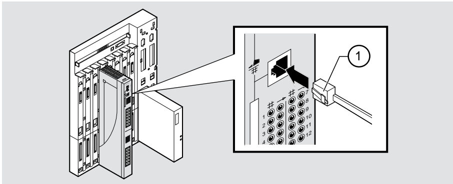
Figure 2-6: LDM Port Cable Connection
