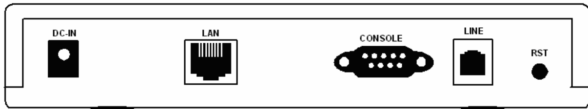
Rear Panel of SHDSL.bis 2-wire/1-port router/bridge
